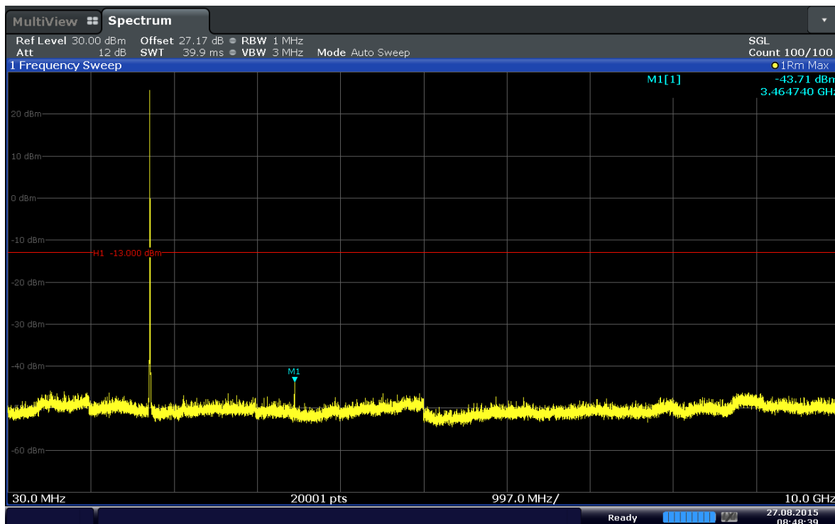
Plot 6-37. Conducted Spurious Plot (Band 4–5MHz–QPSK–RB Size 1–RB Offset 12–Ch.20175)
