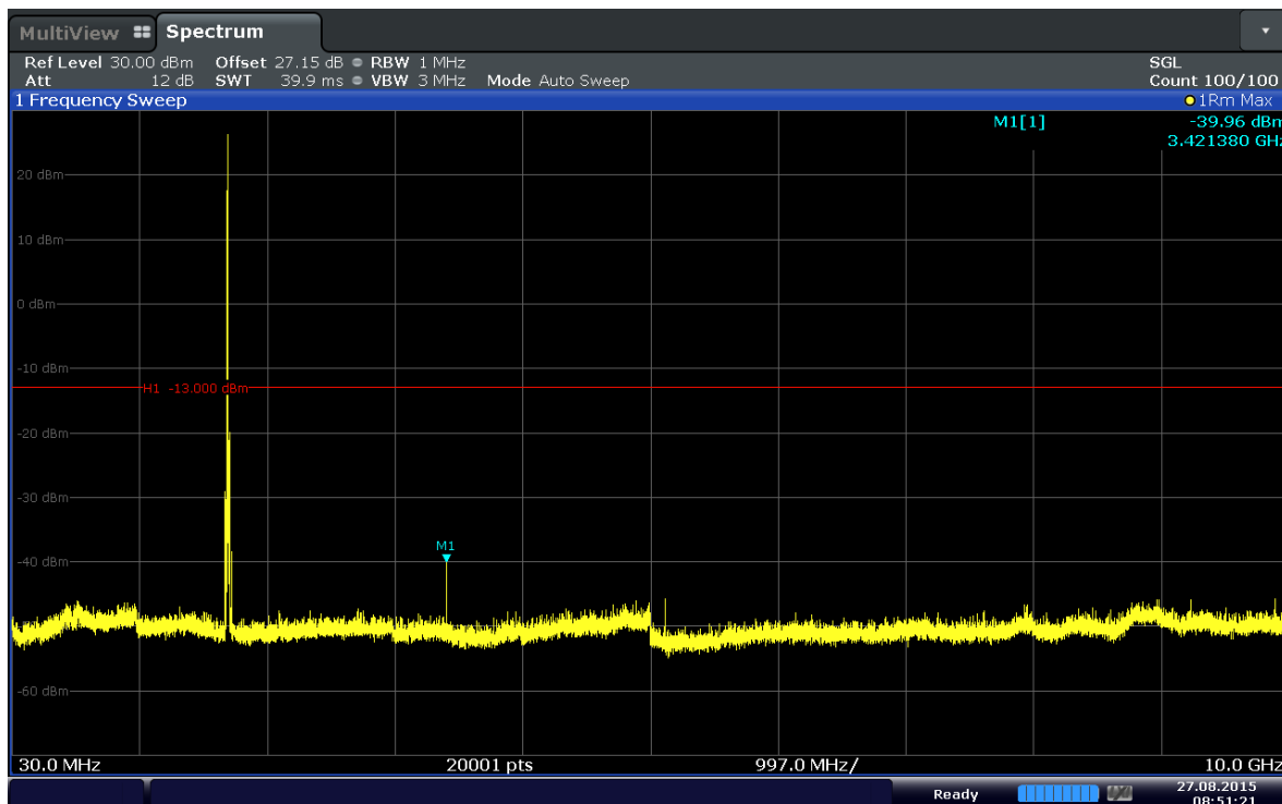
Plot 6-41. Conducted Spurious Plot (Band 4–10MHz–QPSK–RB Size 1–RB Offset 0–Ch.20000)
