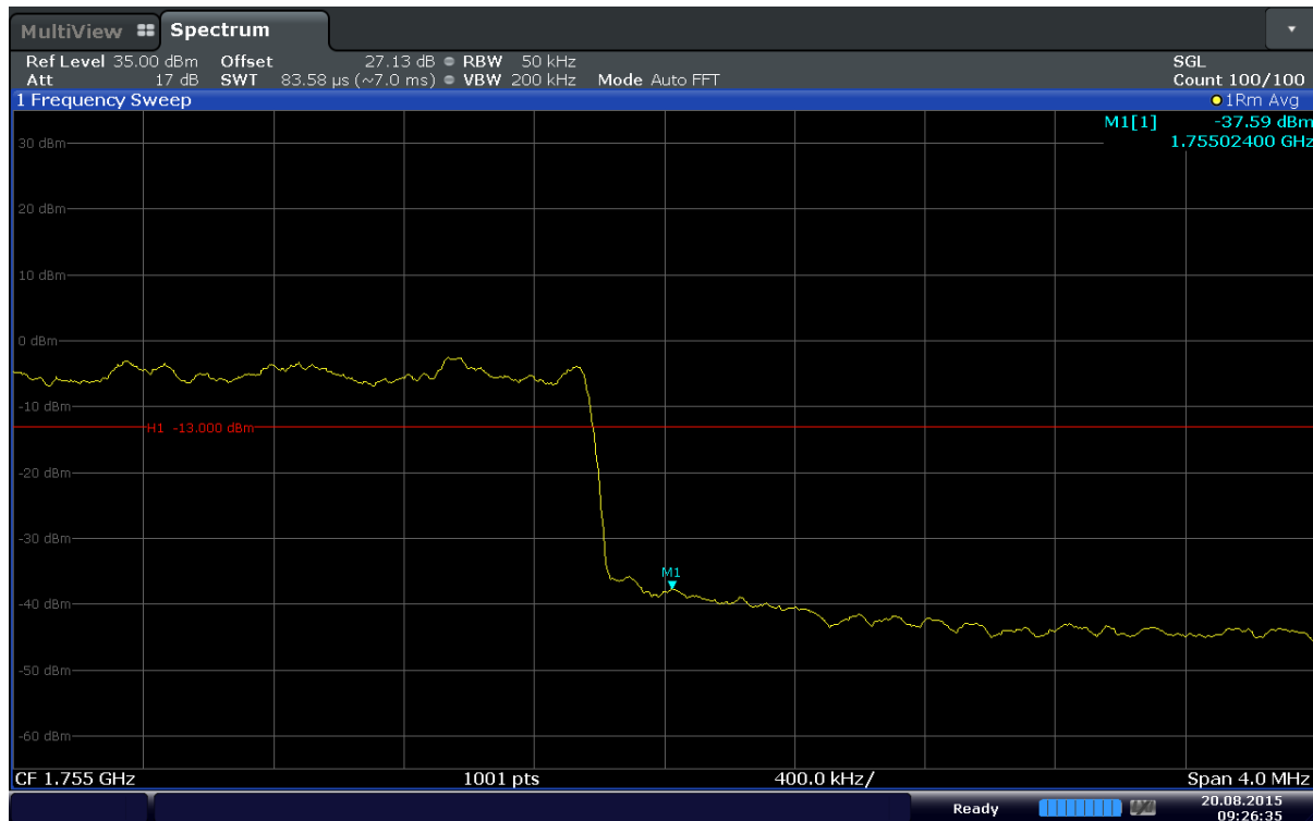
Plot 6-75. Upper Band Edge Plot (Band 4 – 5MHz – QPSK – RB Size 25)
