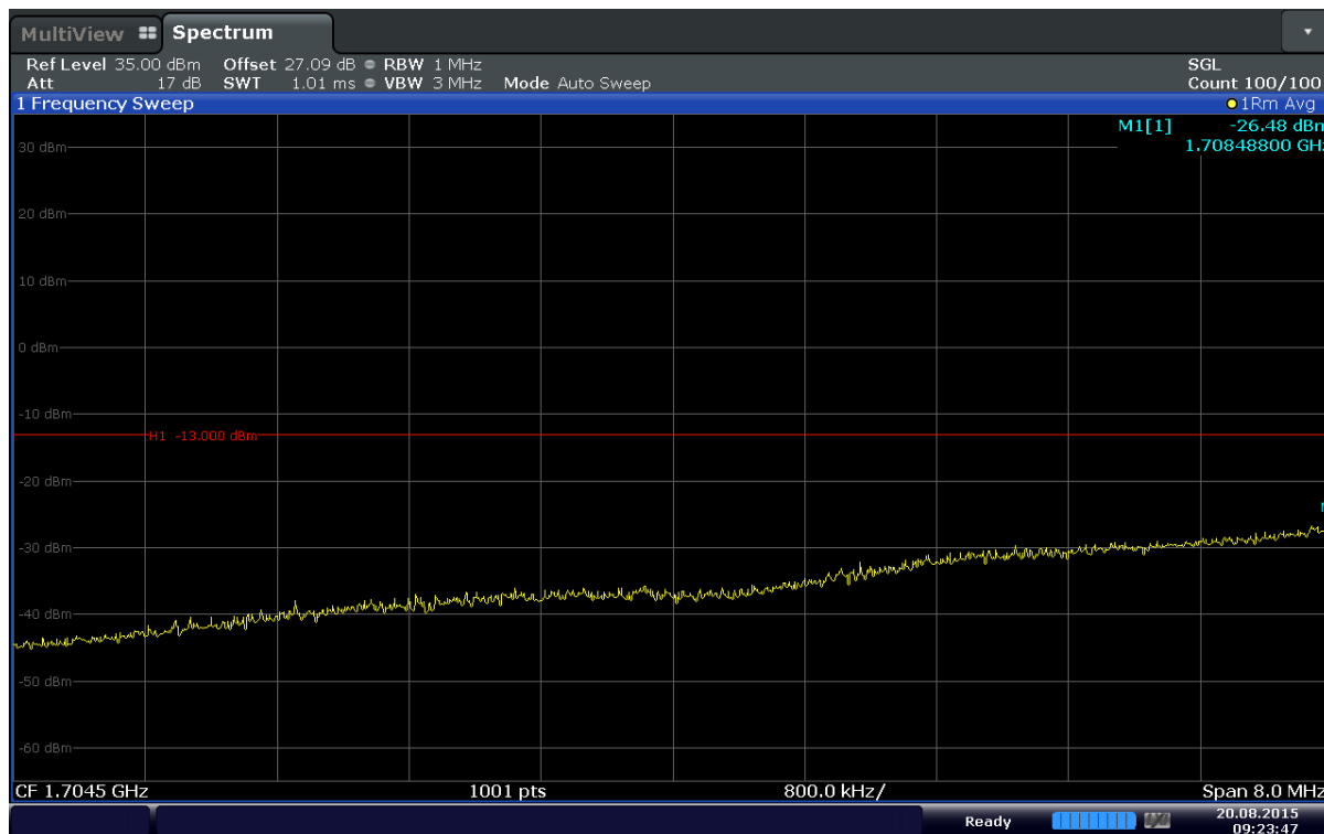
Plot 6-74. Extended Lower Band Edge Plot (Band 4 – 5MHz – QPSK – RB Size 25)
