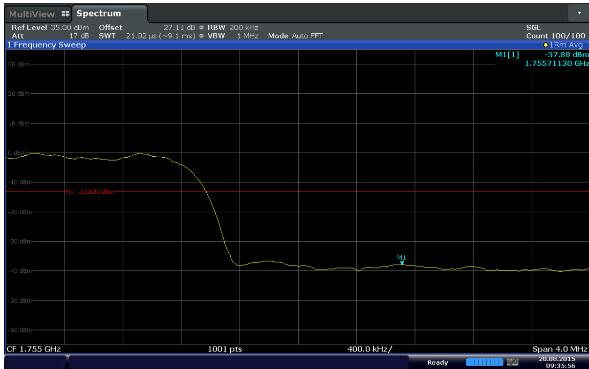
Plot 6-83. Upper Band Edge Plot (Band 4 – 15MHz – QPSK – RB Size 75)
