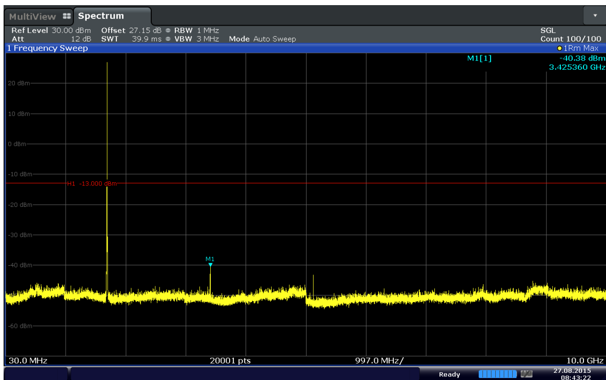
Plot 6-29. Conducted Spurious Plot (Band 4–3MHz–QPSK–RB Size 1–RB Offset 14–Ch.19965)
