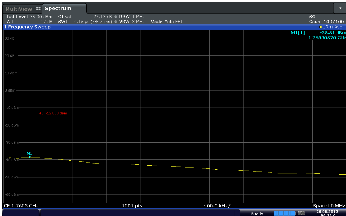
Plot 6-72. Extended Upper Band Edge Plot (Band 4 – 3MHz – QPSK – RB Size 15)
