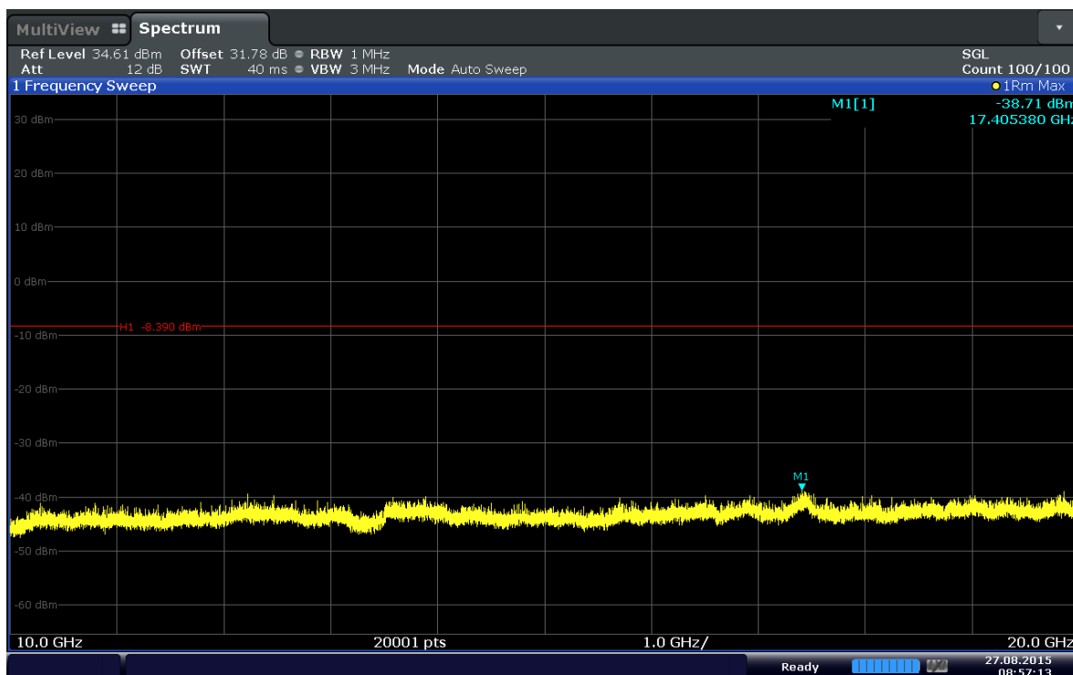
Plot 6-50. Conducted Spurious Plot (Band 4–15MHz–QPSK–RB Size 1–RB Offset 36–Ch.20175)
