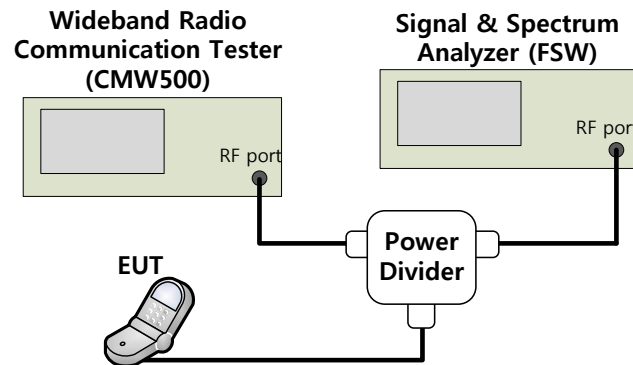
Figure 6-3. Test Instruments & Measurement Setup
