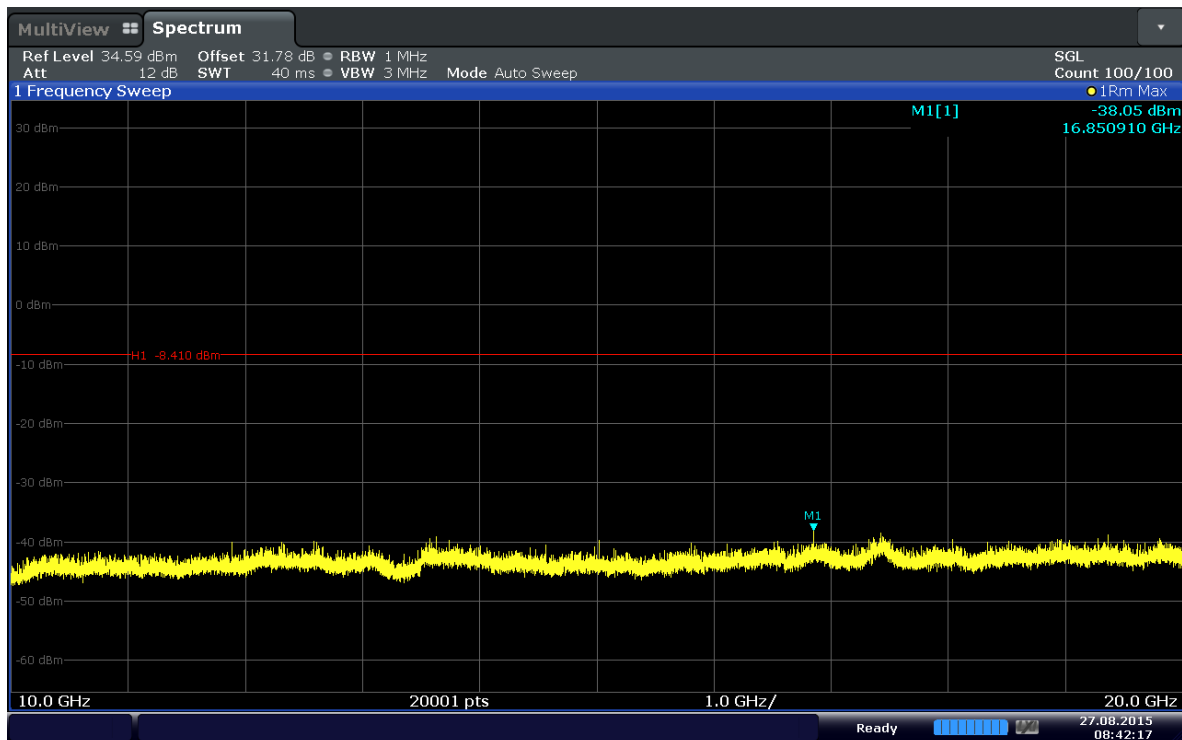
Plot 6-28. Conducted Spurious Plot (Band 4–1.4MHz–QPSK–RB Size 1–RB Offset 2–Ch.20393)
