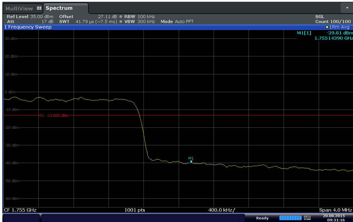
Plot 6-79. Upper Band Edge Plot (Band 4 – 10MHz – QPSK – RB Size 50)
