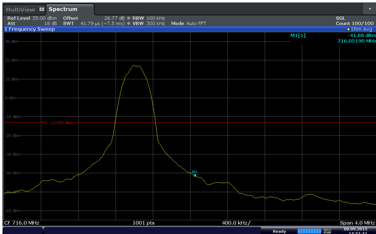
Plot 6-64. Upper Band Edge Plot (Band 17 – 10MHz – QPSK – RB Size 1 – RB Offset 49)
