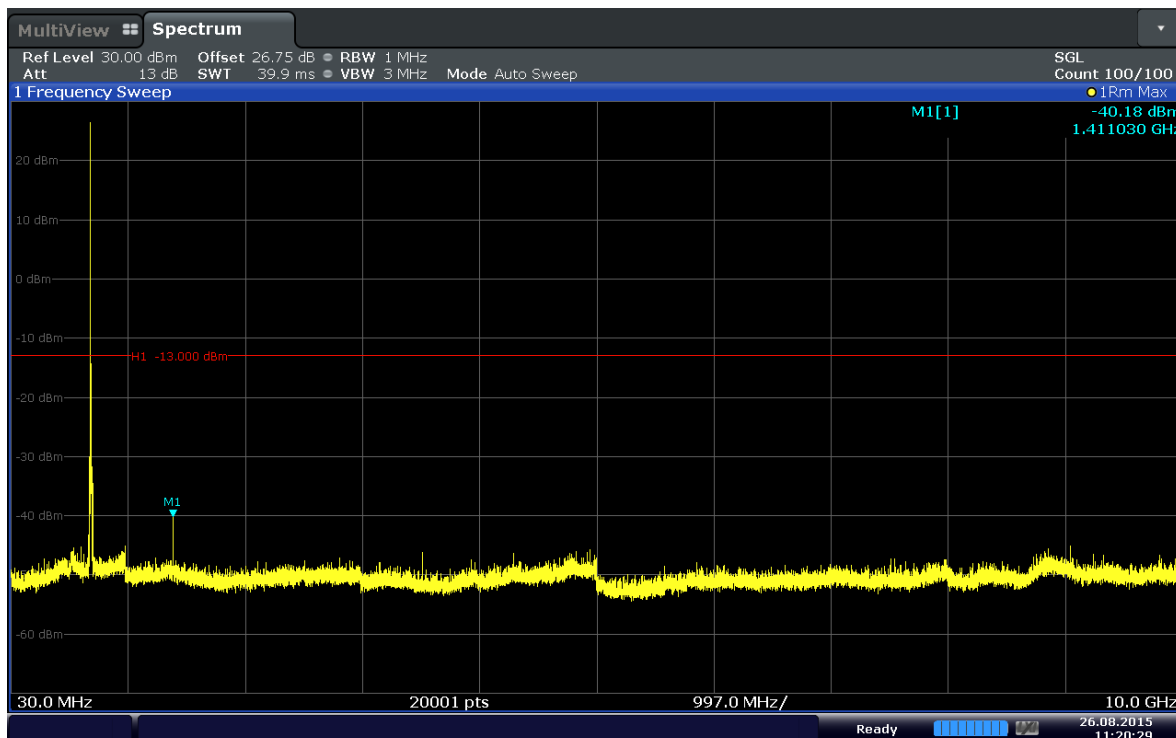
Plot 6-21. Conducted Spurious Plot (Band 17–10MHz–QPSK–RB Size 1–RB Offset 0–Ch.23790)
