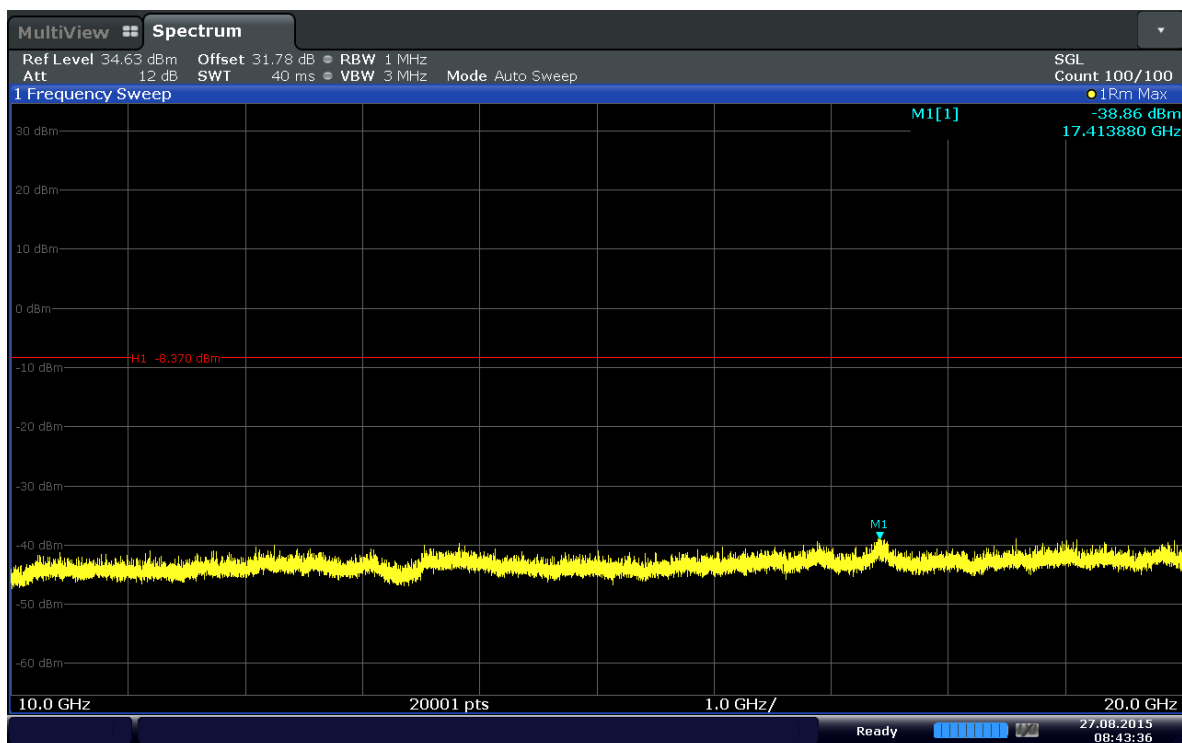
Plot 6-30. Conducted Spurious Plot (Band 4–3MHz–QPSK–RB Size 1–RB Offset 14–Ch.19965)
