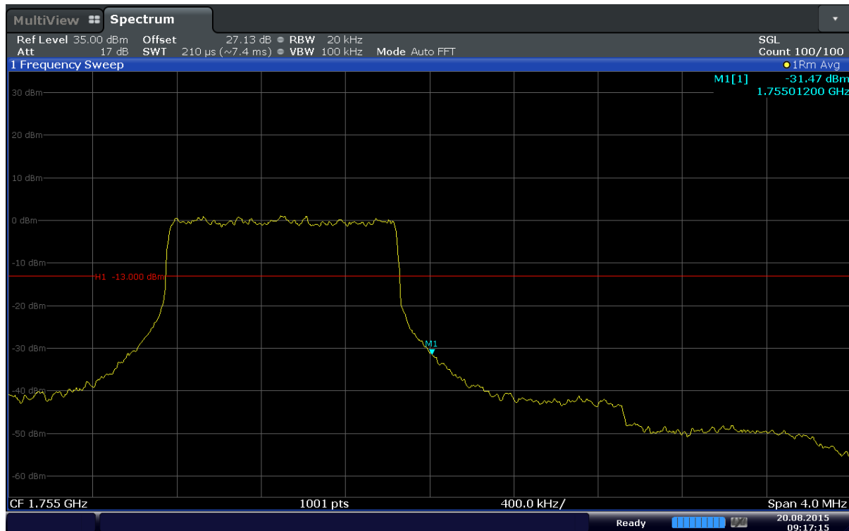
Plot 6-67. Upper Band Edge Plot (Band 4 – 1.4MHz – QPSK – RB Size 6)
