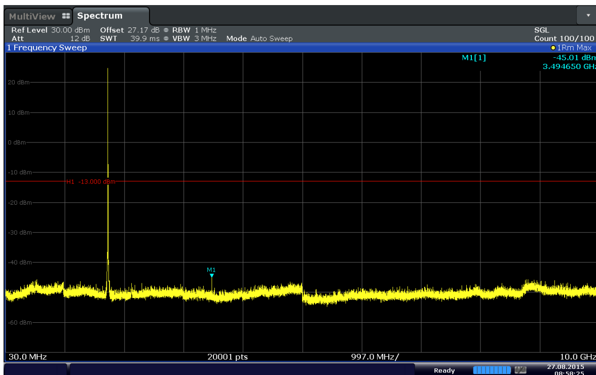
Plot 6-51. Conducted Spurious Plot (Band 4–15MHz–QPSK–RB Size 1–RB Offset 36–Ch.20325)
