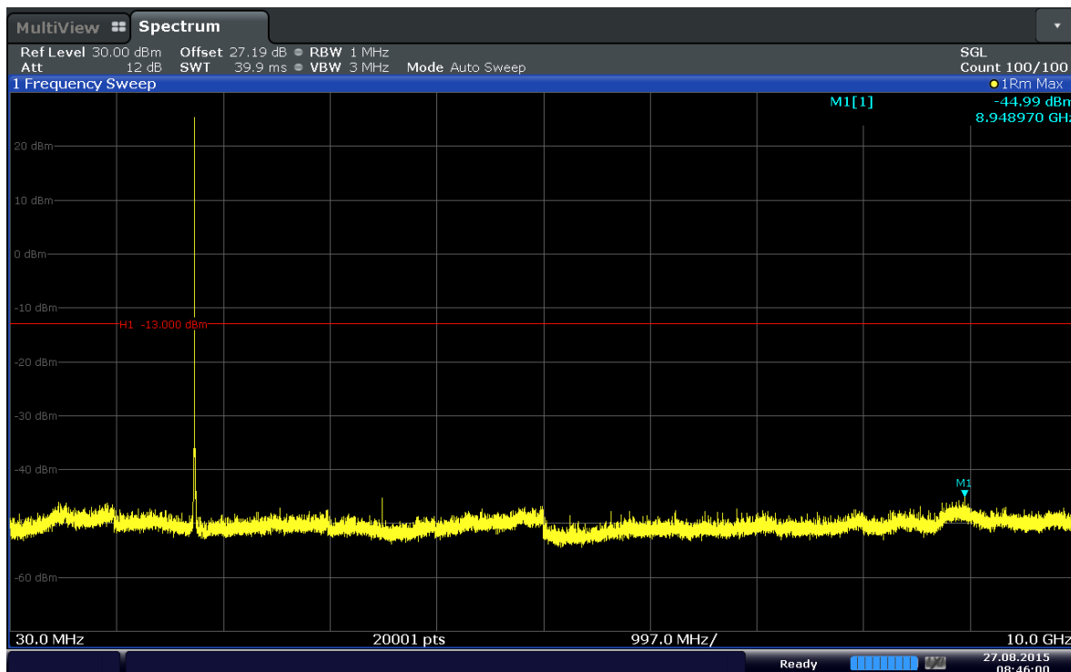
Plot 6-33. Conducted Spurious Plot (Band 4-3MHz-QPSK-RB Size 1-RB Offset 7-Ch.20385)
