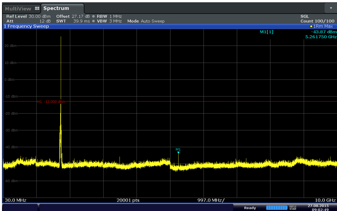
Plot 6-57. Conducted Spurious Plot (Band 4–20MHz–QPSK–RB Size 1–RB Offset 99–Ch.20300)
