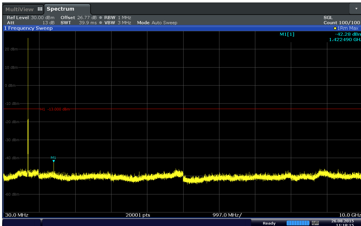
Plot 6-19. Conducted Spurious Plot (Band 17–5MHz–QPSK–RB Size 1–RB Offset 0–Ch.23825)
