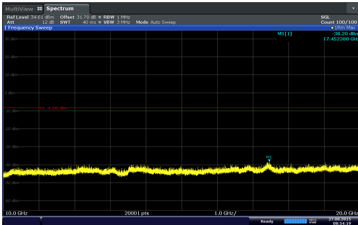
Plot 6-46. Conducted Spurious Plot (Band 4–10MHz–QPSK–RB Size 1–RB Offset 49–Ch.20350)
