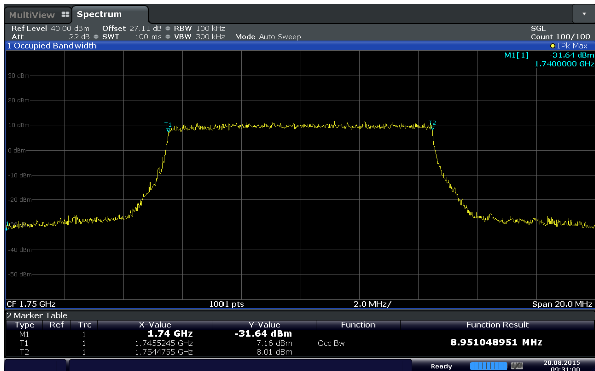
Plot 6-12. Occupied Bandwidth Plot (Band 4 – 10MHz 16QAM - RB Size 50)
