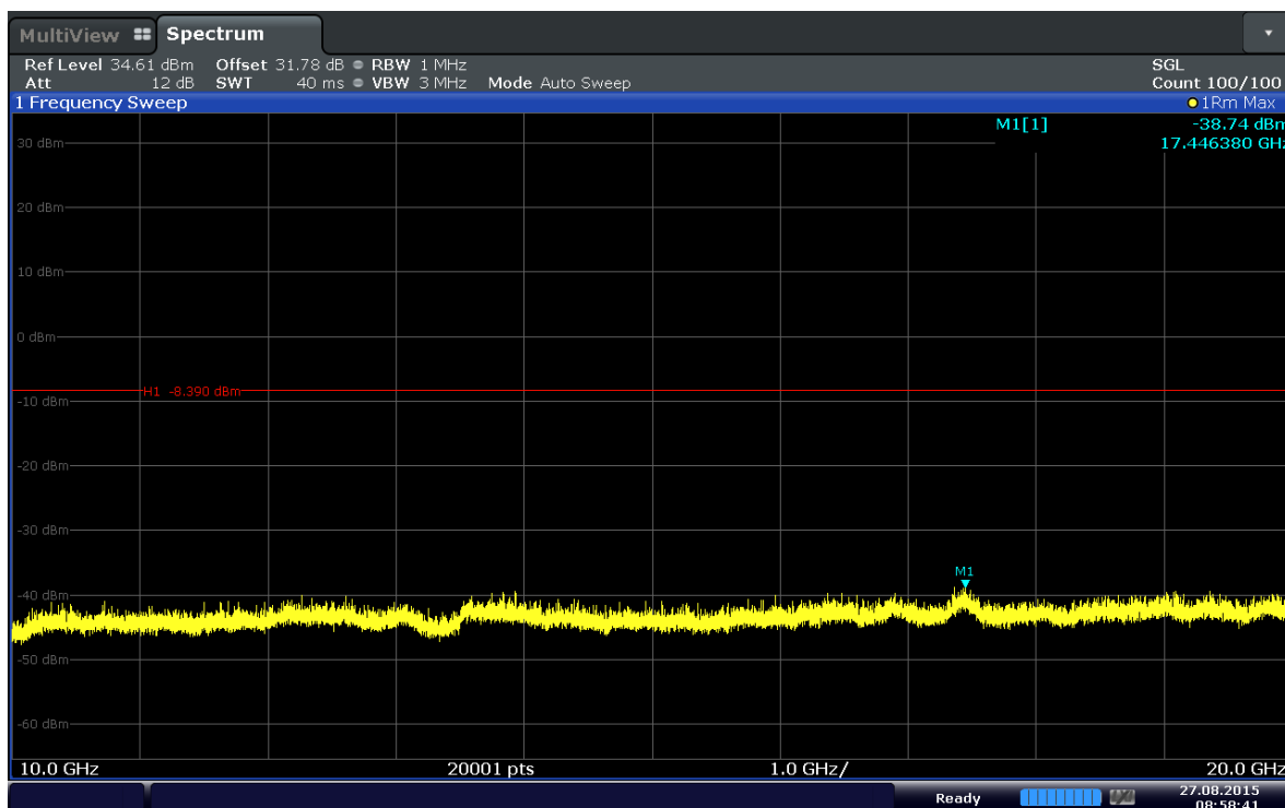
Plot 6-52. Conducted Spurious Plot (Band 4–15MHz–QPSK–RB Size 1–RB Offset 36–Ch.20325)
