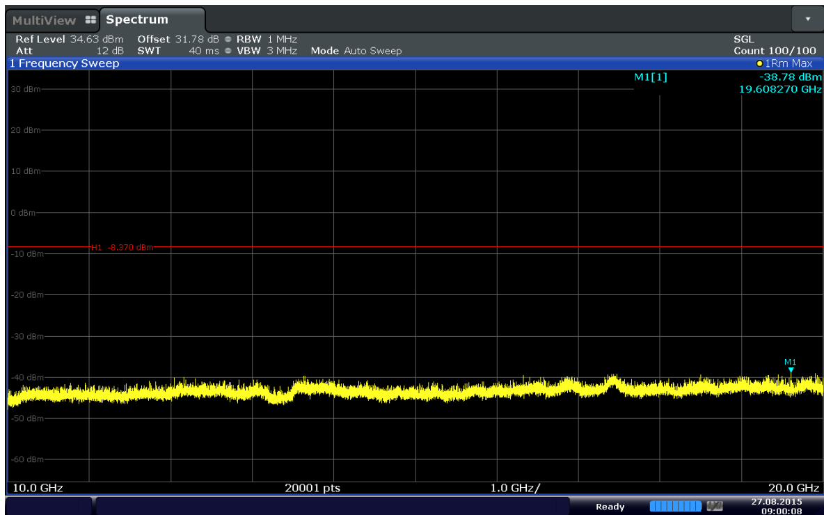
Plot 6-54. Conducted Spurious Plot (Band 4–20MHz–QPSK–RB Size 1–RB Offset 50–Ch.20050)
