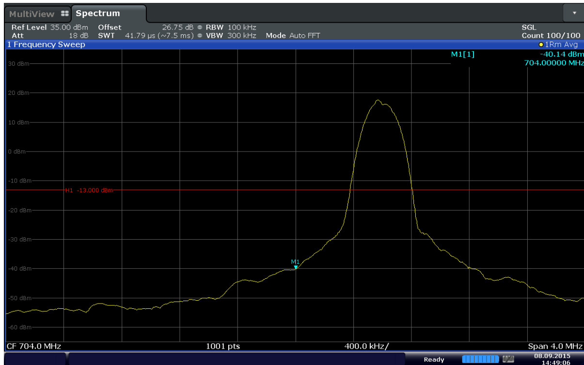
Plot 6-63. Lower Band Edge Plot (Band 17 – 10MHz – QPSK – RB Size 1 – RB Offset 0)
