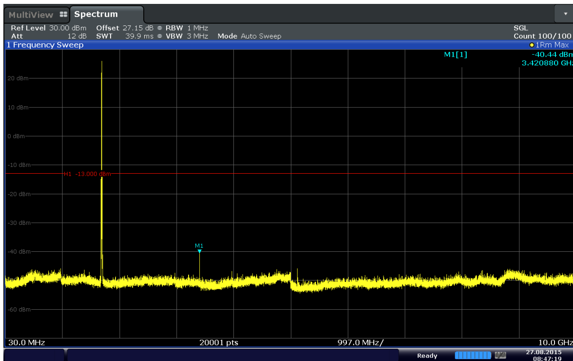
Plot 6-35. Conducted Spurious Plot (Band 4–5MHz–QPSK–RB Size 1–RB Offset 0–Ch.19975)
