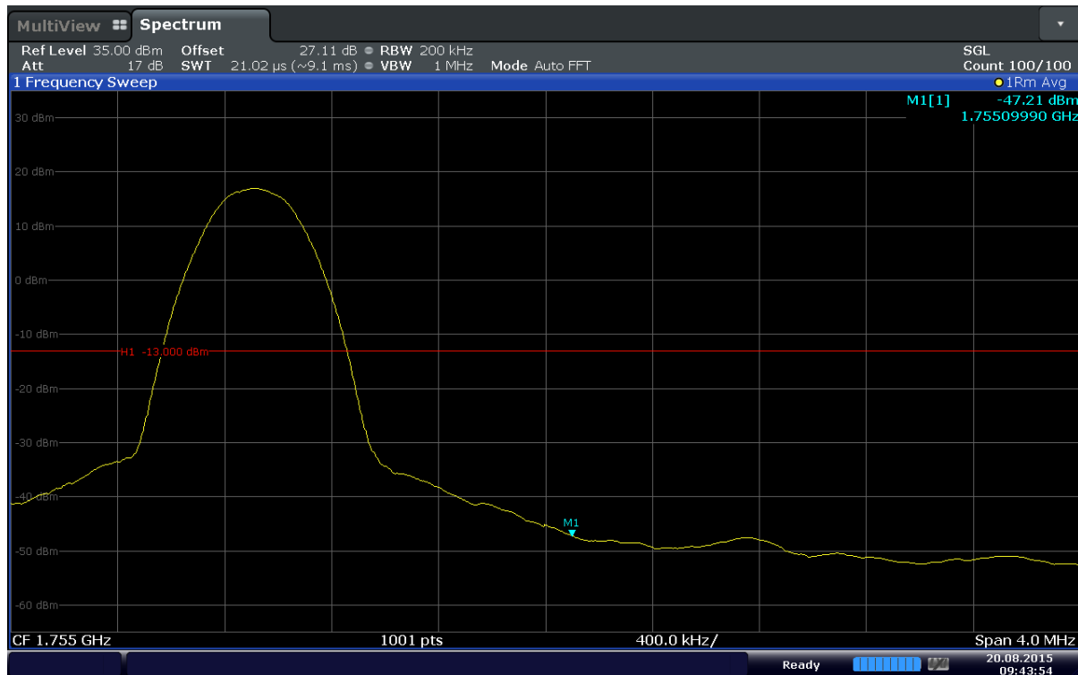
Plot 6-91. Upper Band Edge Plot (Band 4 – 20MHz – QPSK – RB Size 1 – RB Offset 99)
