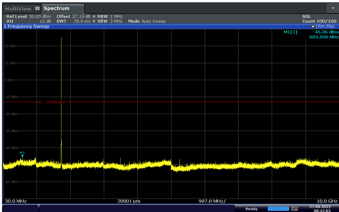
Plot 6-27. Conducted Spurious Plot (Band 4–1.4MHz–QPSK–RB Size 1–RB Offset 2–Ch.20393)
