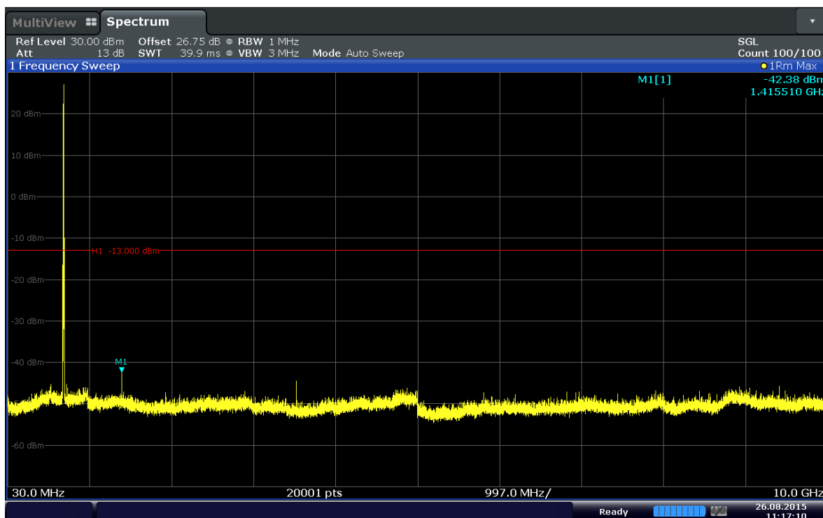
Plot 6-17. Conducted Spurious Plot (Band 17-5MHz-QPSK-RB Size 1-RB Offset 0-Ch.23755)85
