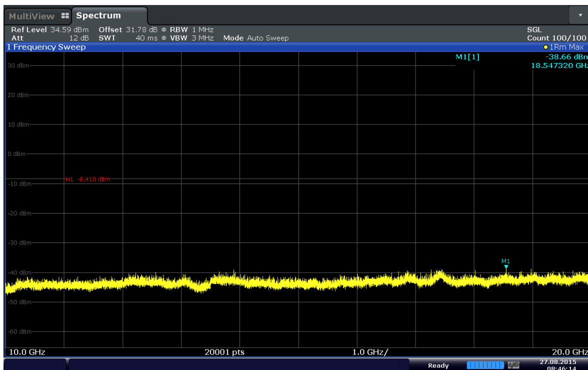
Plot 6-34. Conducted Spurious Plot (Band 4-3MHz-QPSK-RB Size 1-RB Offset 7-Ch.20385)
