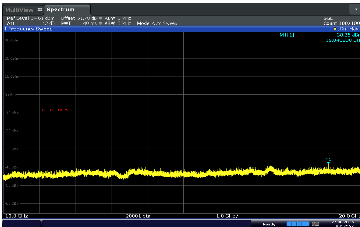
Plot 6-44. Conducted Spurious Plot (Band 4–10MHz–QPSK–RB Size 1–RB Offset 49–Ch.20175)
