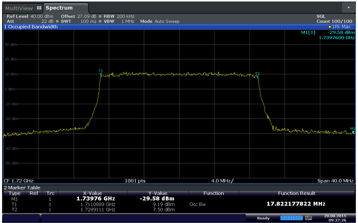
Plot 6-16. Occupied Bandwidth Plot (Band 4 - 20MHz 16QAM - RB Size 100)
