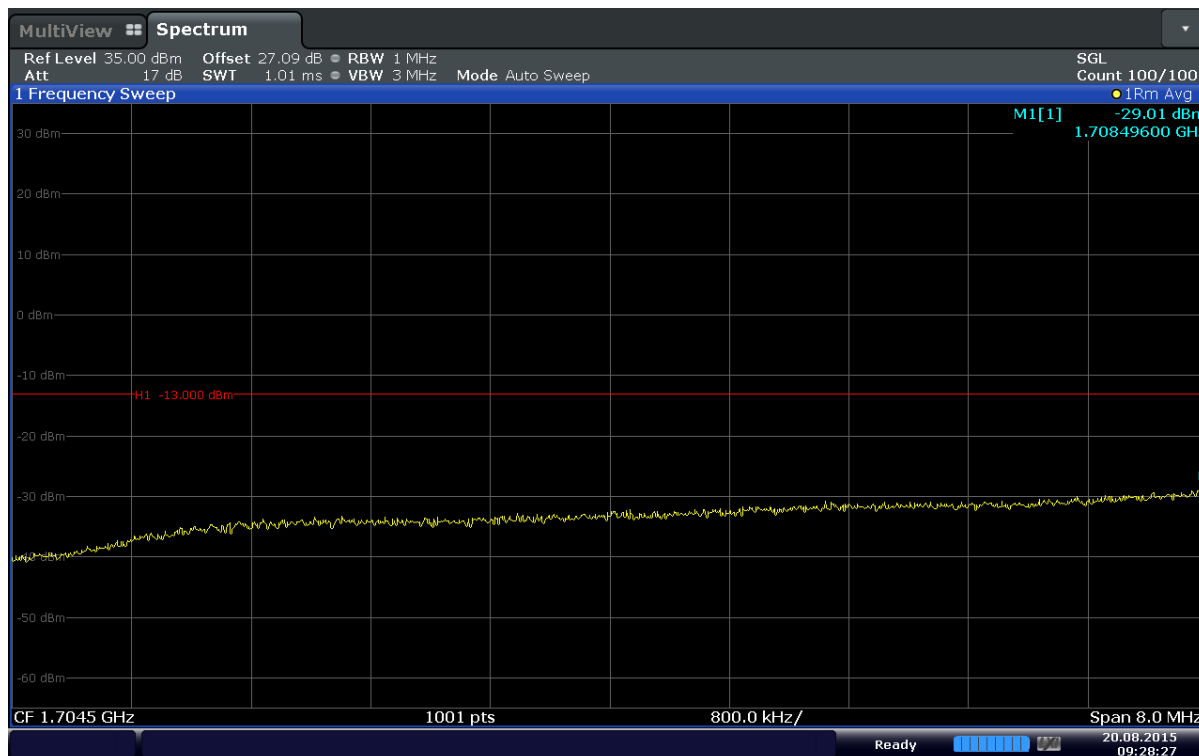
Plot 6-78. Extended Lower Band Edge Plot (Band 4 – 10MHz – QPSK – RB Size 50)
