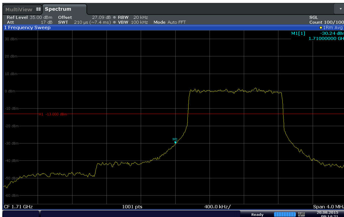
Plot 6-65. Lower Band Edge Plot (Band 4 – 1.4MHz – QPSK – RB Size 6)
