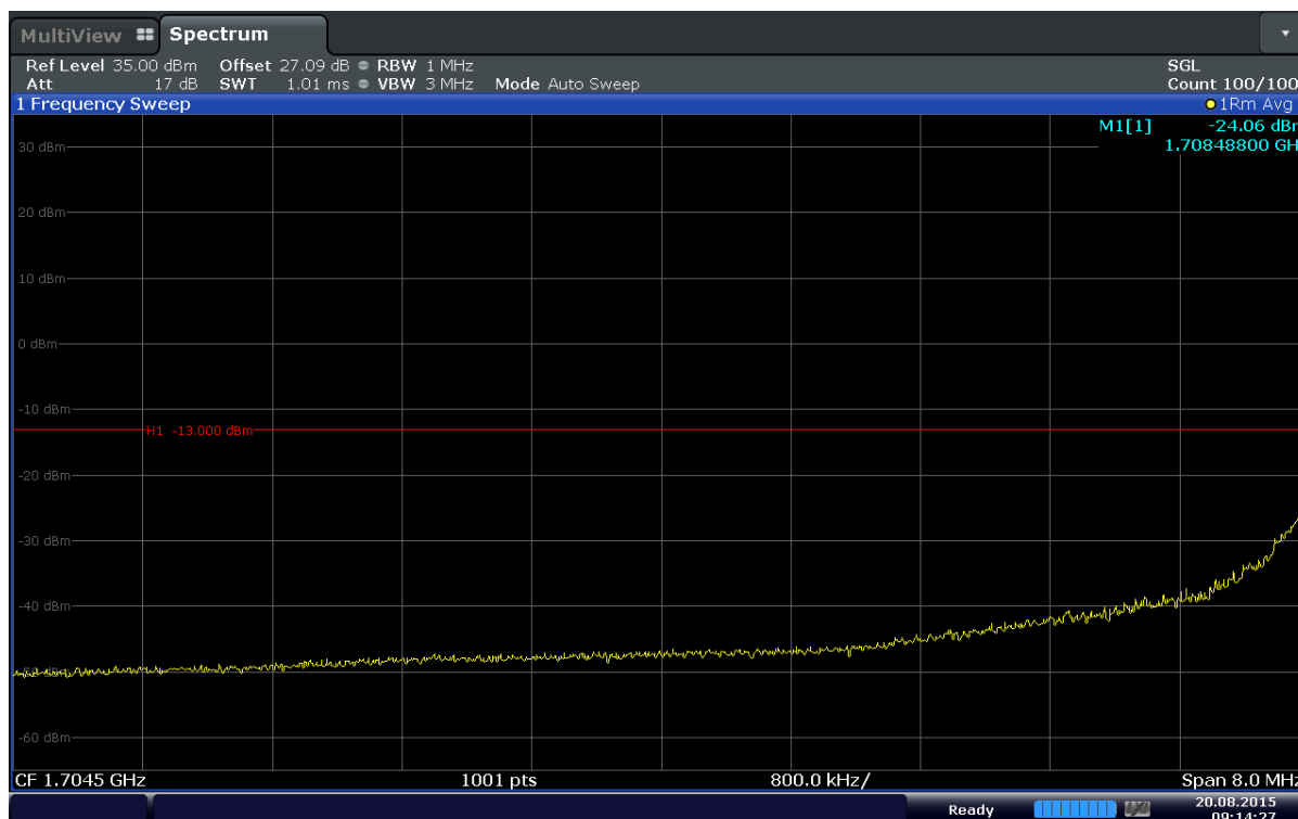
Plot 6-66. Extended Lower Band Edge Plot (Band 4 – 1.4MHz – QPSK – RB Size 6)
