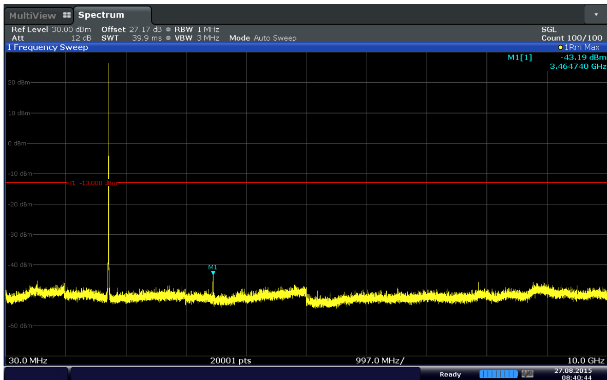
Plot 6-25. Conducted Spurious Plot (Band 4–1.4MHz–QPSK–RB Size 1–RB Offset 2–Ch.20175)
