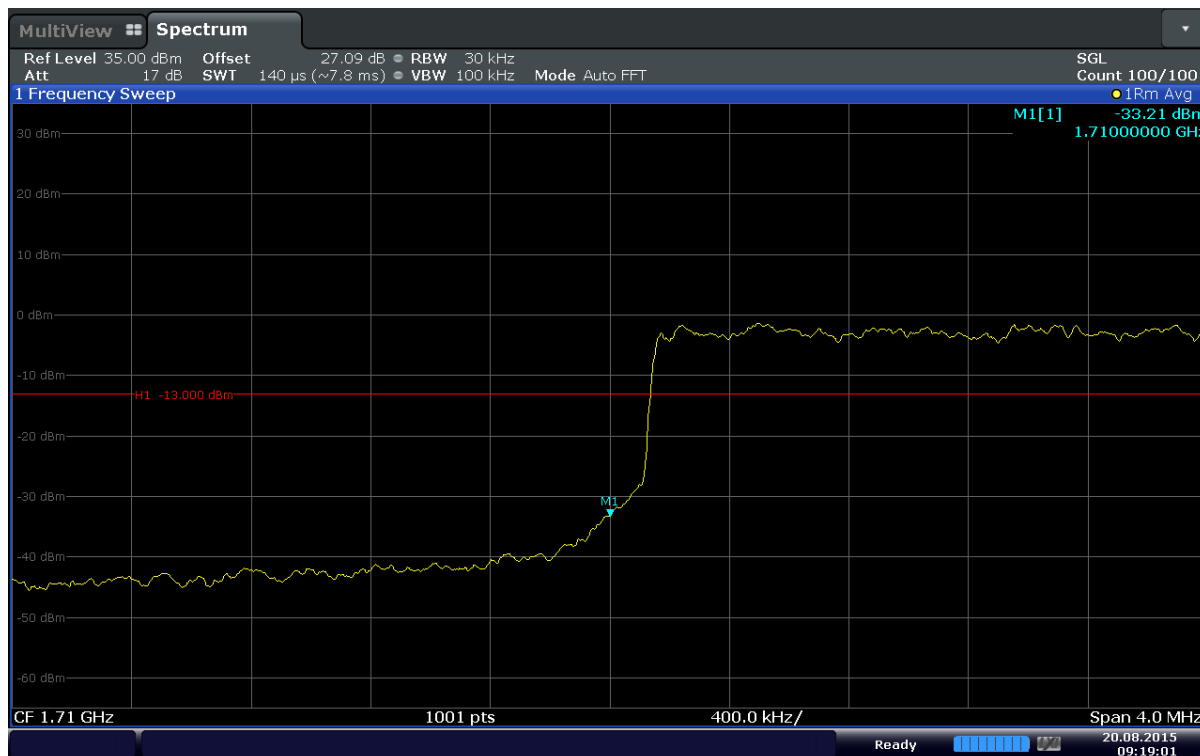
Plot 6-69. Lower Band Edge Plot (Band 4 – 3MHz – QPSK – RB Size 15)
