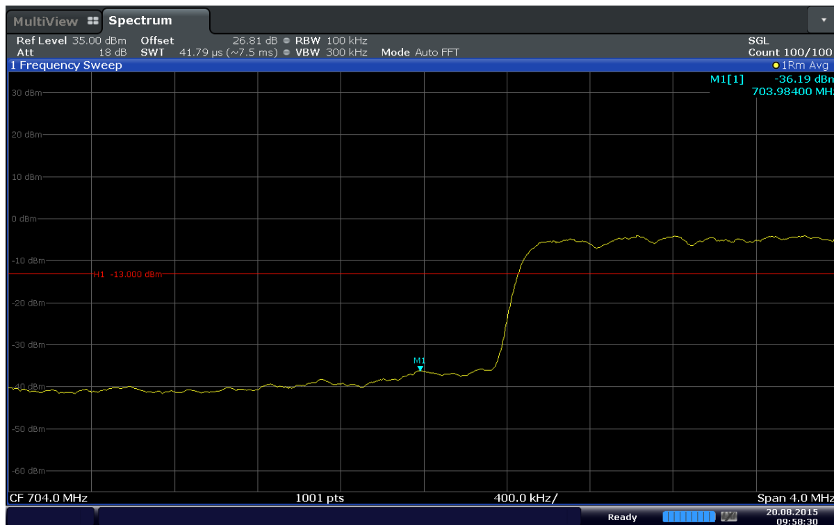
Plot 6-61. Lower Band Edge Plot (Band 17 – 10MHz – QPSK – RB Size 50)
