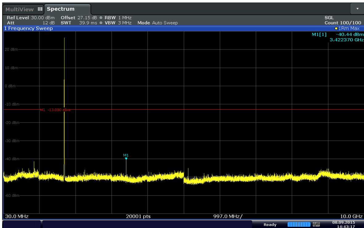
Plot 6-23. Conducted Spurious Plot (Band 4–1.4MHz–QPSK–RB Size 1–RB Offset 2–Ch.19957)
