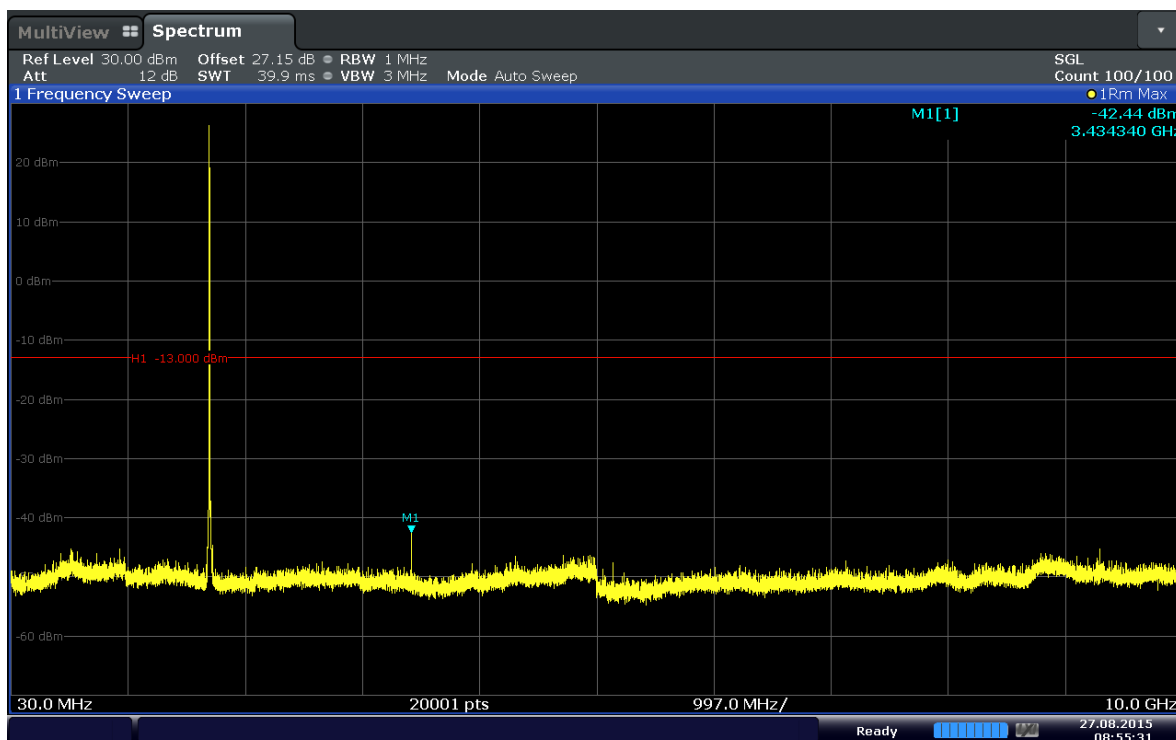
Plot 6-47. Conducted Spurious Plot (Band 4–15MHz–QPSK–RB Size 1–RB Offset 36–Ch.20025)
