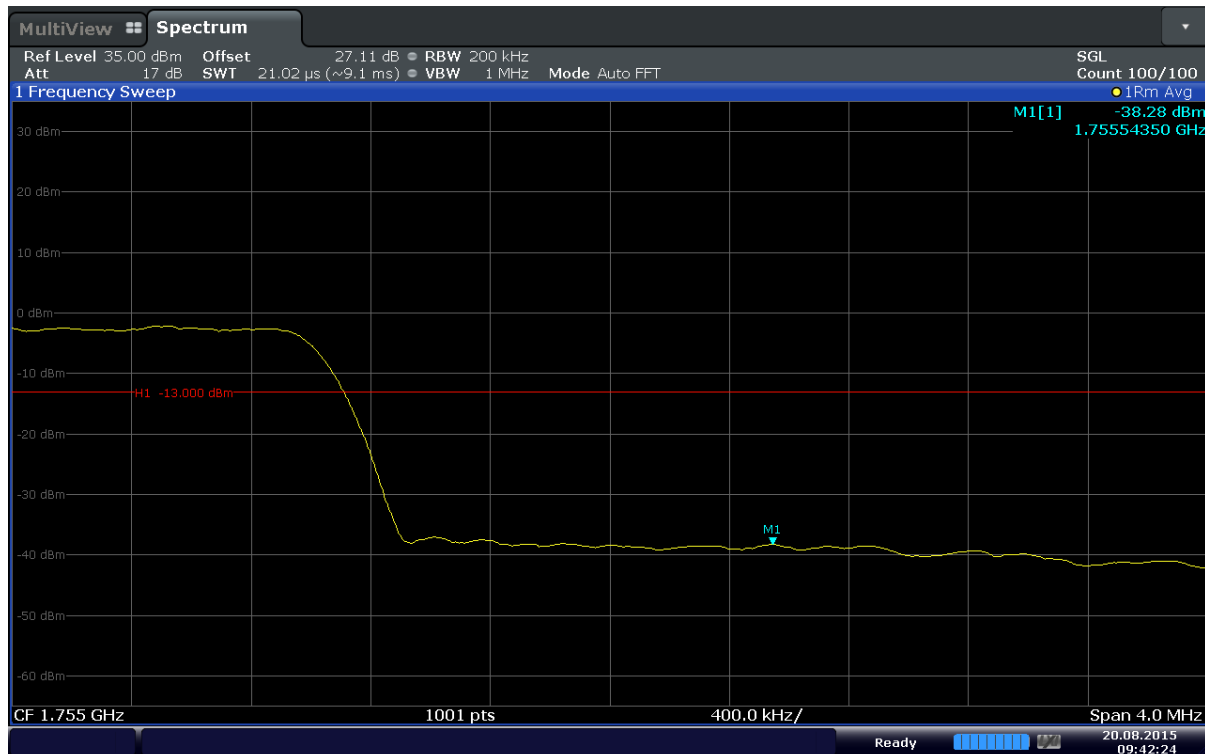
Plot 6-87. Upper Band Edge Plot (Band 4 – 20MHz – QPSK – RB Size 100)
