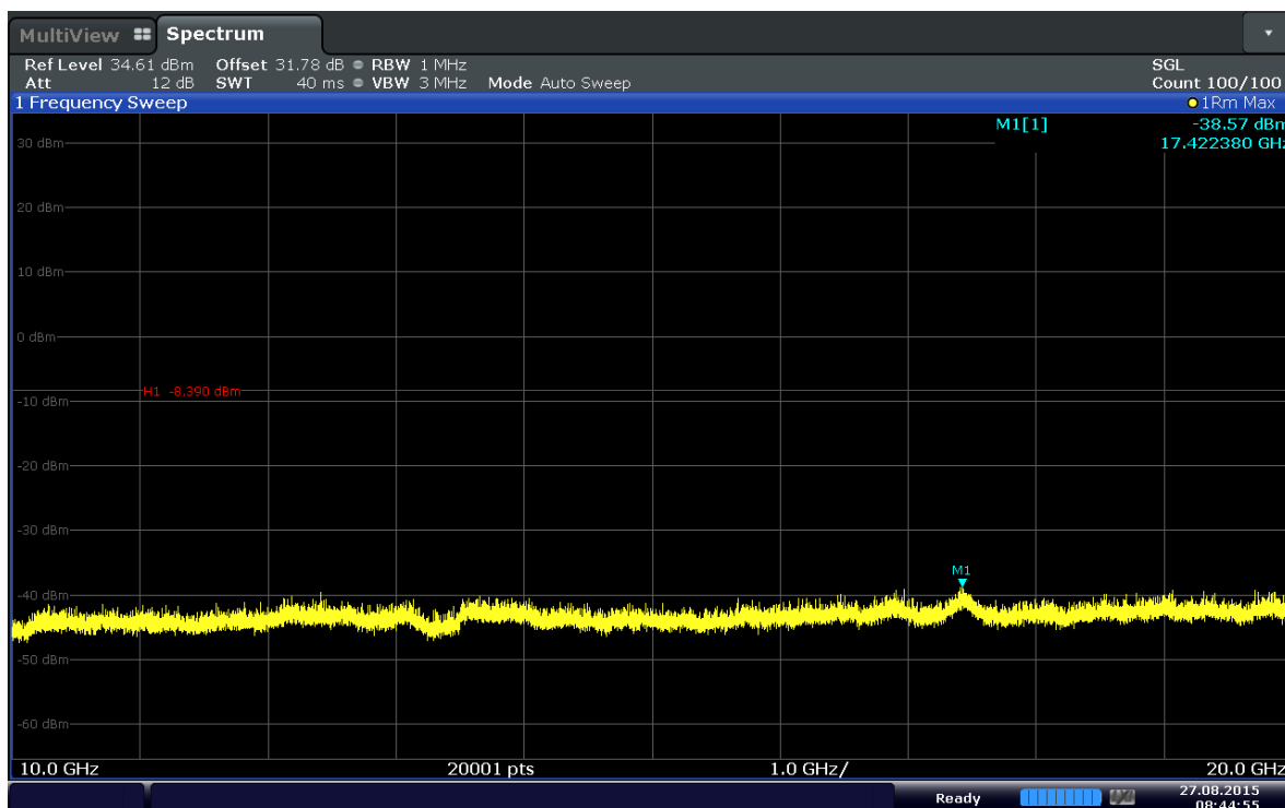
Plot 6-32. Conducted Spurious Plot (Band 4–3MHz–QPSK–RB Size 1–RB Offset 14–Ch.20175)
