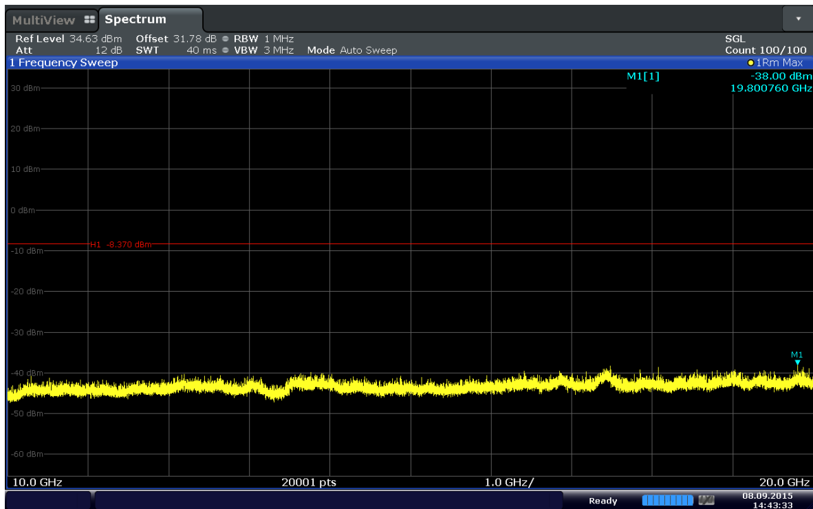
Plot 6-24. Conducted Spurious Plot (Band 4–1.4MHz–QPSK–RB Size 1–RB Offset 2–Ch.19957)
