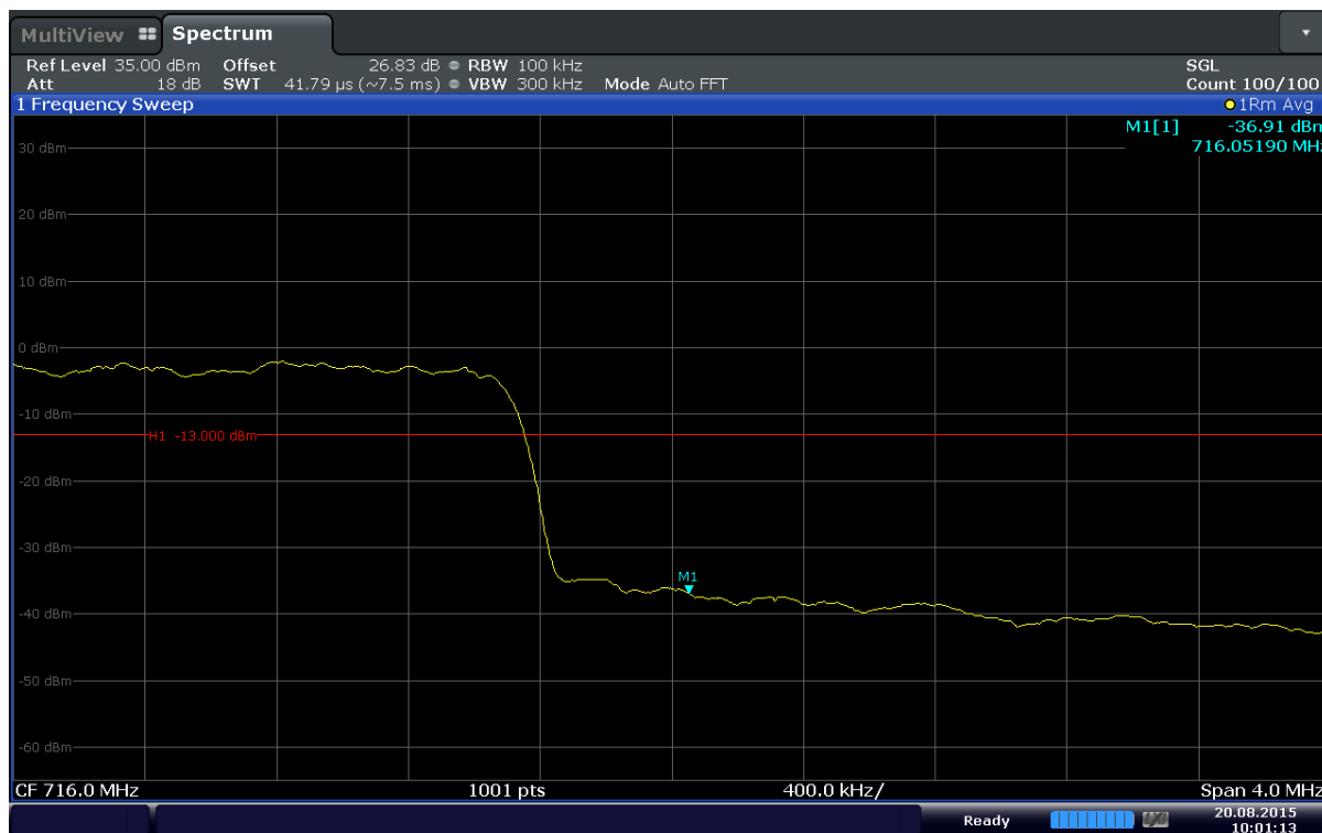
Plot 6-62. Upper Band Edge Plot (Band 17 – 10MHz – QPSK – RB Size 50)
