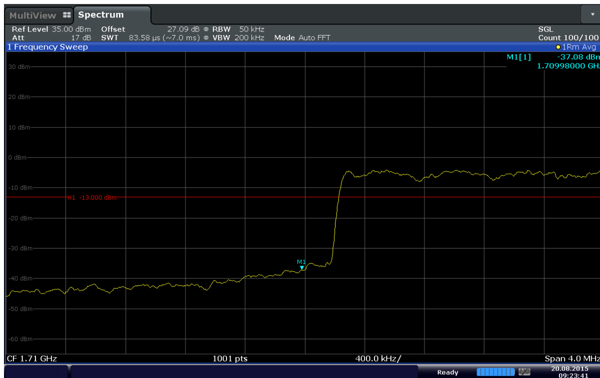
Plot 6-73. Lower Band Edge Plot (Band 4 – 5MHz – QPSK – RB Size 25)
