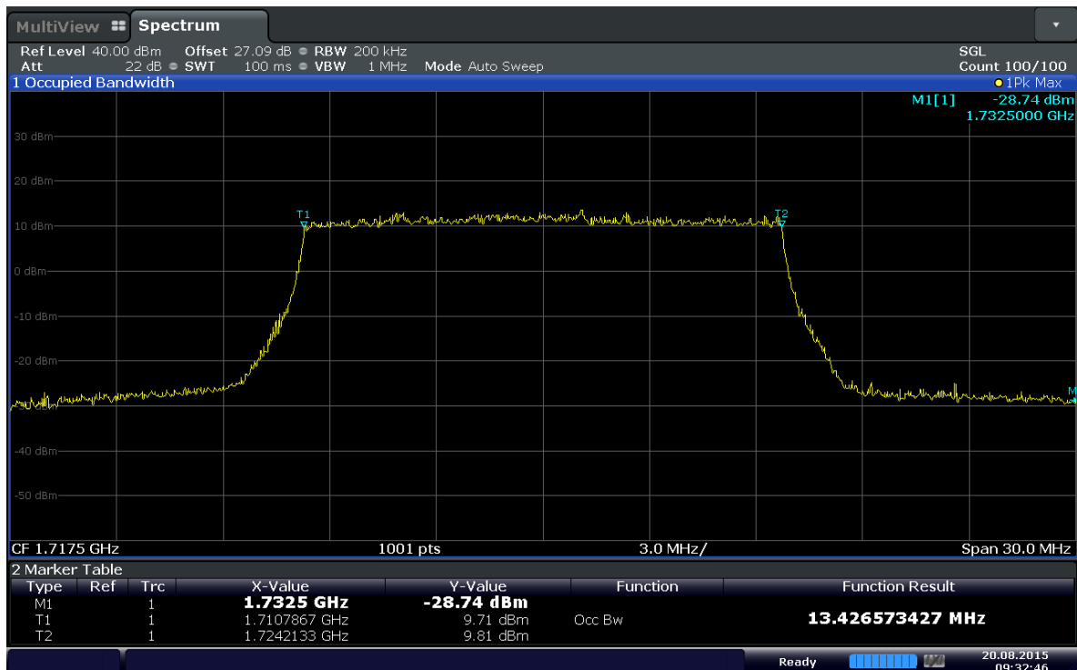
Plot 6-14. Occupied Bandwidth Plot (Band 4 - 15MHz 16QAM - RB Size 75)
