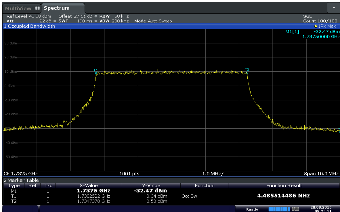
Plot 6-10. Occupied Bandwidth Plot (Band 4 – 5MHz 16QAM - RB Size 25)
