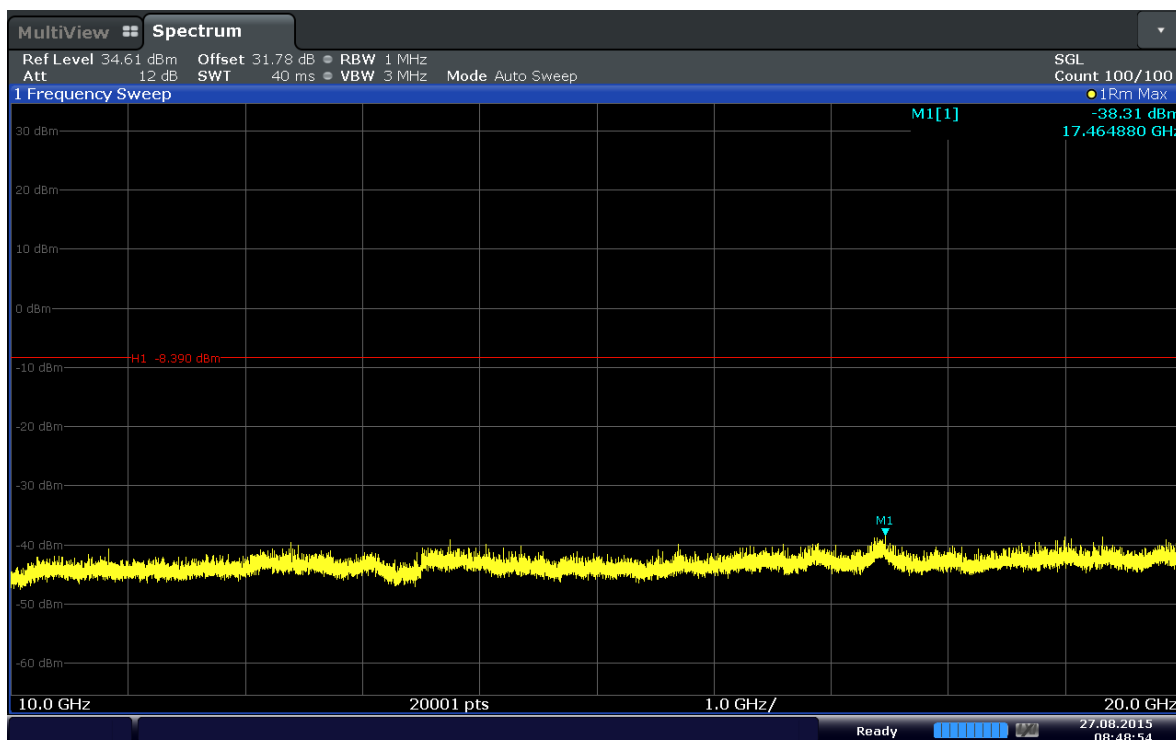
Plot 6-38. Conducted Spurious Plot (Band 4–5MHz–QPSK–RB Size 1–RB Offset 12–Ch.20175)
