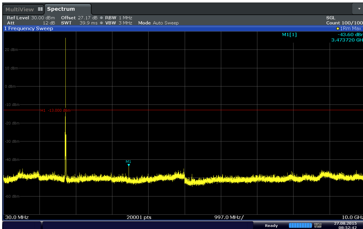
Plot 6-43. Conducted Spurious Plot (Band 4–10MHz–QPSK–RB Size 1–RB Offset 49–Ch.20175)
