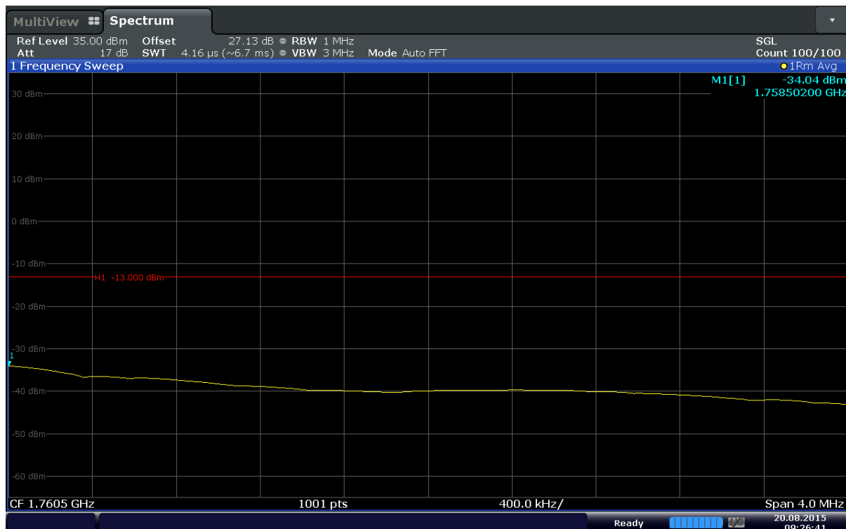
Plot 6-76. Extended Upper Band Edge Plot (Band 4 – 5MHz – QPSK – RB Size 25)
