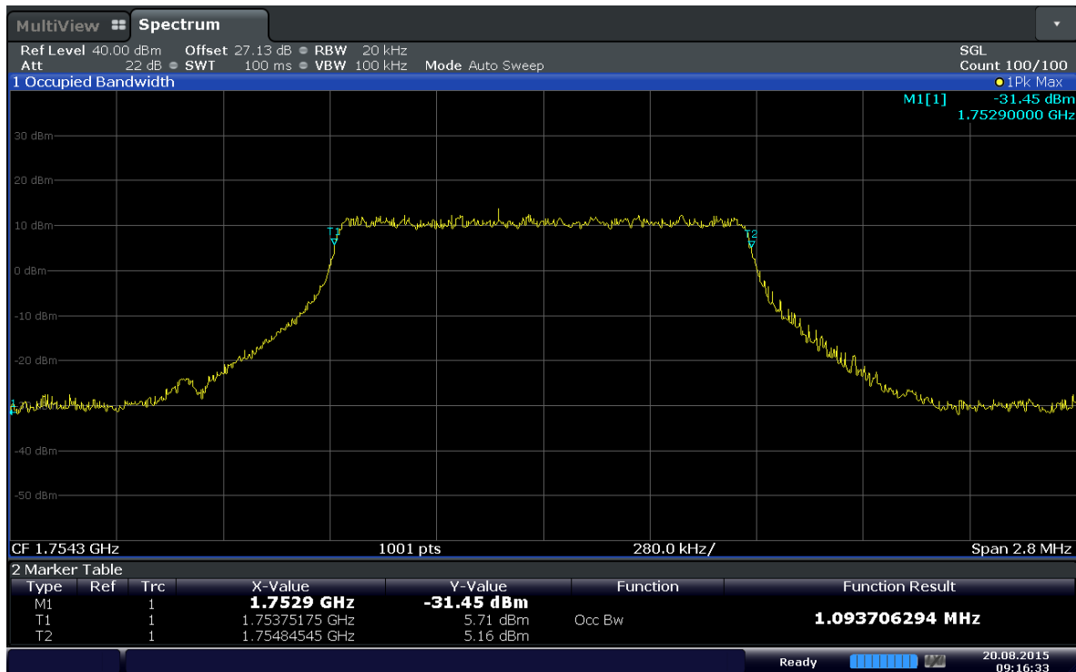
Plot 6-5. Occupied Bandwidth Plot (Band 4 – 1.4MHz QPSK - RB Size 6)
