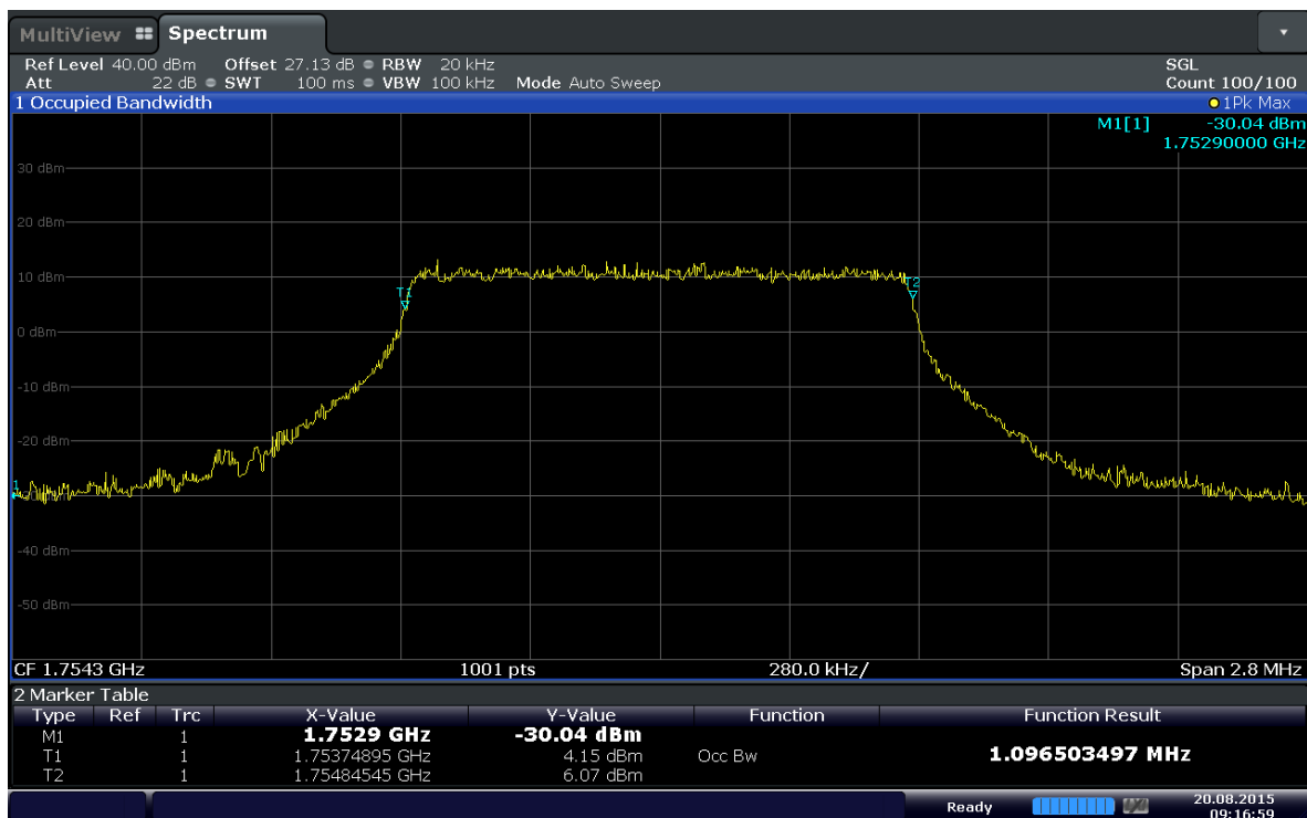
Plot 6-6. Occupied Bandwidth Plot (Band 4 – 1.4MHz 16QAM - RB Size 6)
