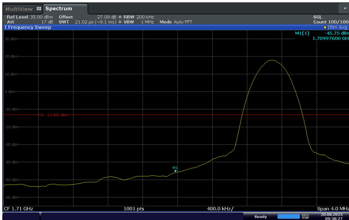
Plot 6-89. Lower Band Edge Plot (Band 4 – 20MHz – QPSK – RB Size 1 – RB Offset 0)
