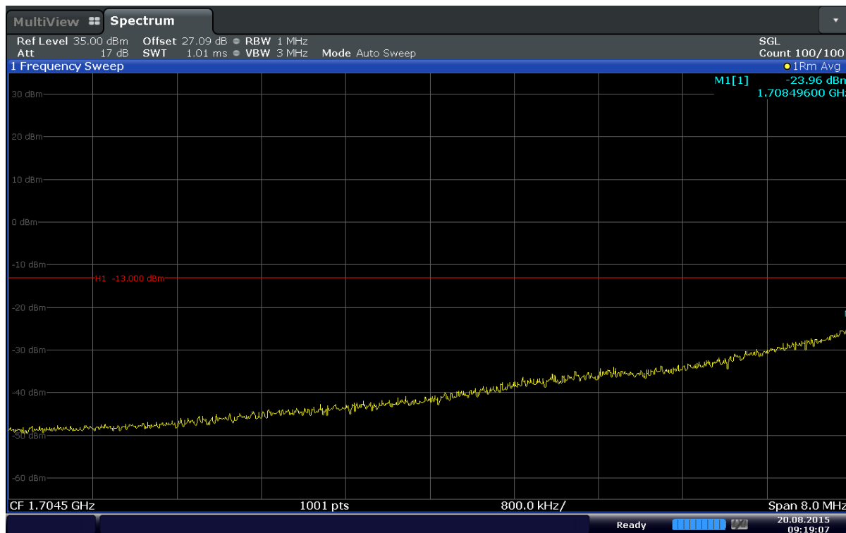
Plot 6-70. Extended Lower Band Edge Plot (Band 4 – 3MHz – QPSK – RB Size 15)
