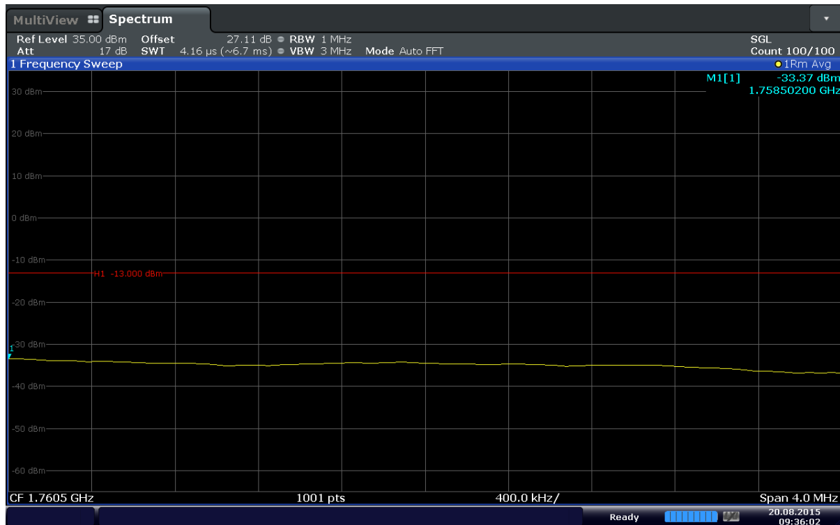
Plot 6-84. Extended Upper Band Edge Plot (Band 4 – 15MHz – QPSK – RB Size 75)
