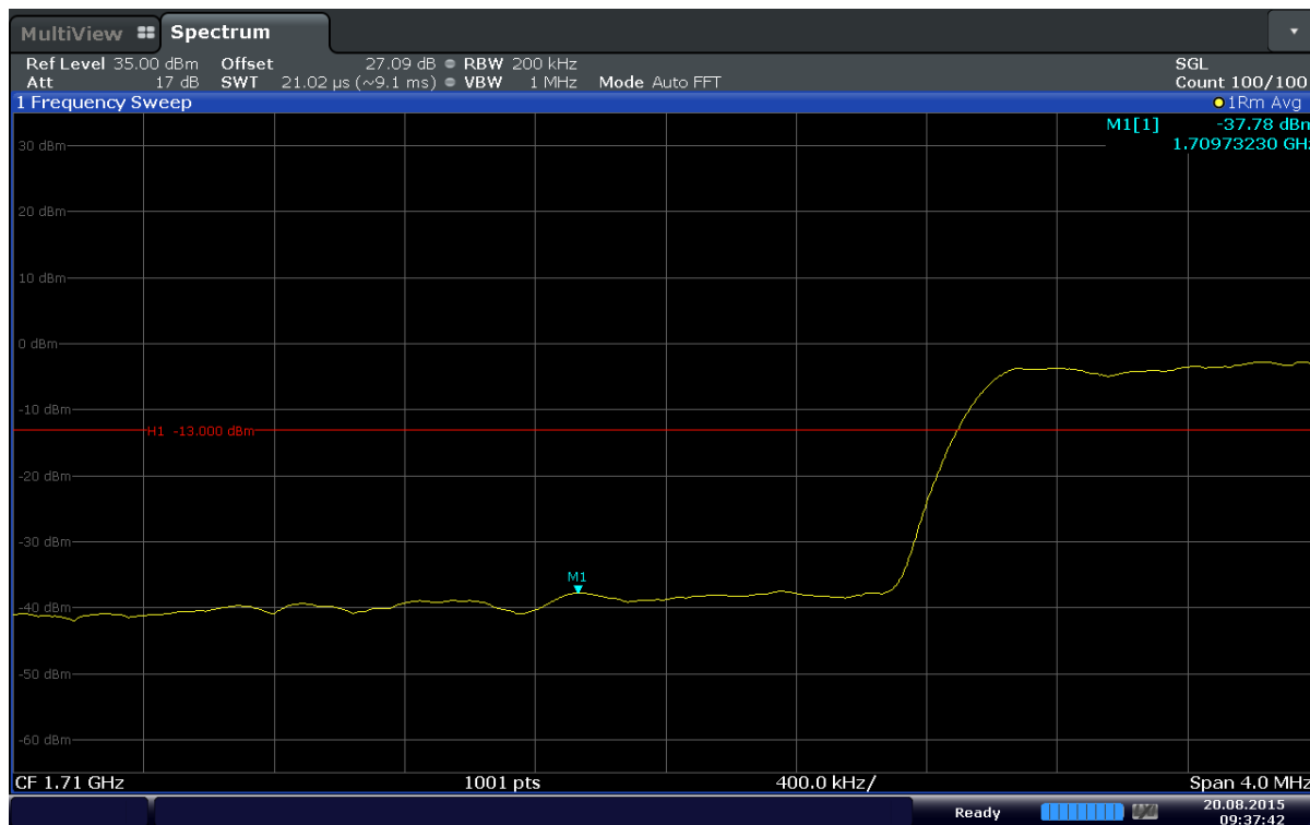
Plot 6-85. Lower Band Edge Plot (Band 4 – 20MHz – QPSK – RB Size 100)
