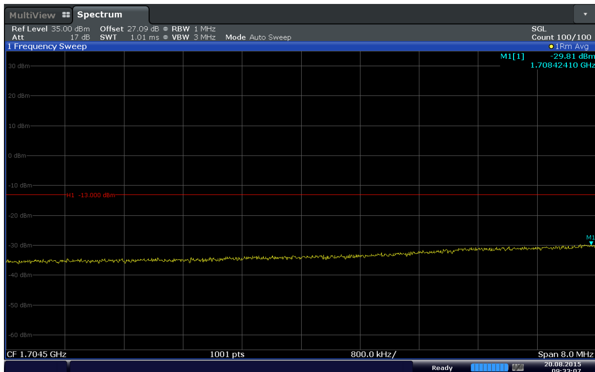
Plot 6-82. Extended Lower Band Edge Plot (Band 4 – 15MHz – QPSK – RB Size 75)
