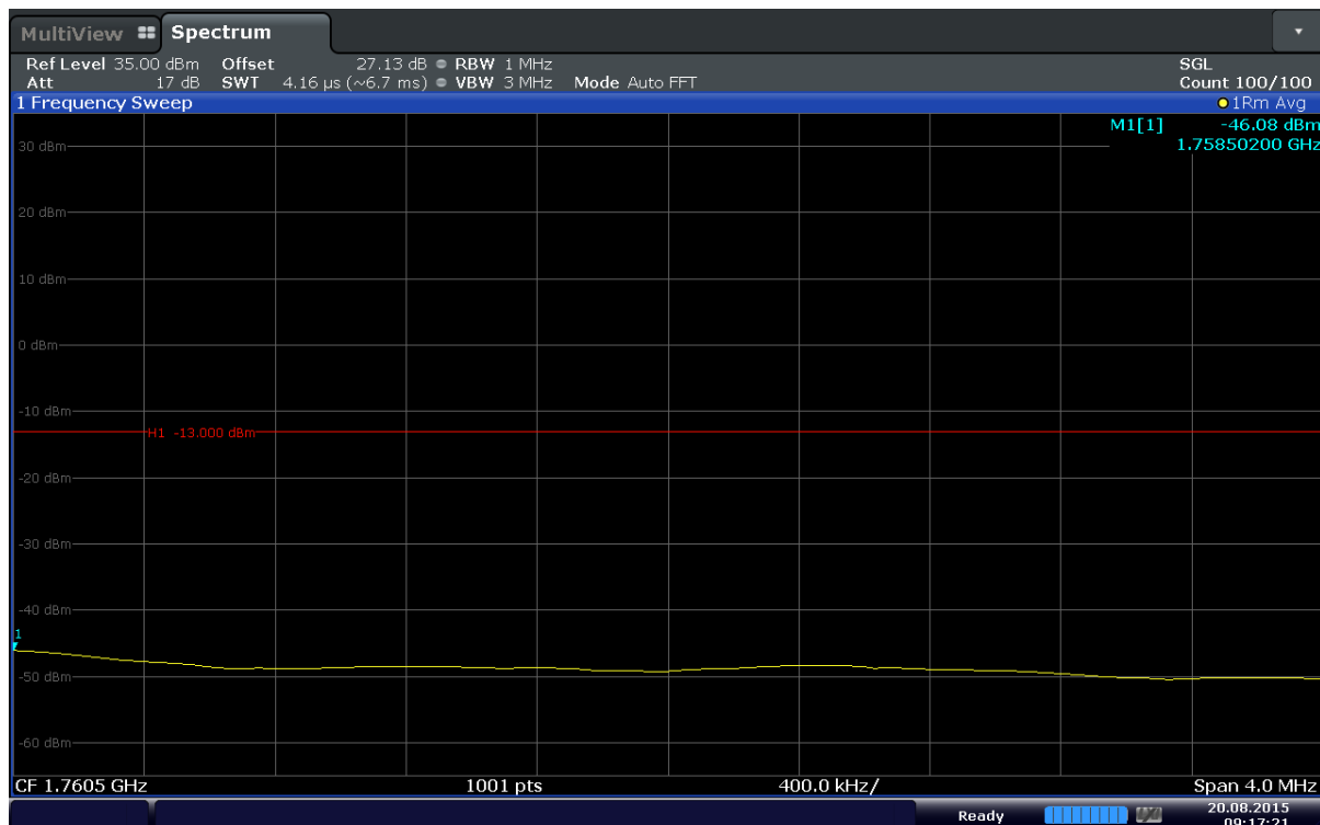
Plot 6-68. Extended Upper Band Edge Plot (Band 4 – 1.4MHz – QPSK – RB Size 6)
