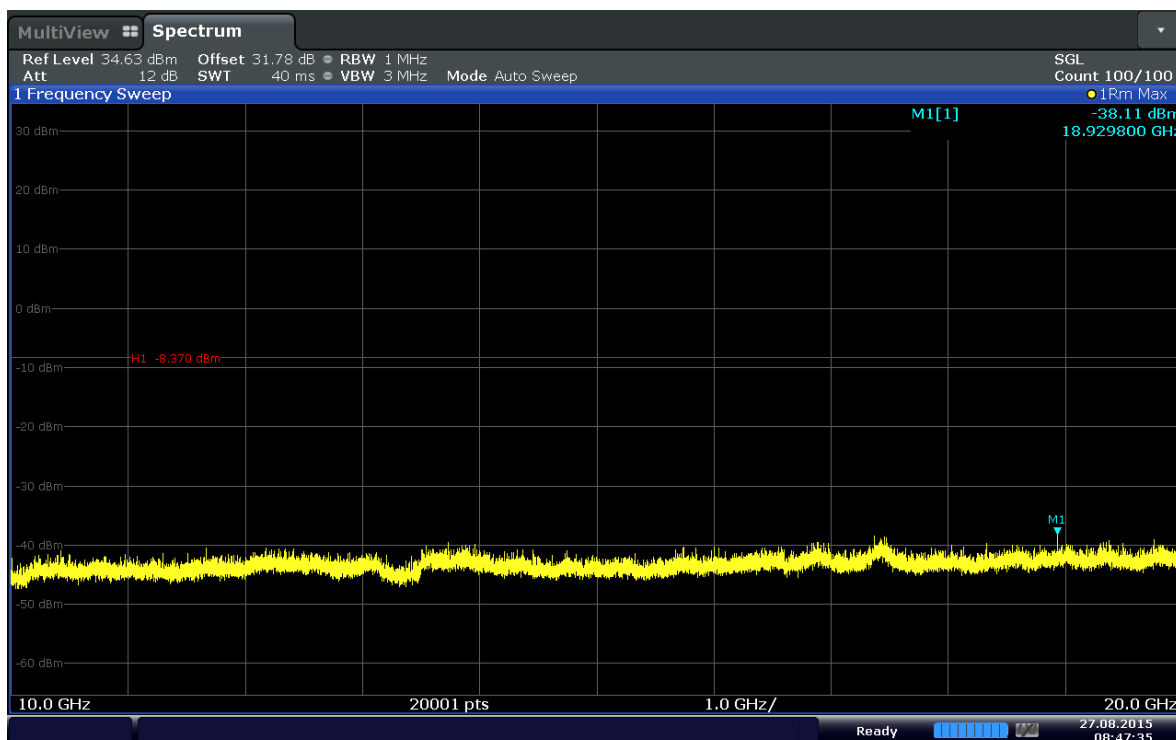
Plot 6-36. Conducted Spurious Plot (Band 4–5MHz–QPSK–RB Size 1–RB Offset 0–Ch.19975)
