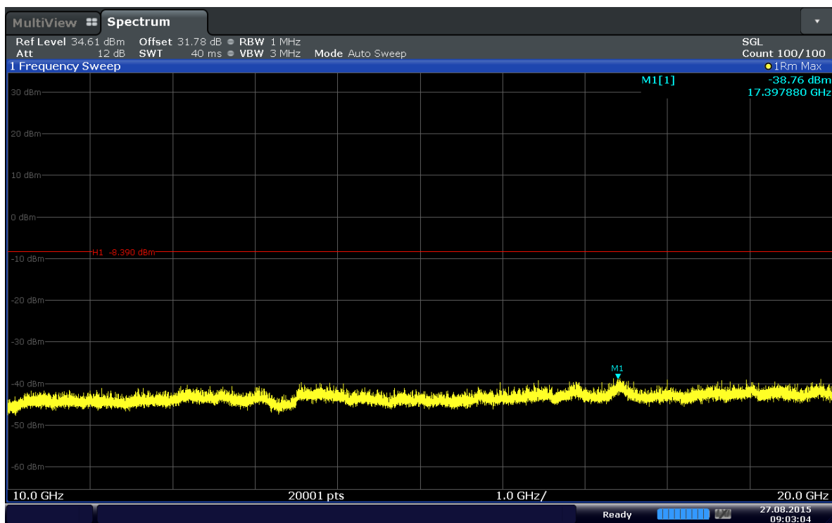
Plot 6-58. Conducted Spurious Plot (Band 4–20MHz–QPSK–RB Size 1–RB Offset 99–Ch.20300)
