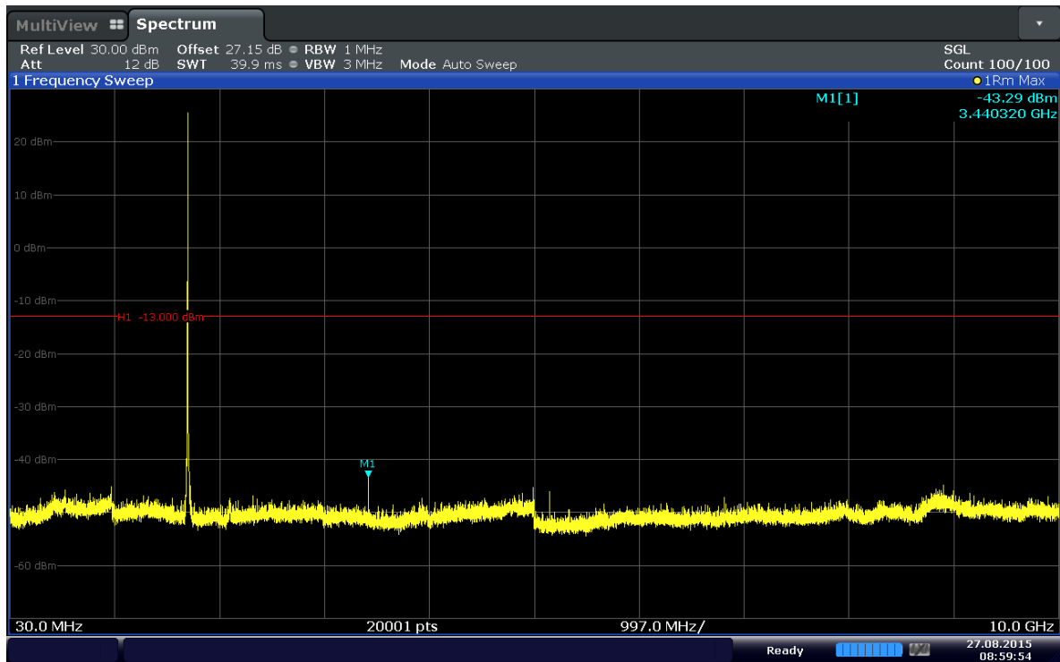
Plot 6-53. Conducted Spurious Plot (Band 4–20MHz–QPSK–RB Size 1–RB Offset 50–Ch.20050)
