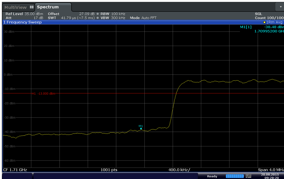
Plot 6-77. Lower Band Edge Plot (Band 4 – 10MHz – QPSK – RB Size 50)
