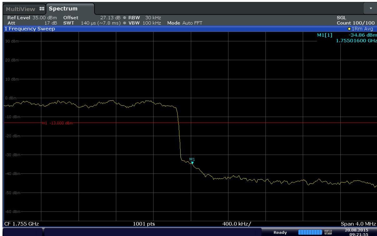
Plot 6-71. Upper Band Edge Plot (Band 4 – 3MHz – QPSK – RB Size 15)
