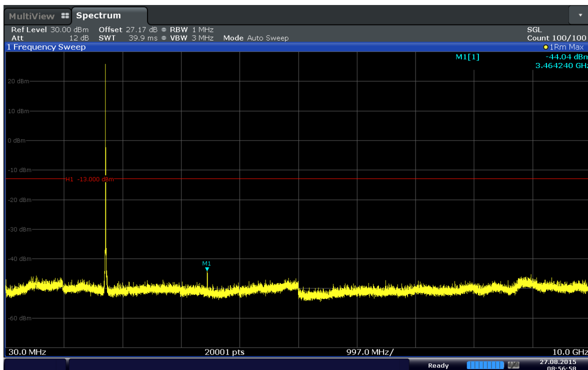
Plot 6-49. Conducted Spurious Plot (Band 4–15MHz–QPSK–RB Size 1–RB Offset 36–Ch.20175)
