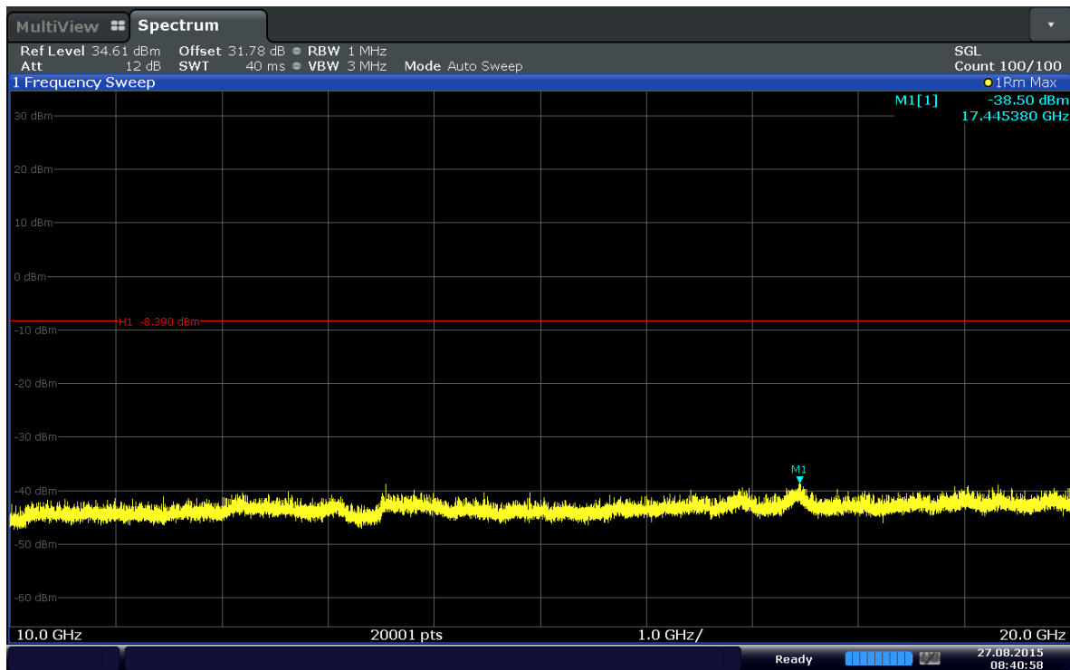
Plot 6-26. Conducted Spurious Plot (Band 4–1.4MHz–QPSK–RB Size 1–RB Offset 2–Ch.20175)
