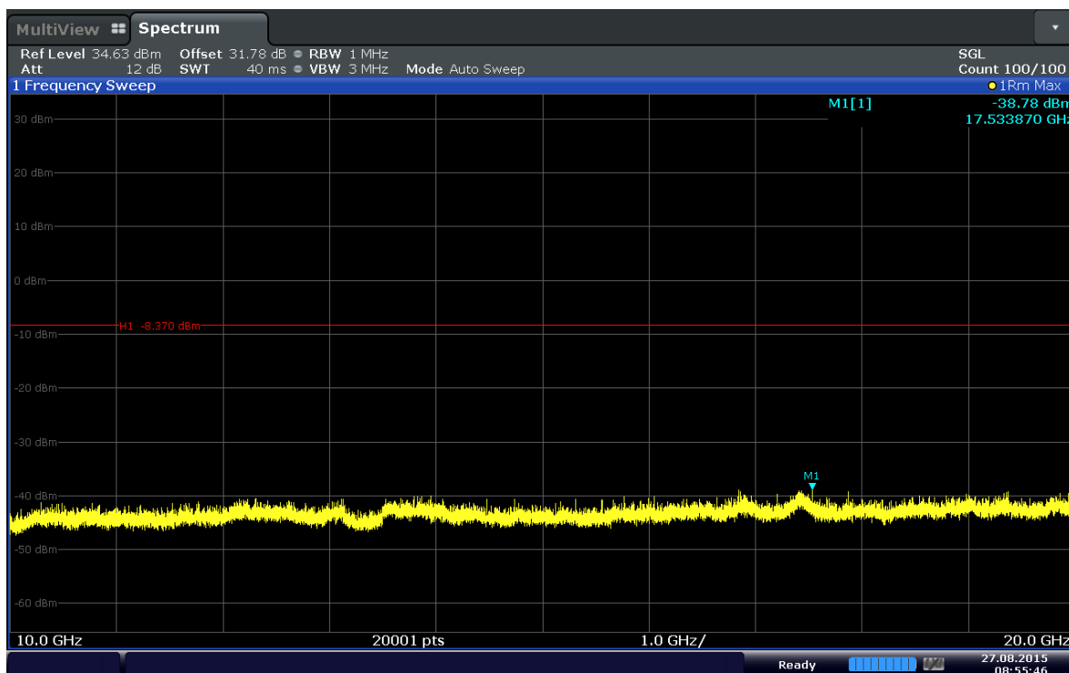
Plot 6-48. Conducted Spurious Plot (Band 4–15MHz–QPSK–RB Size 1–RB Offset 36–Ch.20025)
