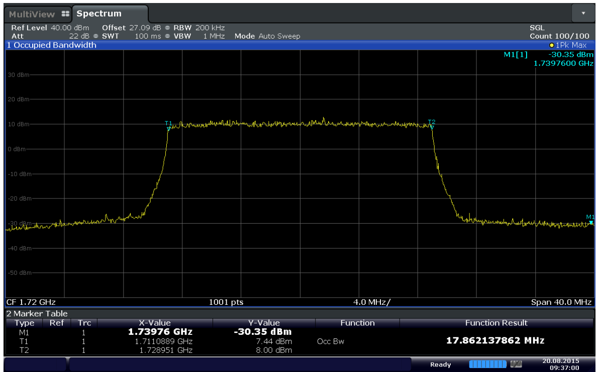
Plot 6-15. Occupied Bandwidth Plot (Band 4 - 20MHz QPSK - RB Size 100)
