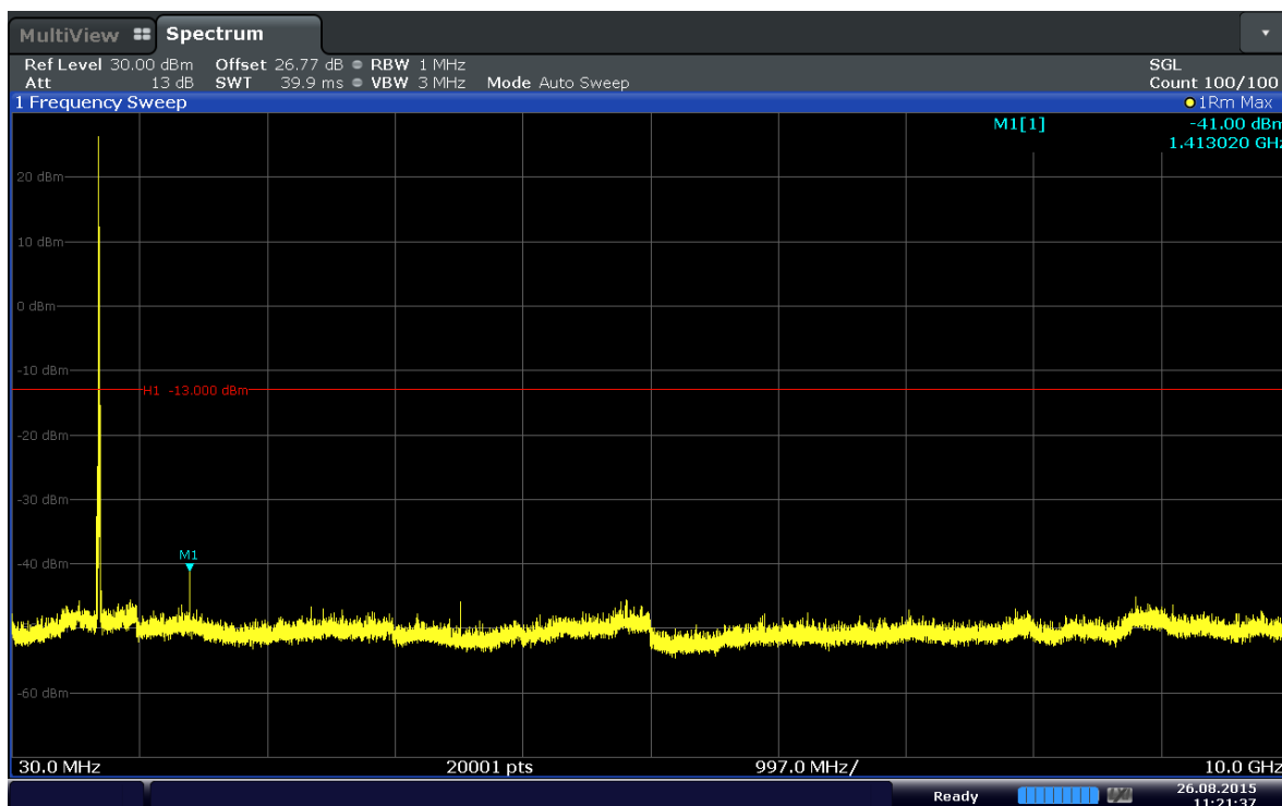
Plot 6-22. Conducted Spurious Plot (Band 17–10MHz–QPSK–RB Size 1–RB Offset 0–Ch.23800)
