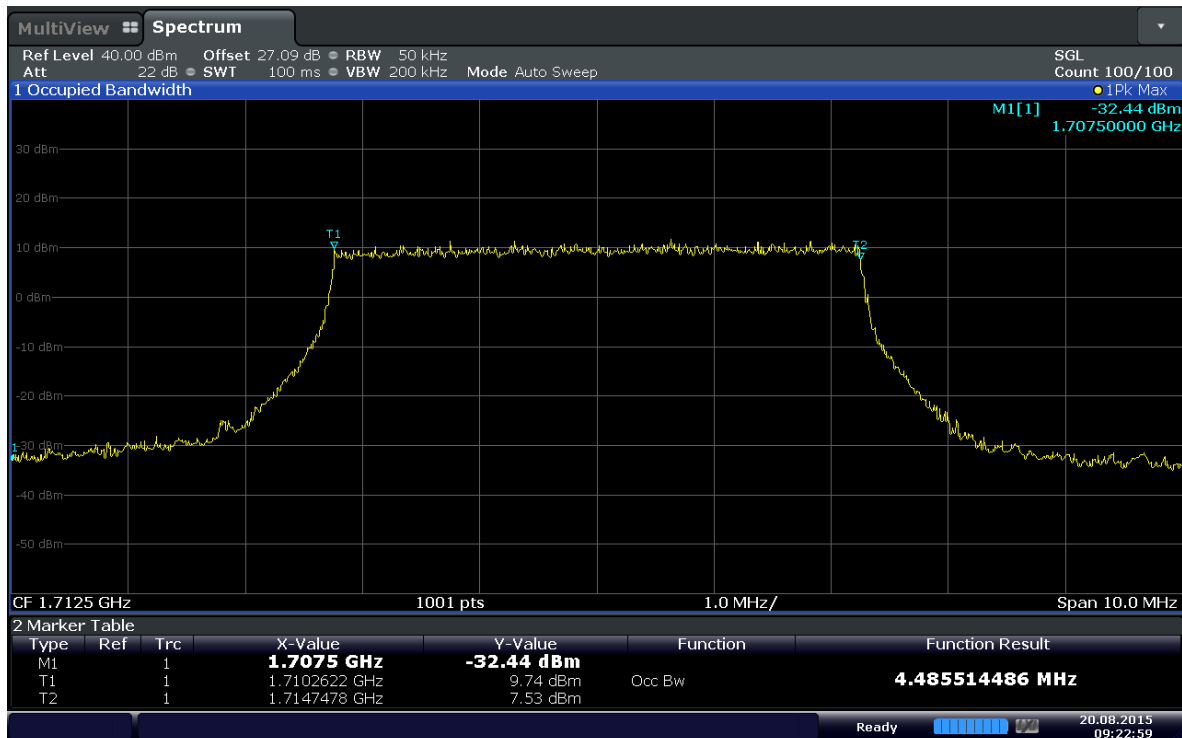
Plot 6-9. Occupied Bandwidth Plot (Band 4 – 5MHz QPSK - RB Size 25)
