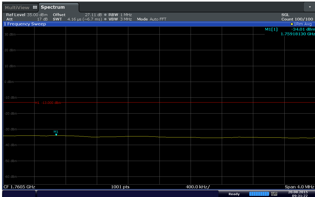
Plot 6-80. Extended Upper Band Edge Plot (Band 4 – 10MHz – QPSK – RB Size 50)
