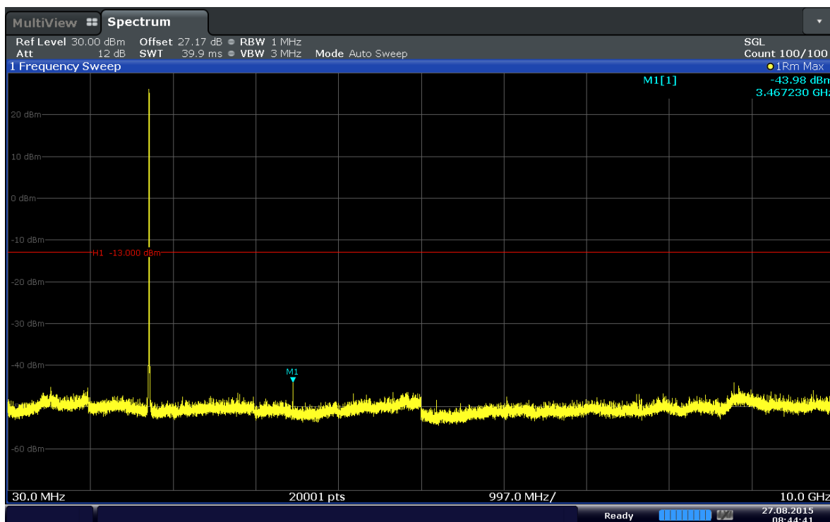
Plot 6-31. Conducted Spurious Plot (Band 4–3MHz–QPSK–RB Size 1–RB Offset 14–Ch.20175)
