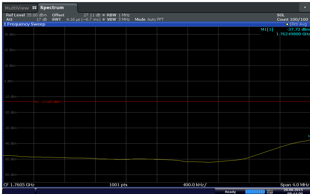
Plot 6-92. Extended Upper Band Edge Plot (Band 4 – 20MHz – QPSK – RB Size 1 – RB Offset 99)
