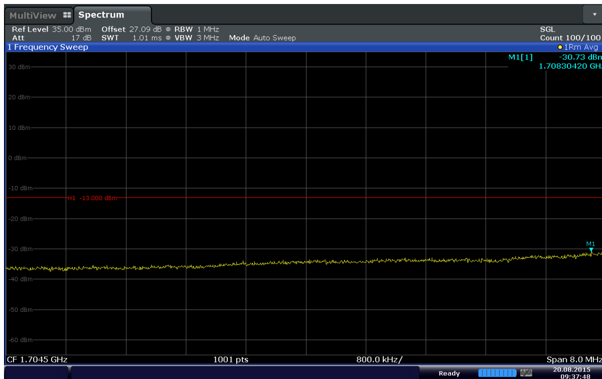
Plot 6-86. Extended Lower Band Edge Plot (Band 4 – 20MHz – QPSK – RB Size 100)
