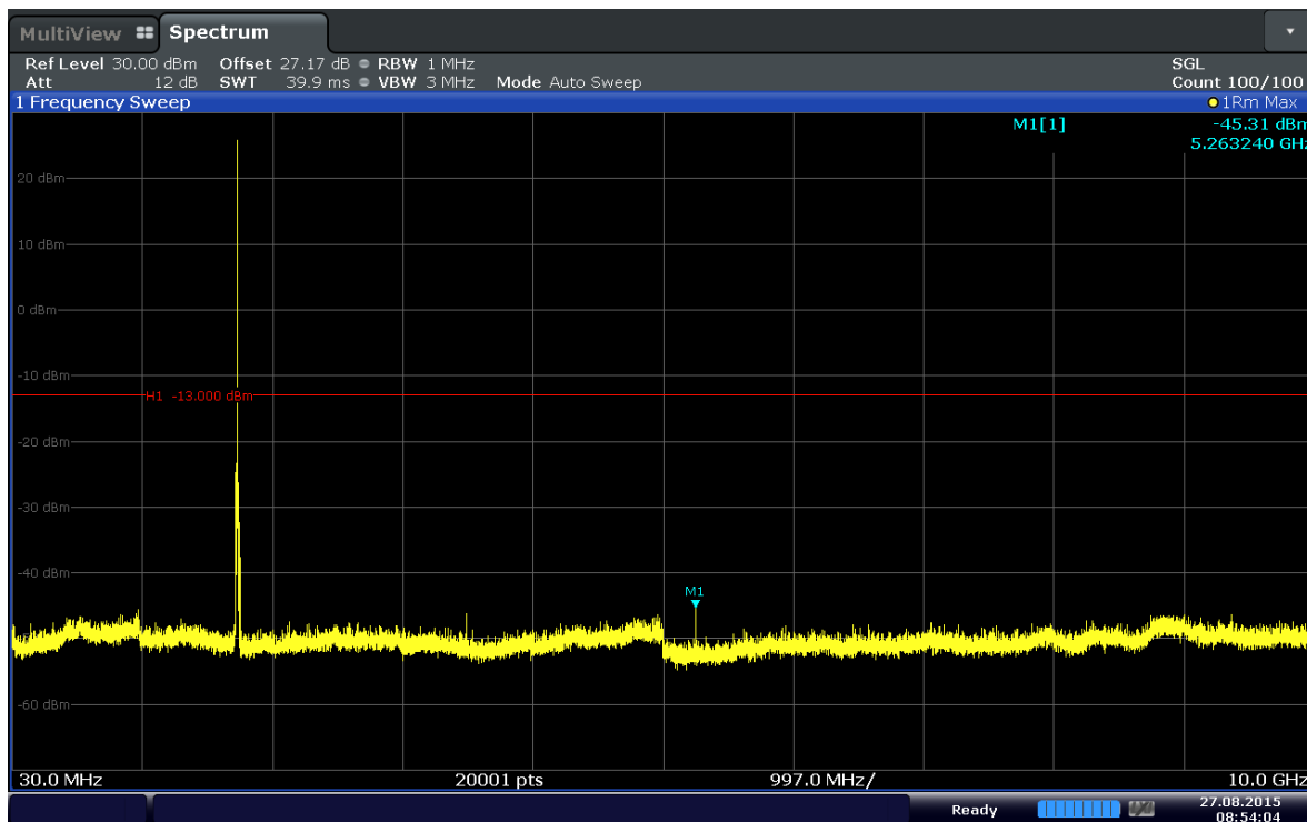
Plot 6-45. Conducted Spurious Plot (Band 4–10MHz–QPSK–RB Size 1–RB Offset 49–Ch.20350)
