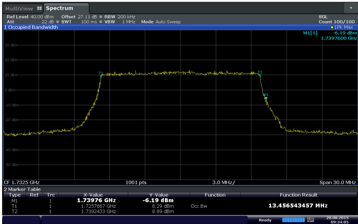
Plot 6-13. Occupied Bandwidth Plot (Band 4 - 15MHz QPSK - RB Size 75)
