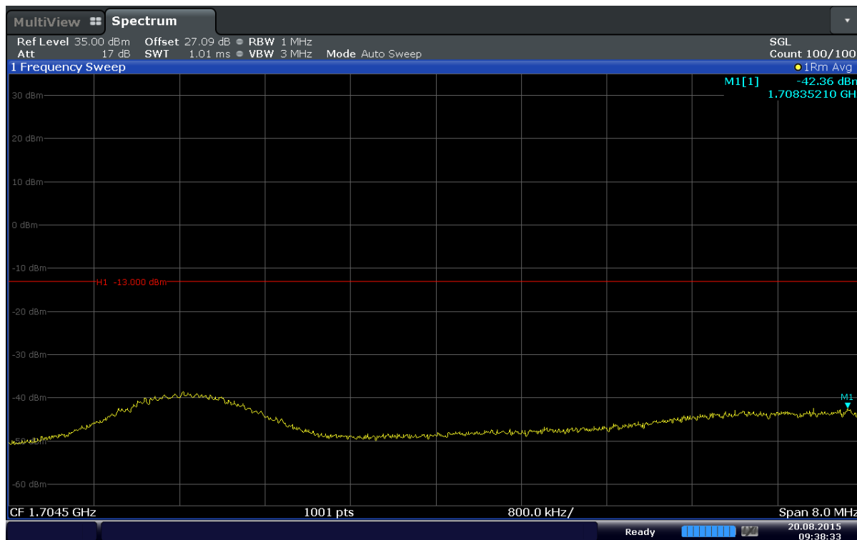
Plot 6-90. Extended Lower Band Edge Plot (Band 4 – 20MHz – QPSK – RB Size 1 – RB Offset 0)
