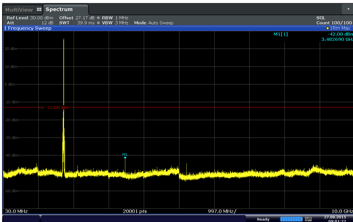
Plot 6-55. Conducted Spurious Plot (Band 4–20MHz–QPSK–RB Size 1–RB Offset 99–Ch.20175)
