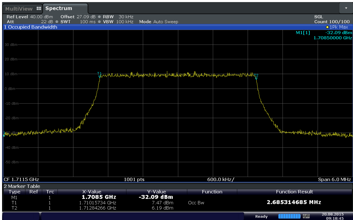
Plot 6-8. Occupied Bandwidth Plot (Band 4 – 3MHz 16QAM - RB Size 15)
