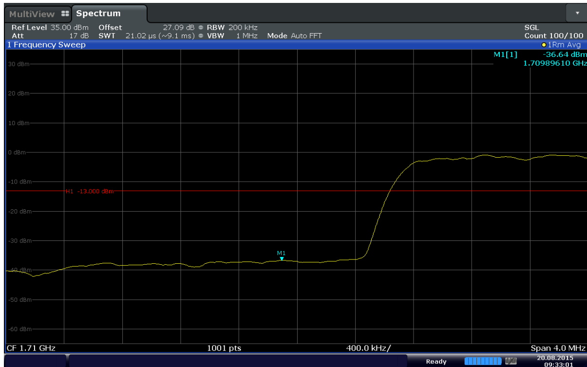
Plot 6-81. Lower Band Edge Plot (Band 4 – 15MHz – QPSK – RB Size 75)
