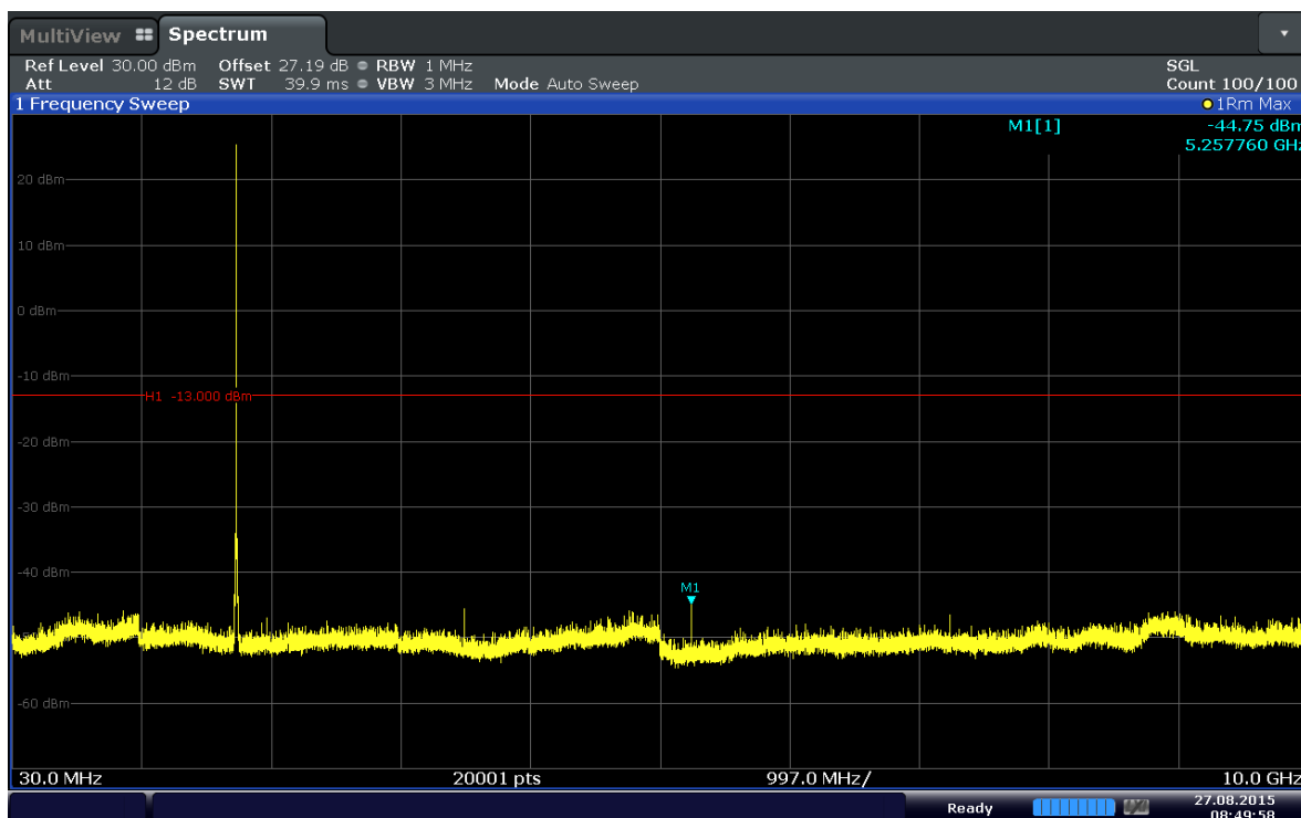
Plot 6-39. Conducted Spurious Plot (Band 4–5MHz–QPSK–RB Size 1–RB Offset 12–Ch.20375)
