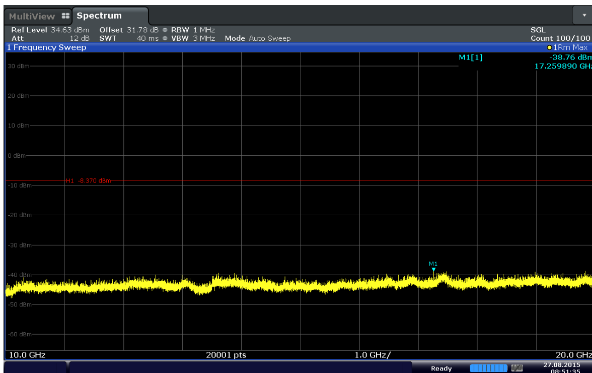
Plot 6-42. Conducted Spurious Plot (Band 4–10MHz–QPSK–RB Size 1–RB Offset 0–Ch.20000)
