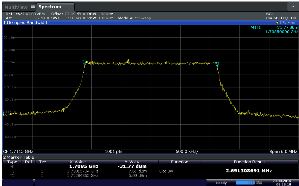
Plot 6-7. Occupied Bandwidth Plot (Band 4 – 3MHz QPSK - RB Size 15)
