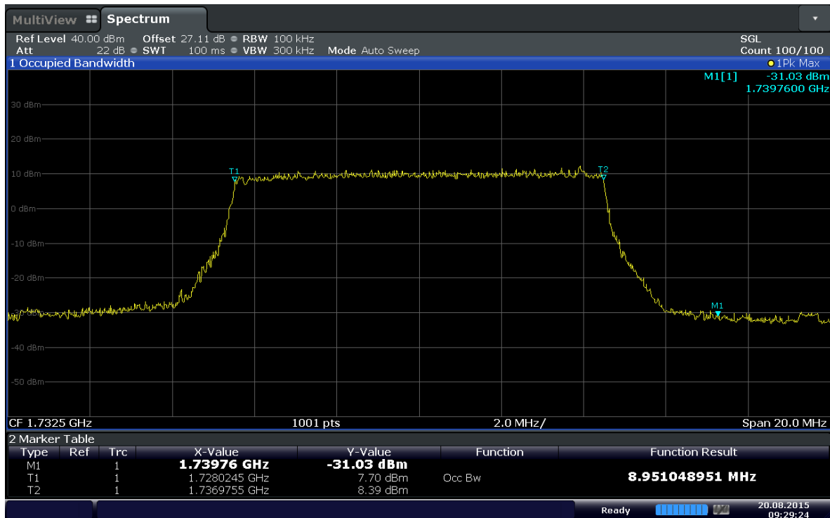
Plot 6-11. Occupied Bandwidth Plot (Band 4 – 10MHz QPSK - RB Size 50)
