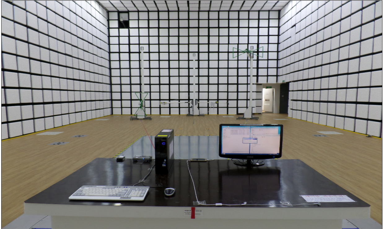
[ Radiated Disturbance for Below 1 GHz – Front ]
