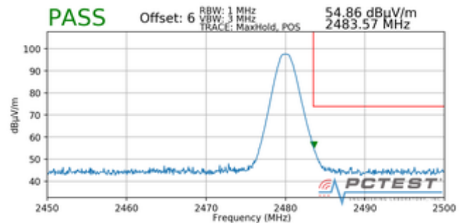
Plot 7-19. Radiated Restricted Upper Band Edge Measurement (Peak)
