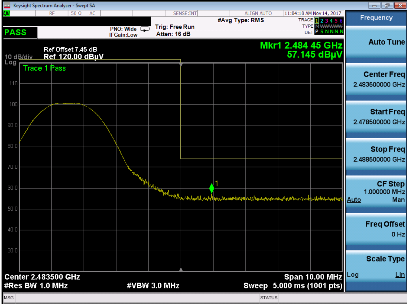
Plot 7-2. Radiated Restricted Upper Band Edge Measurement (Peak)
