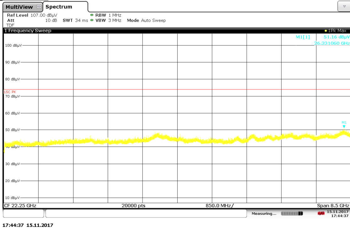
Plot 7-7. Radiated Spurious Plot above 18GHz (Pol. H)
