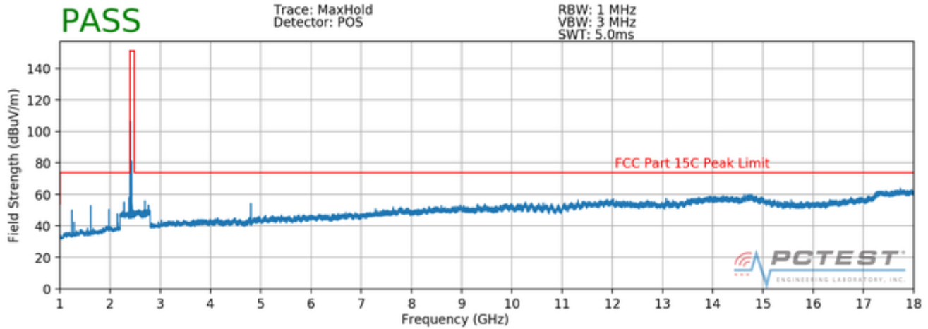
Plot 7-1. Radiated Spurious Plot above 1GHz (BT – Ch. 0, Ant. Pol. H)
