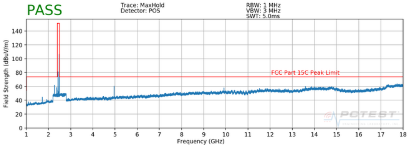
Plot 7-5. Radiated Spurious Plot above 1GHz (BT – Ch. 78, Ant. Pol. H)
