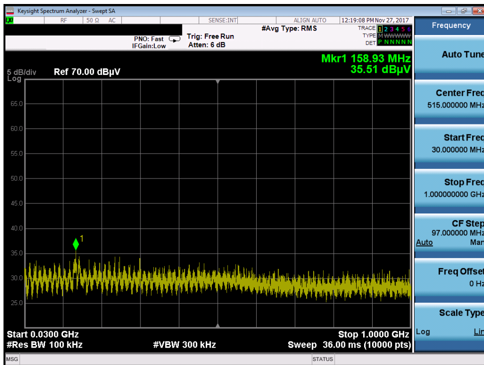
Plot 7-12. Radiated Spurious Plot below 1GHz (Pol. V)
