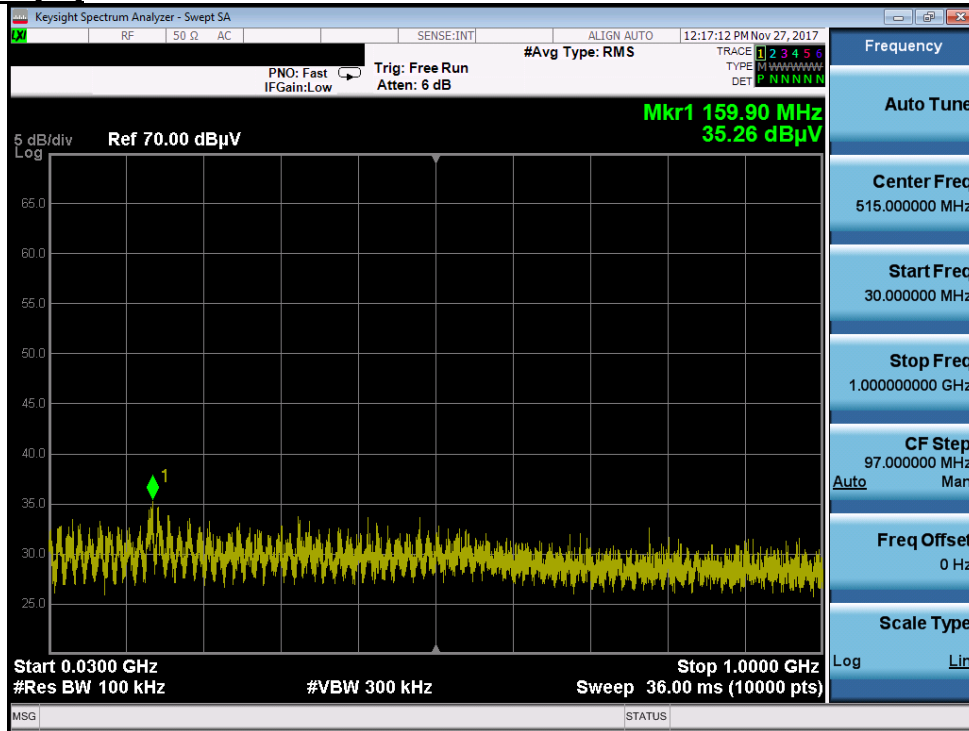
Plot 7-11. Radiated Spurious Plot below 1GHz (Pol. H)
