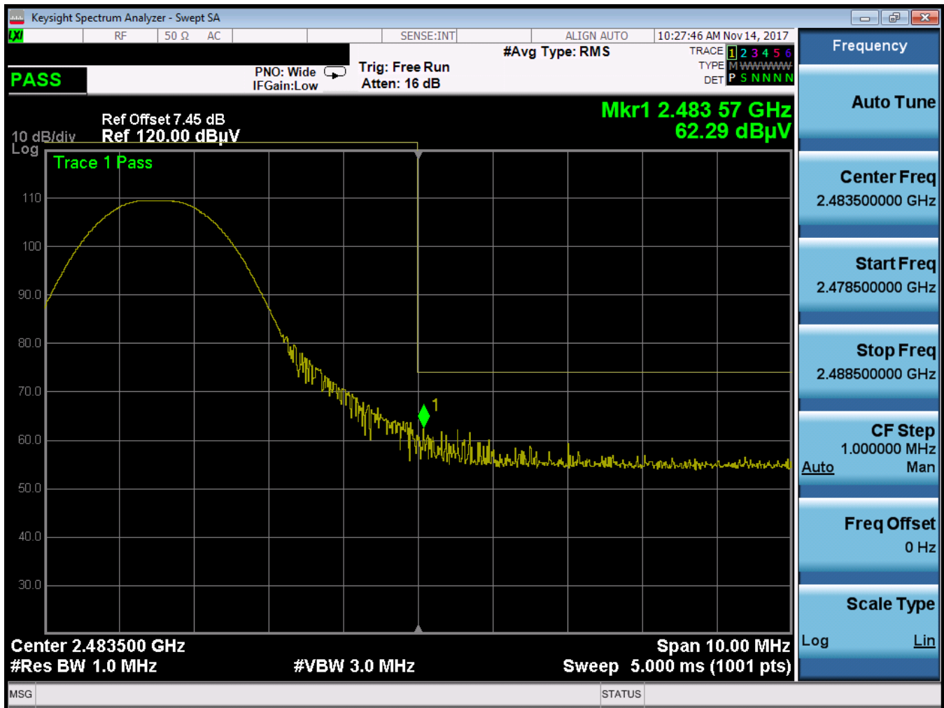
Plot 7-10. Radiated Restricted Upper Band Edge Measurement (Peak)
