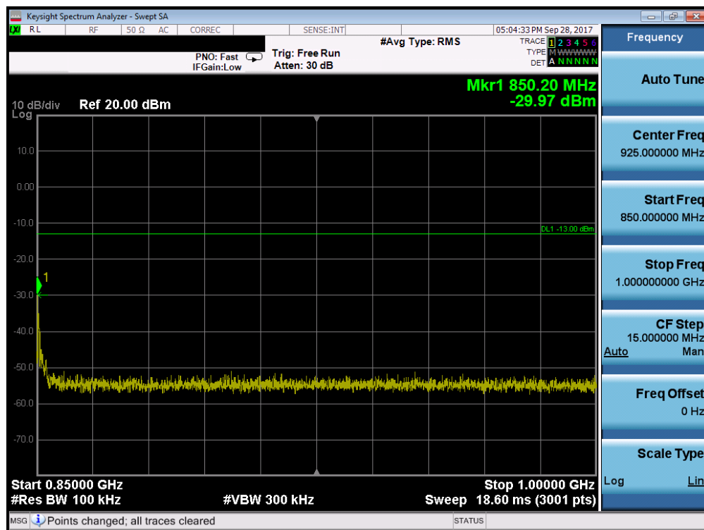
Plot 7-11. Conducted Spurious Plot (Cellular GPRS Mode - High Channel)
