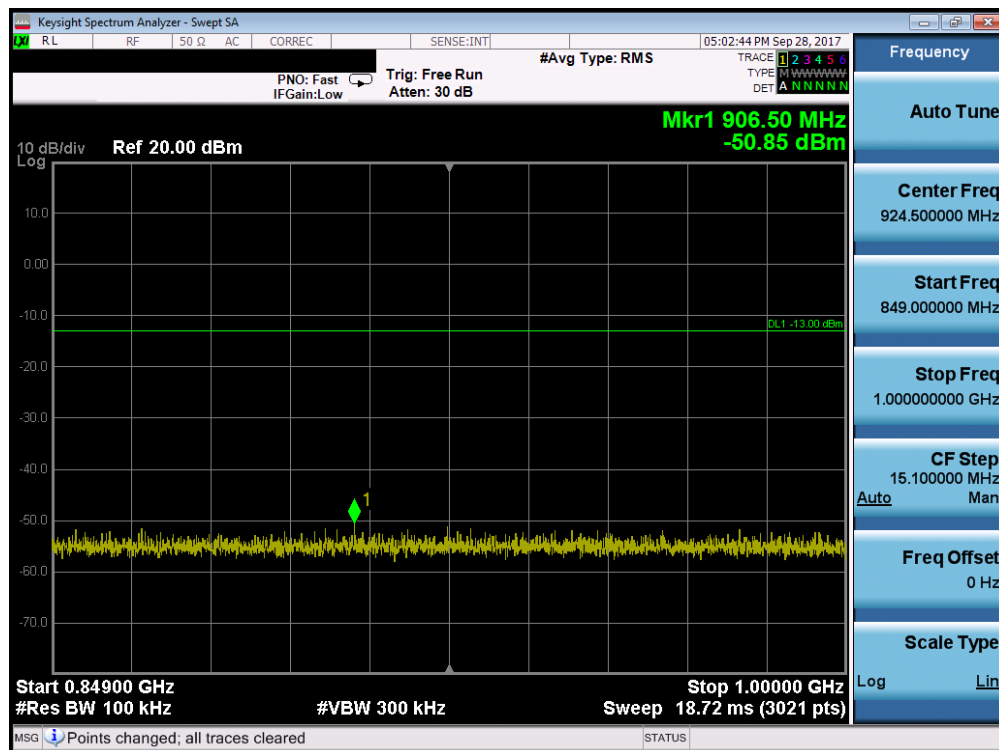
Plot 7-5. Conducted Spurious Plot (Cellular GPRS Mode - Low Channel)
