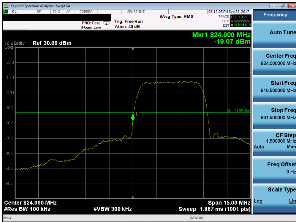
Plot 7-24. Band Edge Plot (Cellular WCDMA Mode - Low Channel)
