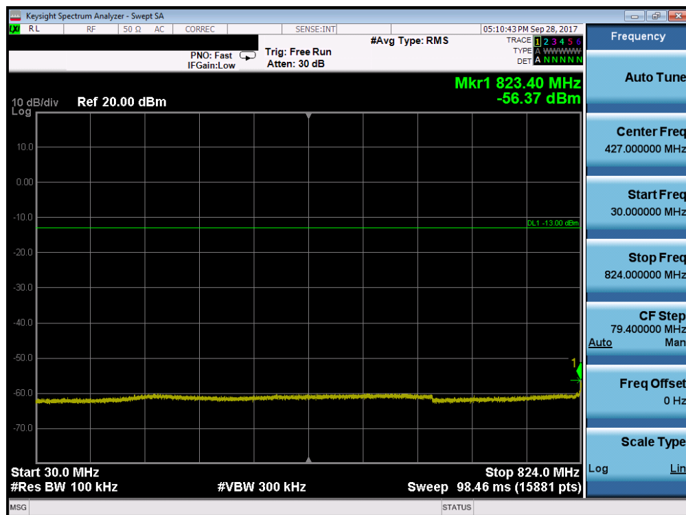
Plot 7-16. Conducted Spurious Plot (Cellular WCDMA Mode - Mid Channel)
