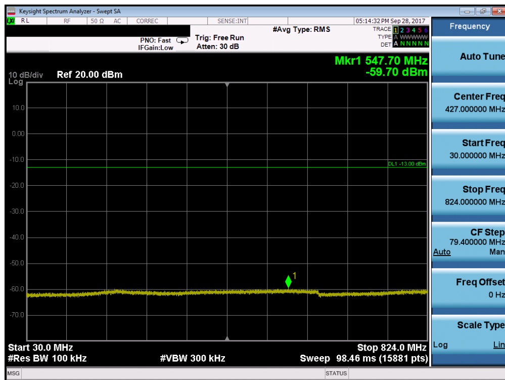
Plot 7-19. Conducted Spurious Plot (Cellular WCDMA Mode - High Channel)
