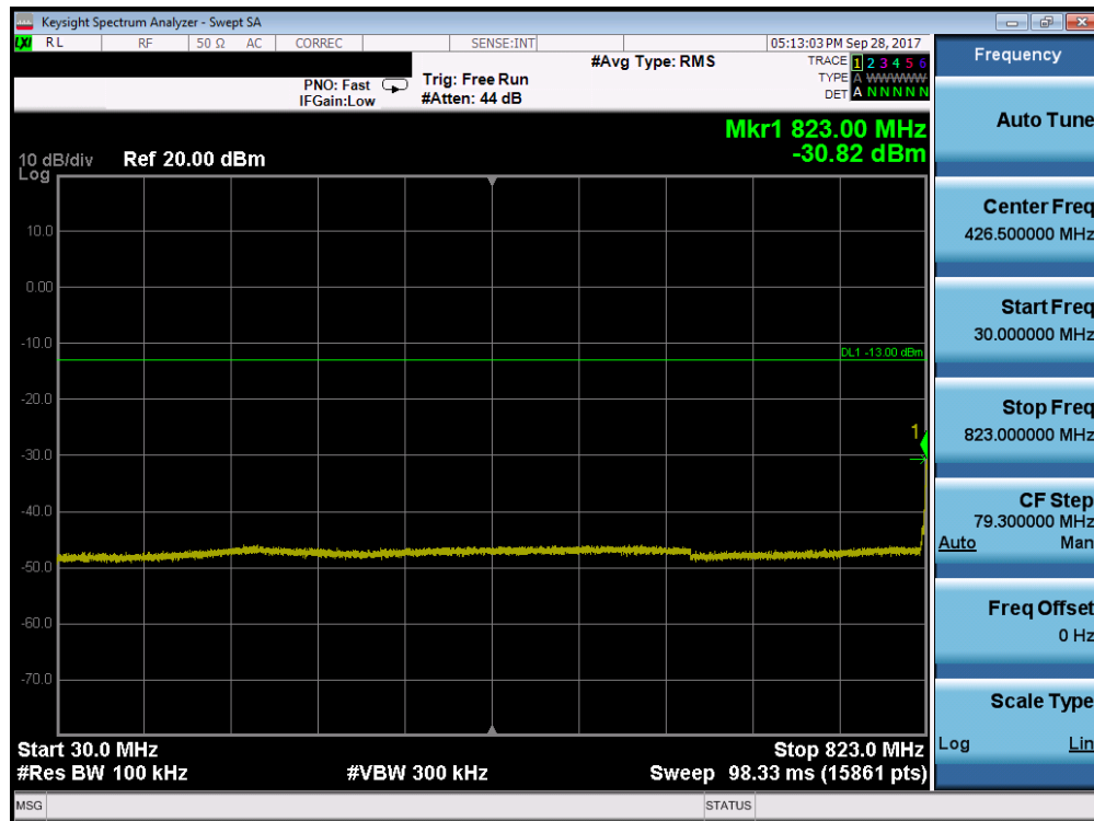
Plot 7-13. Conducted Spurious Plot (Cellular WCDMA Mode - Low Channel)
