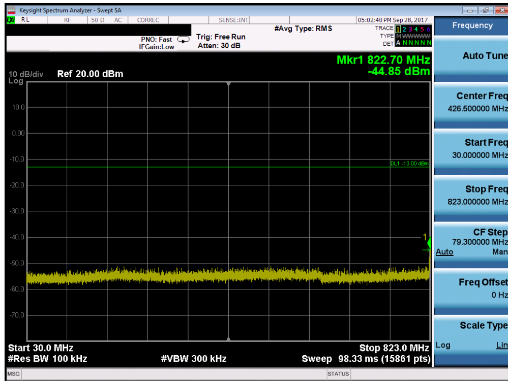
Plot 7-4. Conducted Spurious Plot (Cellular GPRS Mode - Low Channel)
