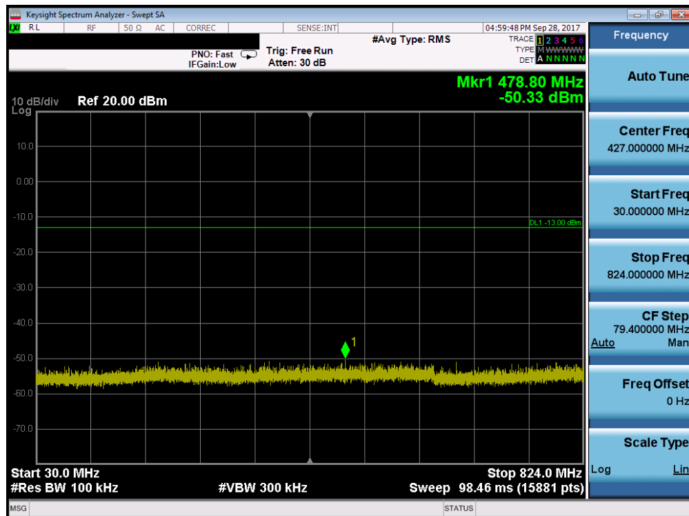
Plot 7-7. Conducted Spurious Plot (Cellular GPRS Mode - Mid Channel)
