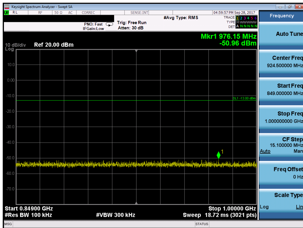
Plot 7-8. Conducted Spurious Plot (Cellular GPRS Mode - Mid Channel)
