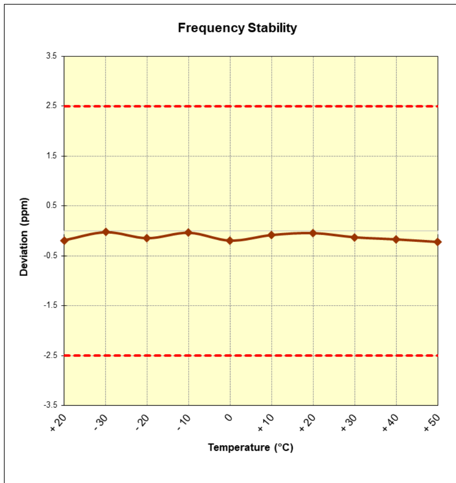
Frequency Stability Graph (Cellular WCDMA Mode – Ch. 4183)
