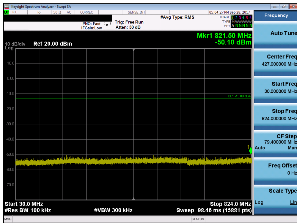
Plot 7-10. Conducted Spurious Plot (Cellular GPRS Mode - High Channel)
