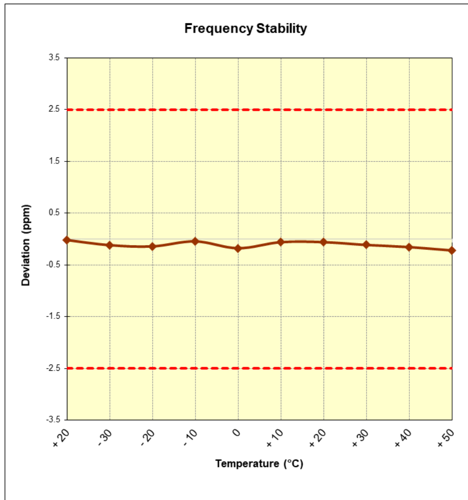
Figure 7-7. Frequency Stability Graph (Cellular GPRS Mode – Ch. 190)
