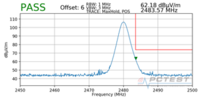
Plot 7-51. Radiated Restricted Upper Band Edge Measurement (Peak)
