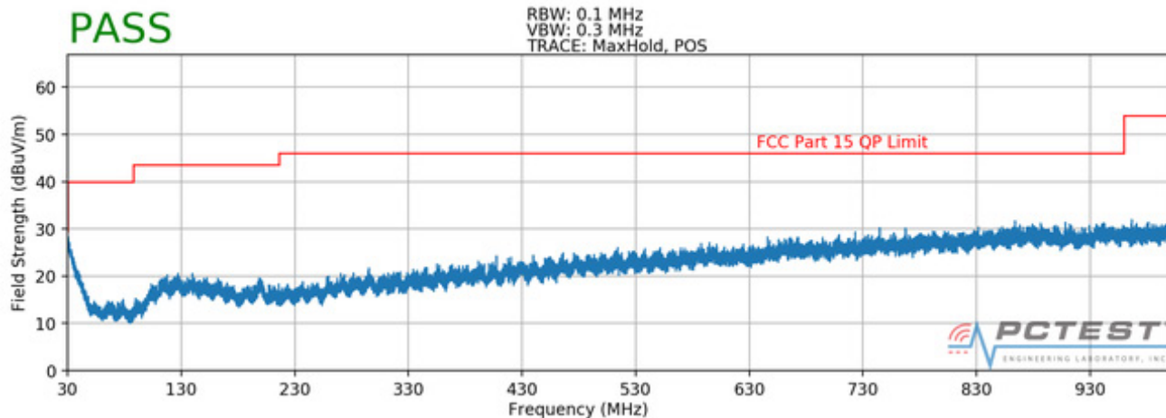
Plot 7-43. Radiated Spurious Plot below 1GHz (Pol. V)
