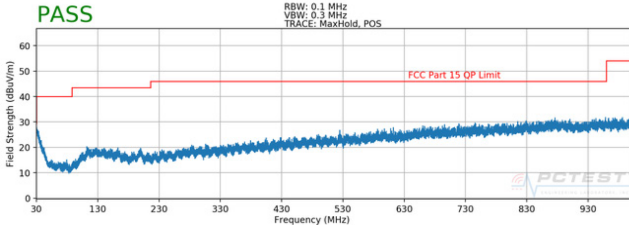
Plot 7-42. Radiated Spurious Plot below 1GHz (Pol. H)
