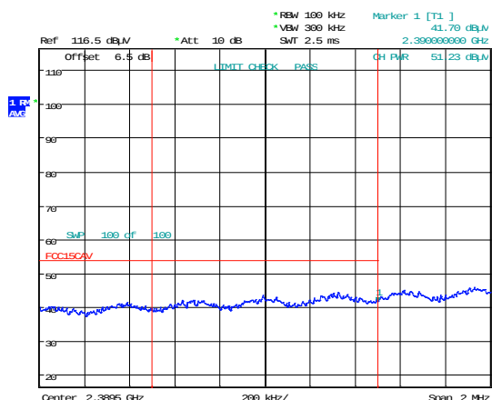
Plot 7-39. Radiated Restricted Lower Band Edge Measurement (Average)
