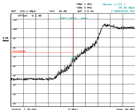
Plot 7-40. Radiated Restricted Lower Band Edge Measurement (Peak)
