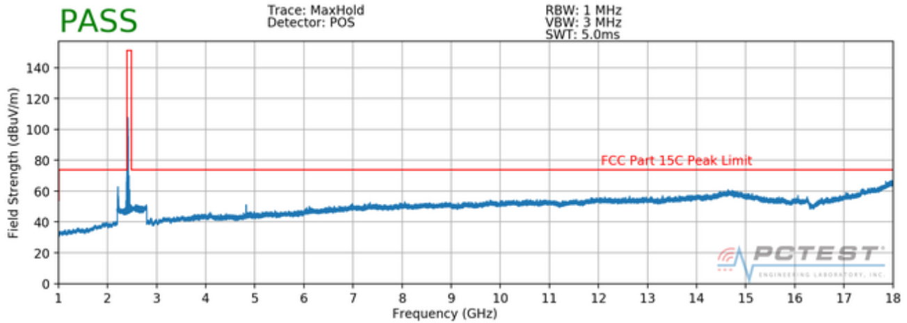
Plot 7-5. Radiated Spurious Plot above 1GHz (802.11b – Ch. 1, Ant. Pol. H)
