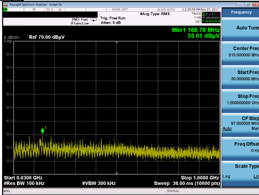
Plot 7-13. Radiated Spurious Plot below 1GHz (Pol. H)
