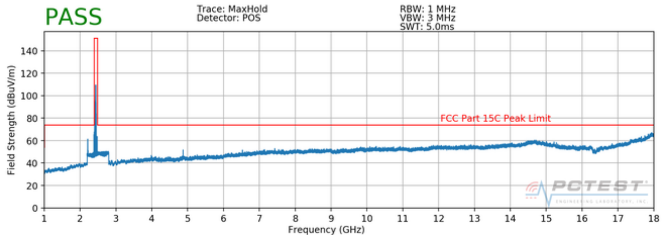
Plot 7-7. Radiated Spurious Plot above 1GHz (802.11b – Ch. 6, Ant. Pol. H)
