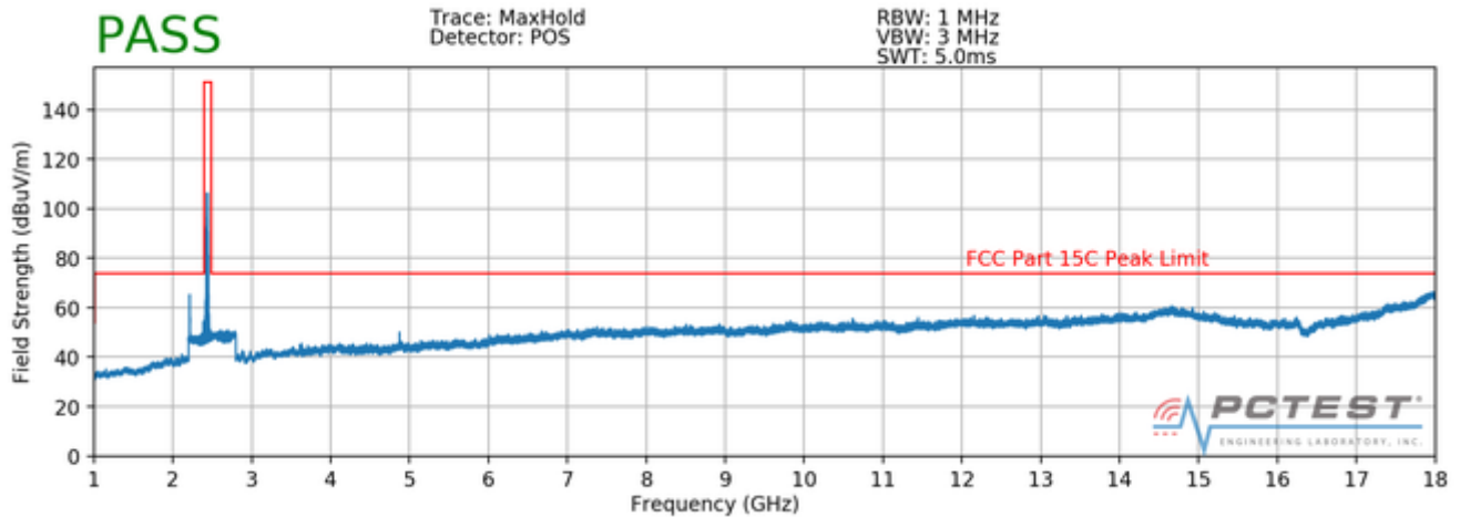
Plot 7-8. Radiated Spurious Plot above 1GHz (802.11b – Ch. 6, Ant. Pol. V)
