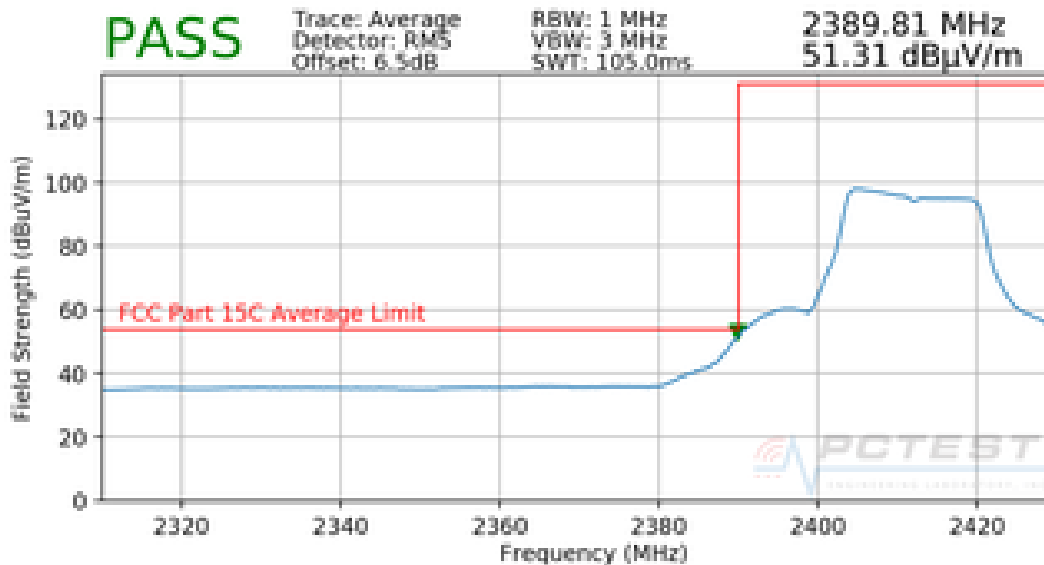
Plot 7-1. Radiated Restricted Lower Band Edge Measurement (Average)
