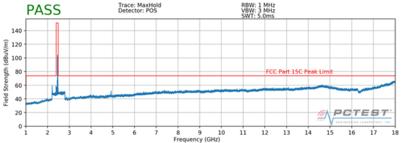
Plot 7-10. Radiated Spurious Plot above 1GHz (802.11b – Ch. 11, Ant. Pol. V)
