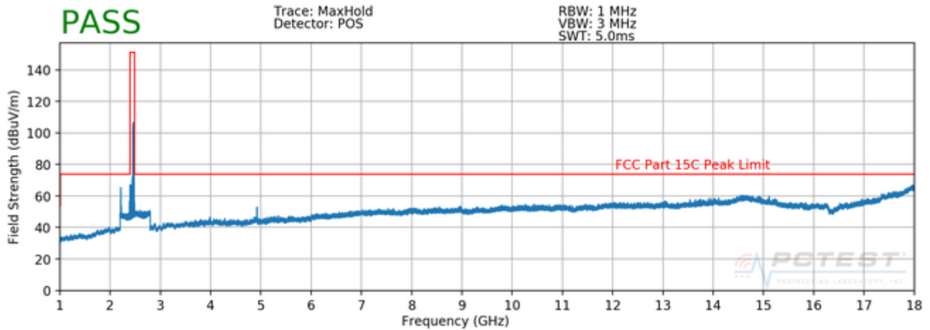
Plot 7-9. Radiated Spurious Plot above 1GHz (802.11b – Ch. 11, Ant. Pol. H)
