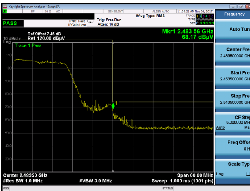
Plot 7-4. Radiated Restricted Upper Band Edge Measurement (Peak)
