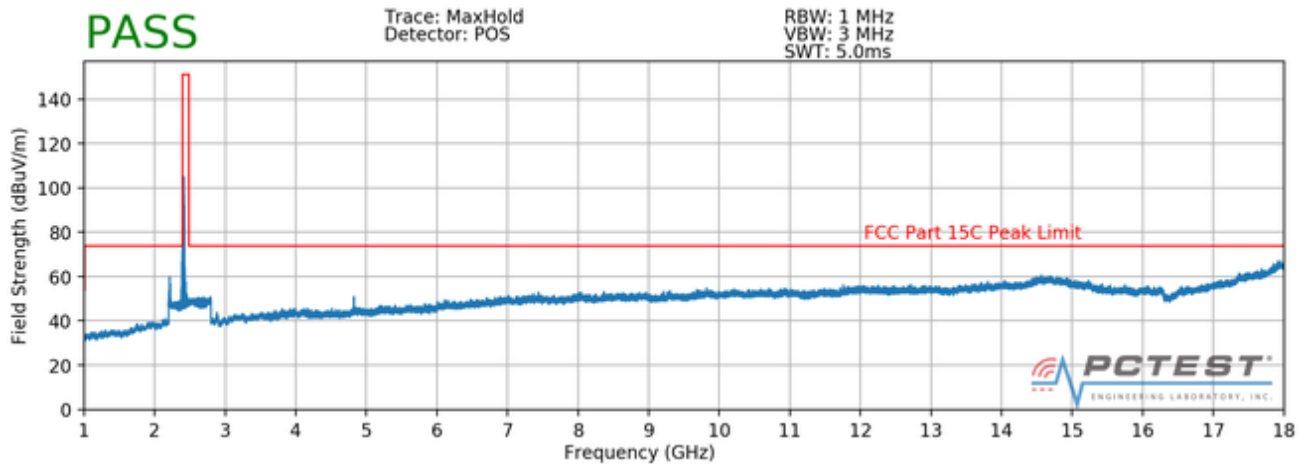
Plot 7-6. Radiated Spurious Plot above 1GHz (802.11b – Ch. 1, Ant. Pol. V)
