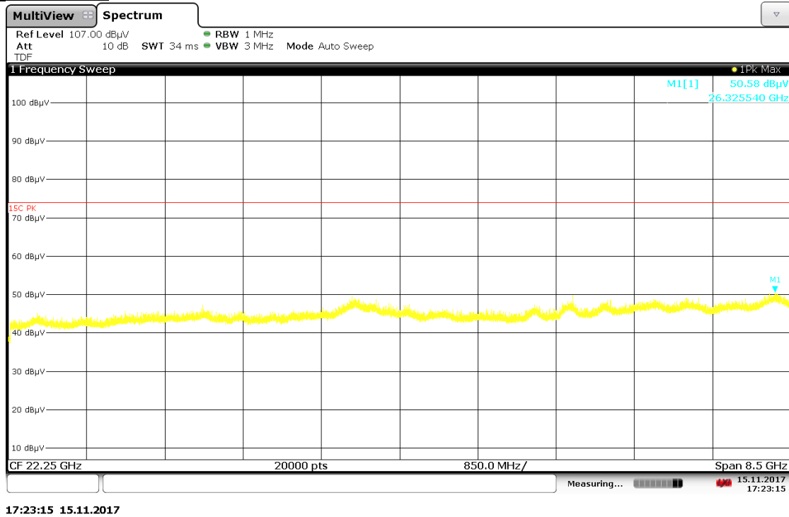
Plot 7-11. Radiated Spurious Plot above 18GHz (Pol. H)
