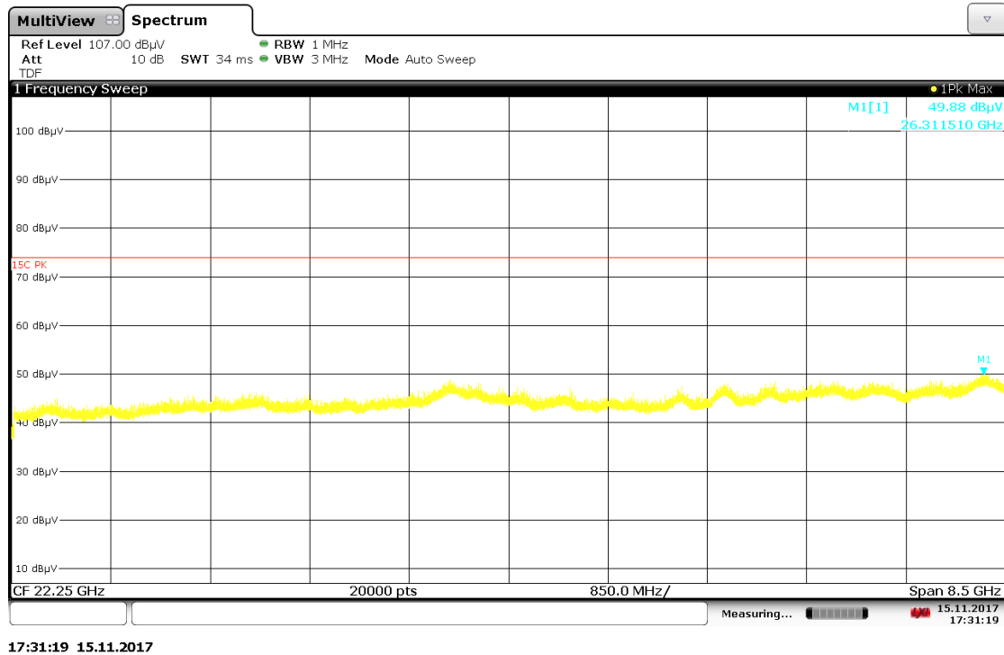
Plot 7-12. Radiated Spurious Plot above 18GHz (Pol. V)
