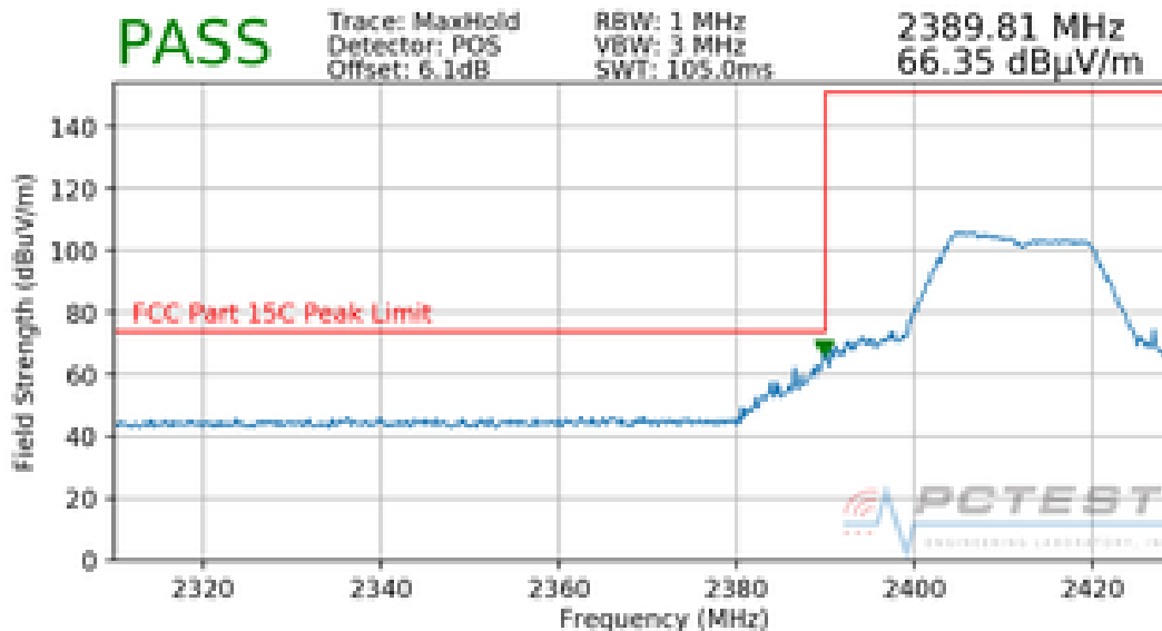
Plot 7-2. Radiated Restricted Lower Band Edge Measurement (Peak)
