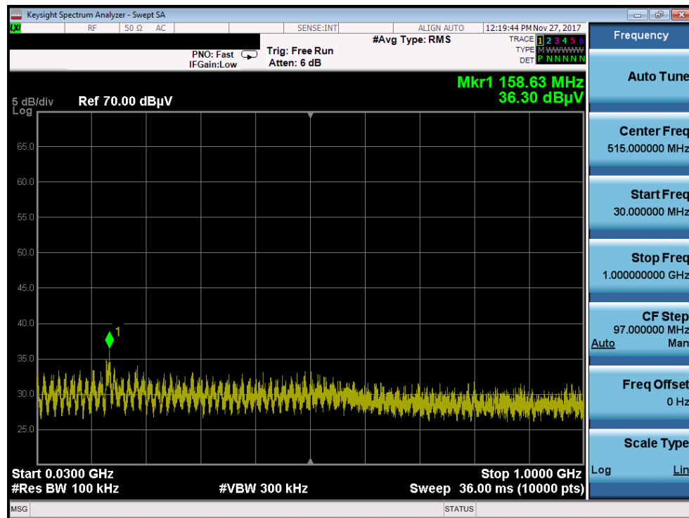
Plot 7-14. Radiated Spurious Plot below 1GHz (Pol. V)
