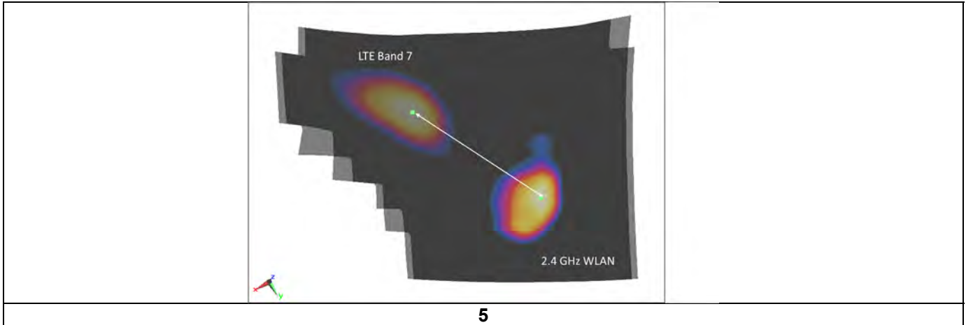
5 Table 12-11 Head SAR to Peak Locations Separation Ratio Plots
