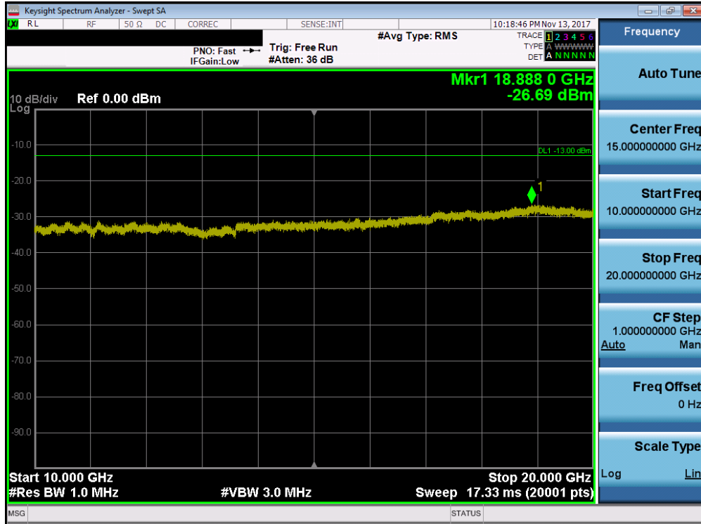
Plot 7-82. Conducted Spurious Plot (Band 66/4 - 15.0MHz QPSK - RB Size 1, RB Offset 0 - High Channel)
