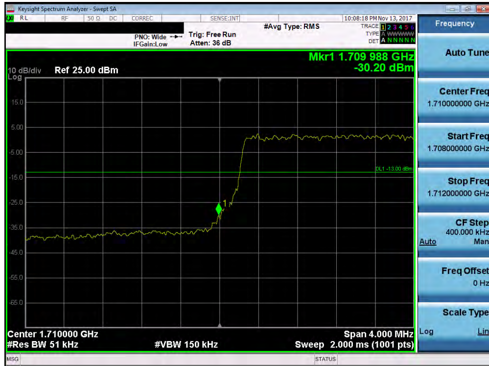
Plot 7-137. Lower Band Edge Plot (Band 66/4 - 5.0MHz QPSK - Full RB Configuration)
