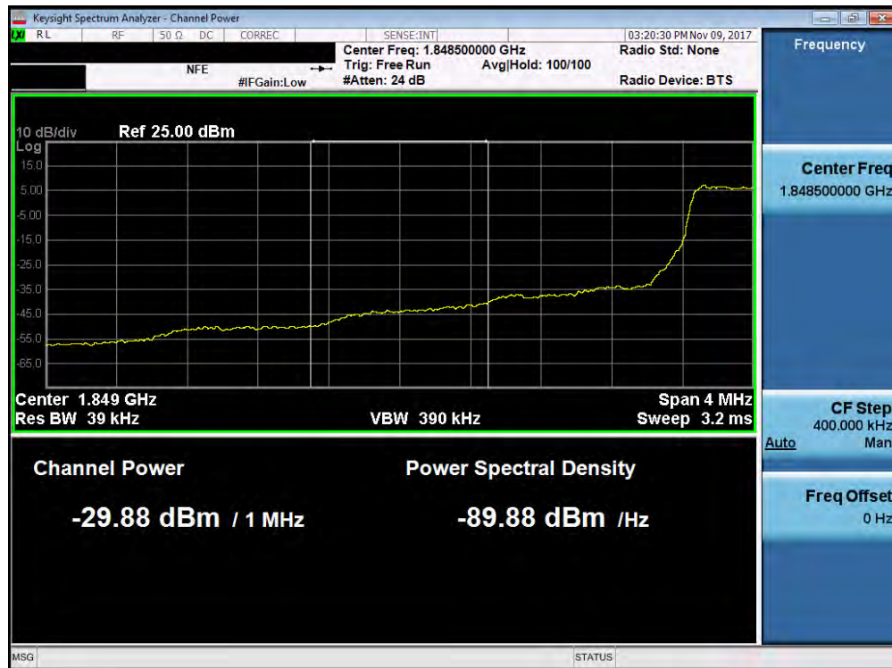
Plot 7-162. . Lower Extended Band Edge Plot (Band 2 - 1.4MHz QPSK - Full RB Configuration)
