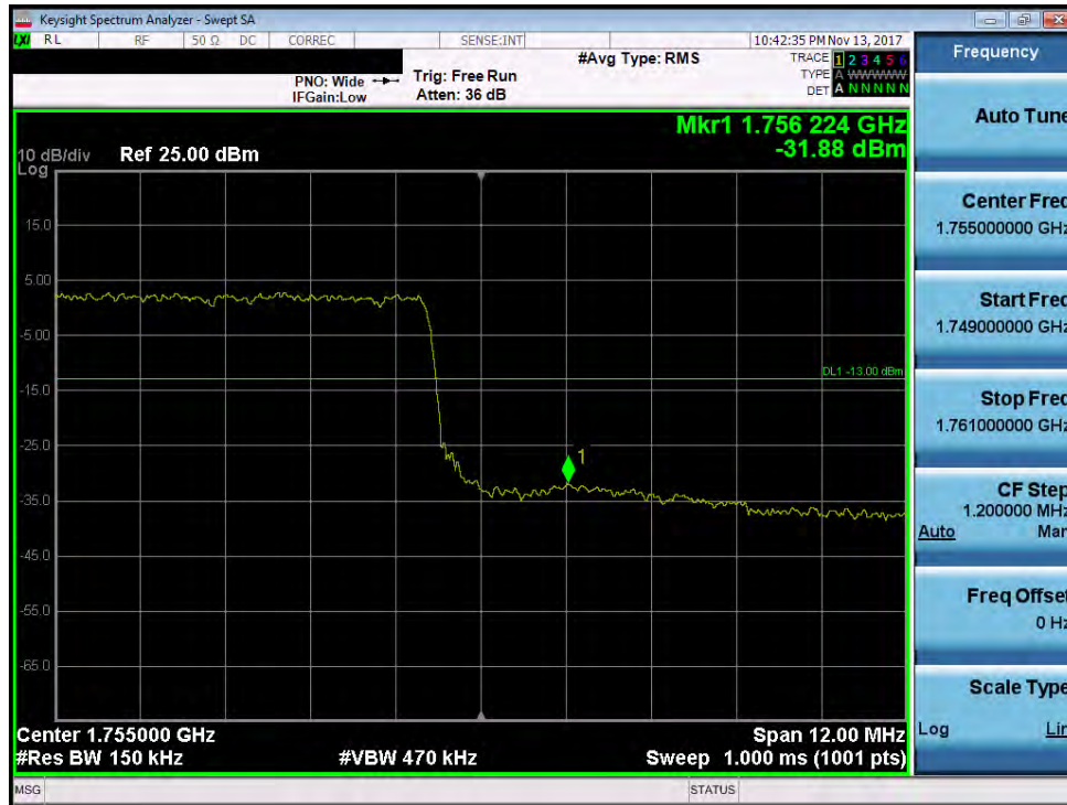
Plot 7-153. Upper Band Edge Plot (Band 4 - 15.0MHz QPSK - Full RB Configuration)
