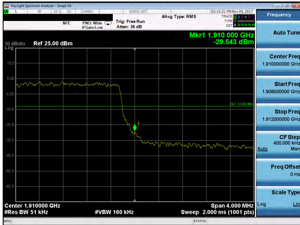
Plot 7-171. Upper Band Edge Plot (Band 2 - 5.0MHz QPSK - Full RB Configuration)
