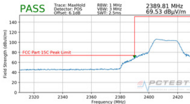
Plot 7-40. Radiated Restricted Lower Band Edge Measurement (Peak)
