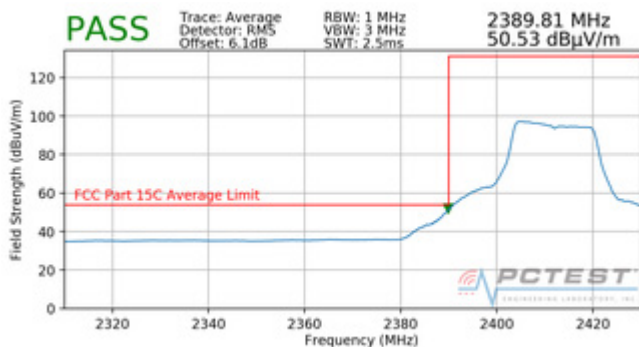
Plot 7-39. Radiated Restricted Lower Band Edge Measurement (Average)
