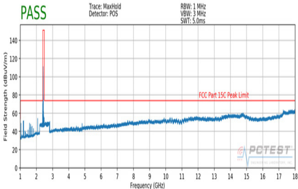
Plot 7-31. Radiated Spurious Plot above 1GHz (802.11b – Ch. 1, Ant. Pol. H)
