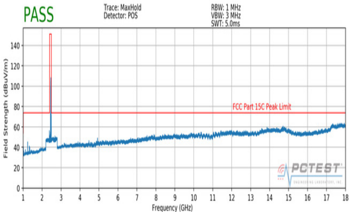
Plot 7-36. Radiated Spurious Plot above 1GHz (802.11b – Ch. 11, Ant. Pol. V)
