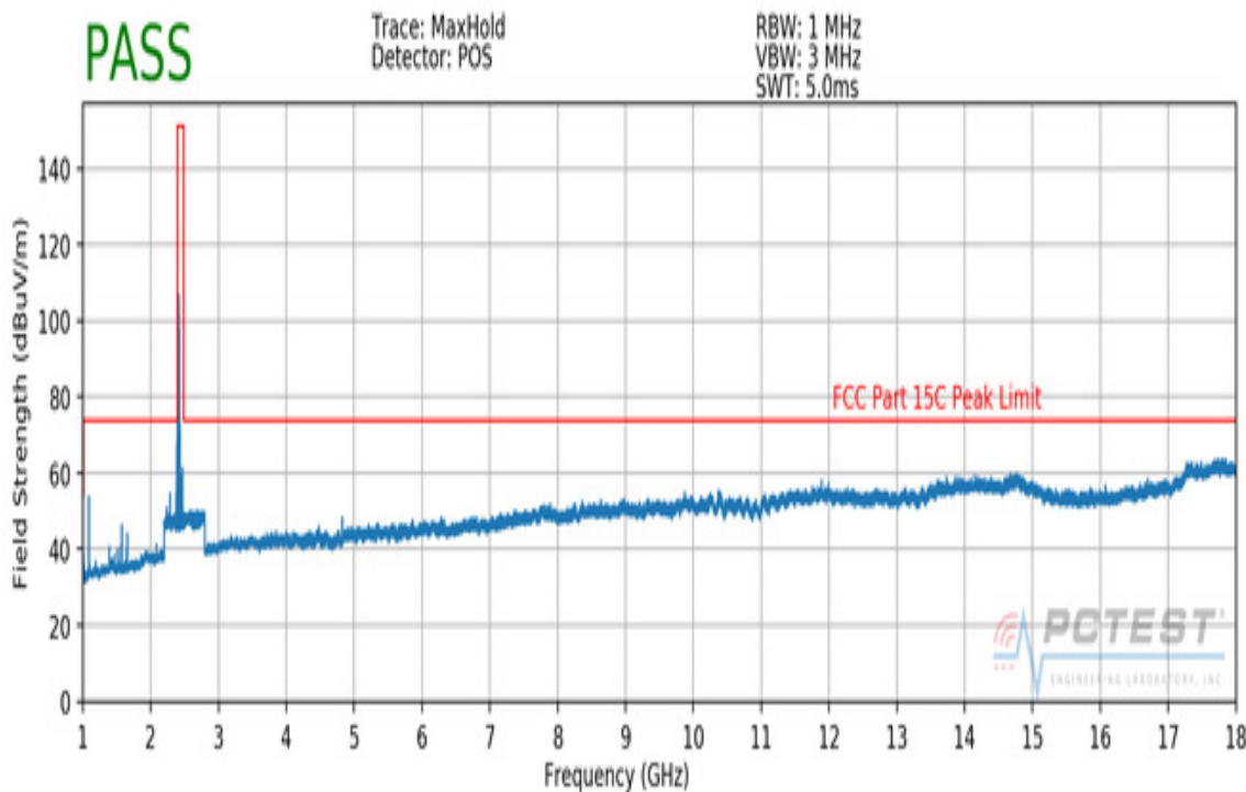
Plot 7-32. Radiated Spurious Plot above 1GHz (802.11b – Ch. 1, Ant. Pol. V)
