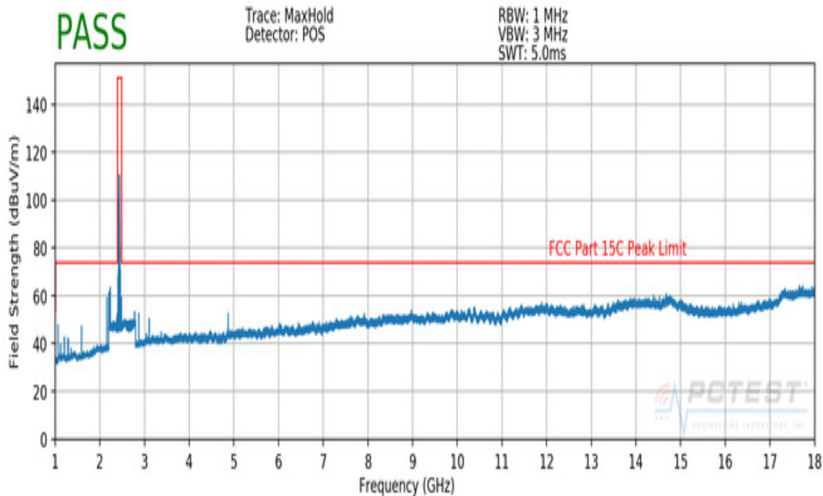
Plot 7-33. Radiated Spurious Plot above 1GHz (802.11b – Ch. 6, Ant. Pol. H)
