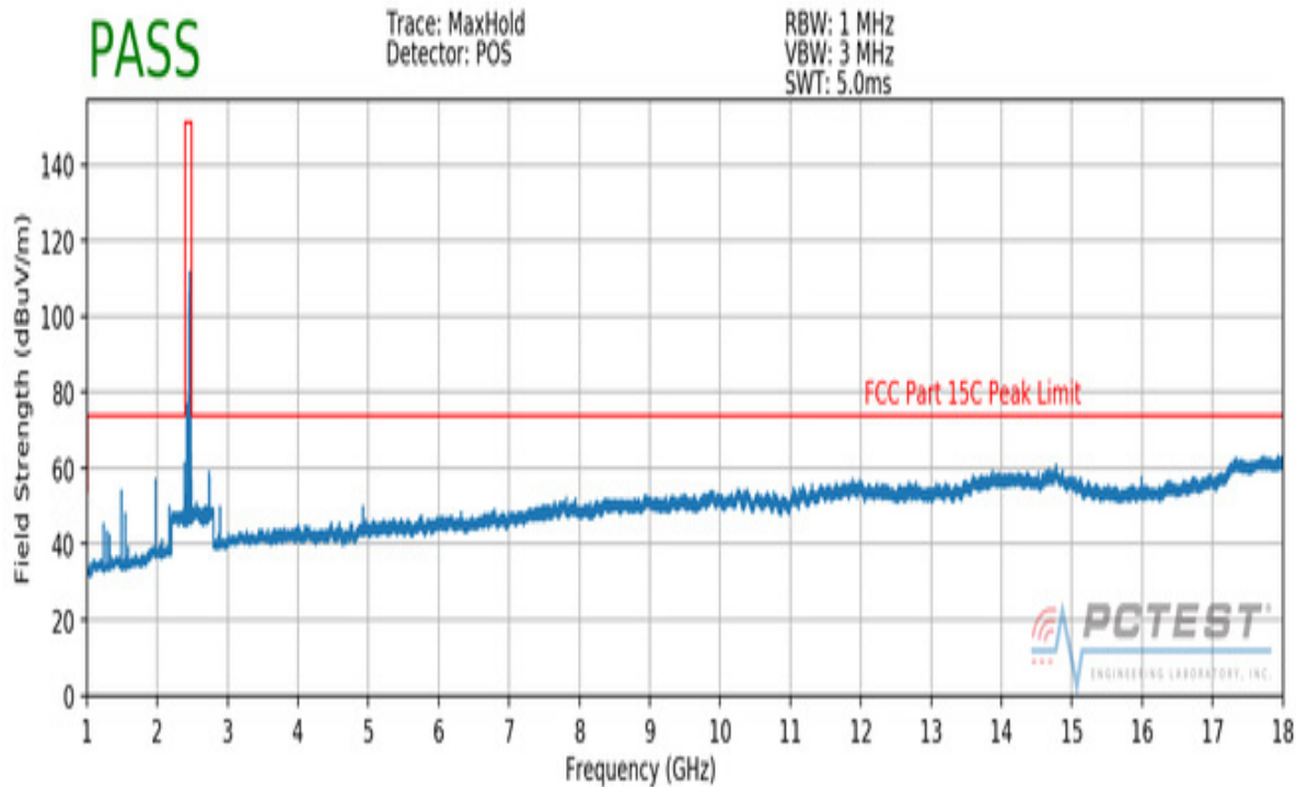
Plot 7-35. Radiated Spurious Plot above 1GHz (802.11b – Ch. 11, Ant. Pol. H)
