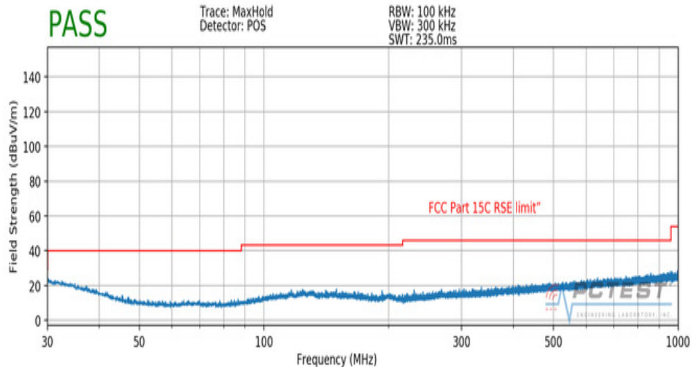
Plot 7-43. Radiated Spurious Plot below 1GHz (Pol. H)
