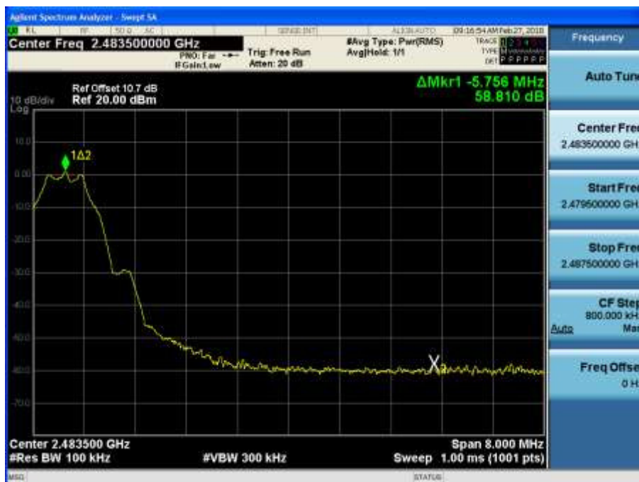
BandEdge (High-CH 39)
