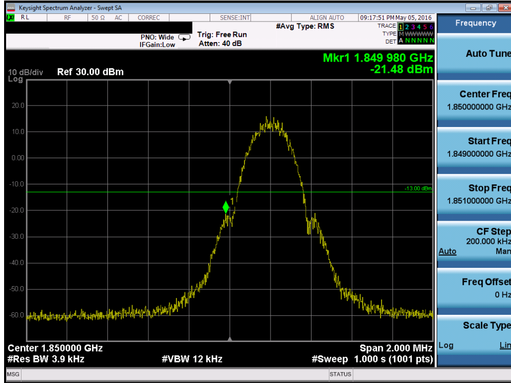
Plot 7-42. Band Edge Plot (PCS GPRS Mode – Ch. 512)
