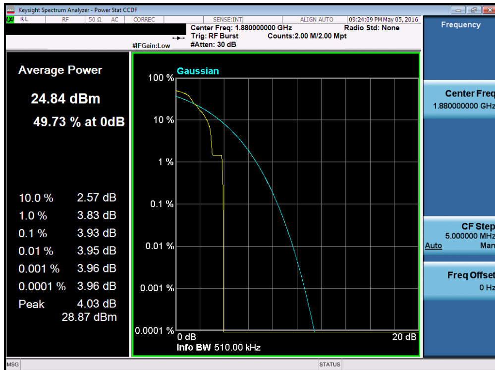
Plot 7-57. Peak-Average Ratio Plot (EDGE1900 Mode – Ch. 661)
