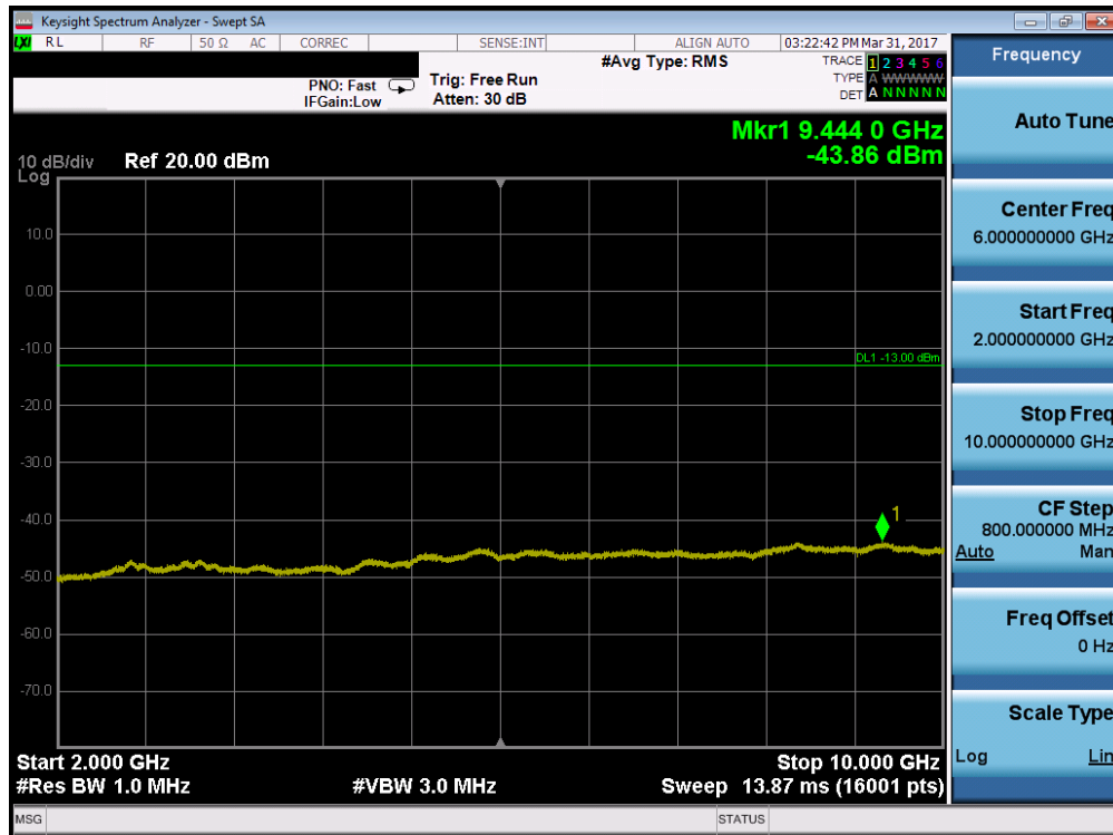
Plot 7-17. Conducted Spurious Plot (Cellular CDMA Mode – Ch. 1013)
