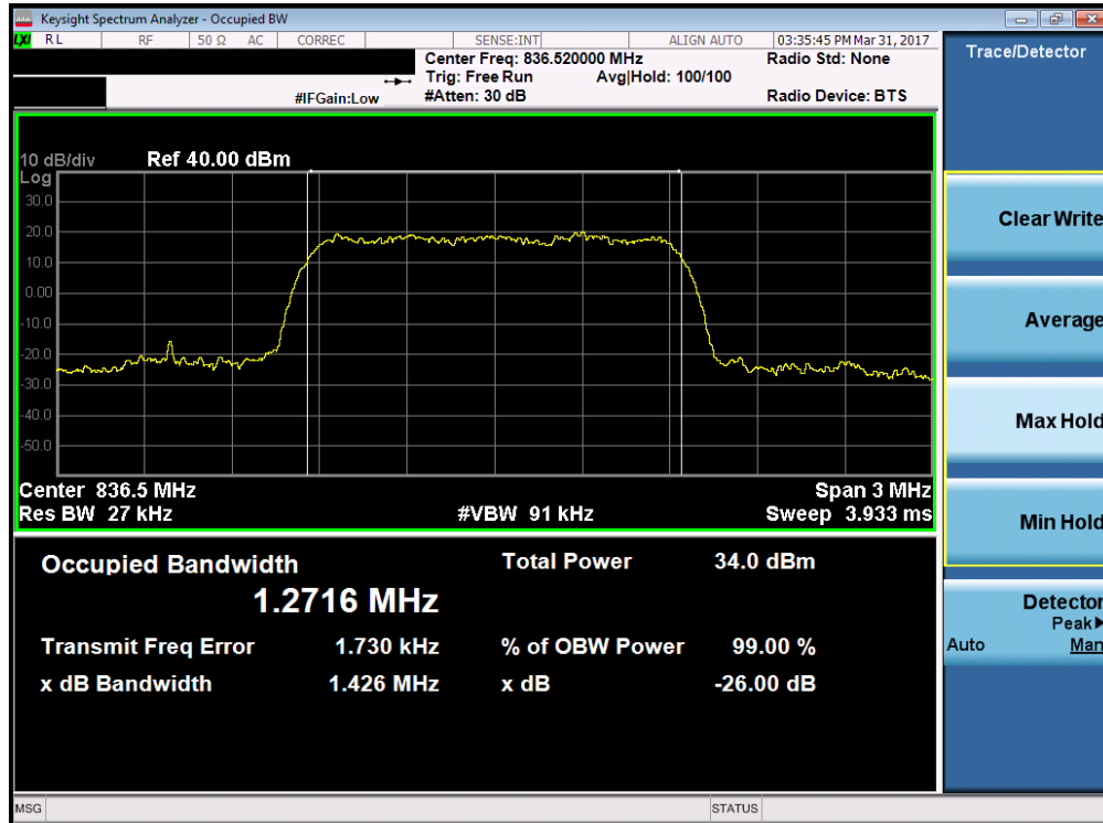
Plot 7-3. Occupied Bandwidth Plot (Cellular CDMA Mode – Ch. 384)
