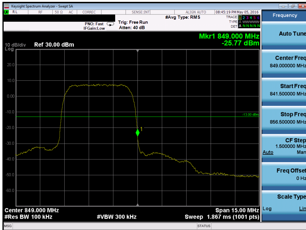
Plot 7-51. Band Edge Plot (Cellular WCDMA Mode – Ch. 4233)
