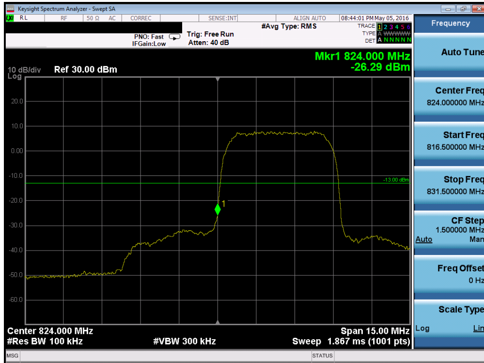
Plot 7-50. Band Edge Plot (Cellular WCDMA Mode – Ch. 4132)
