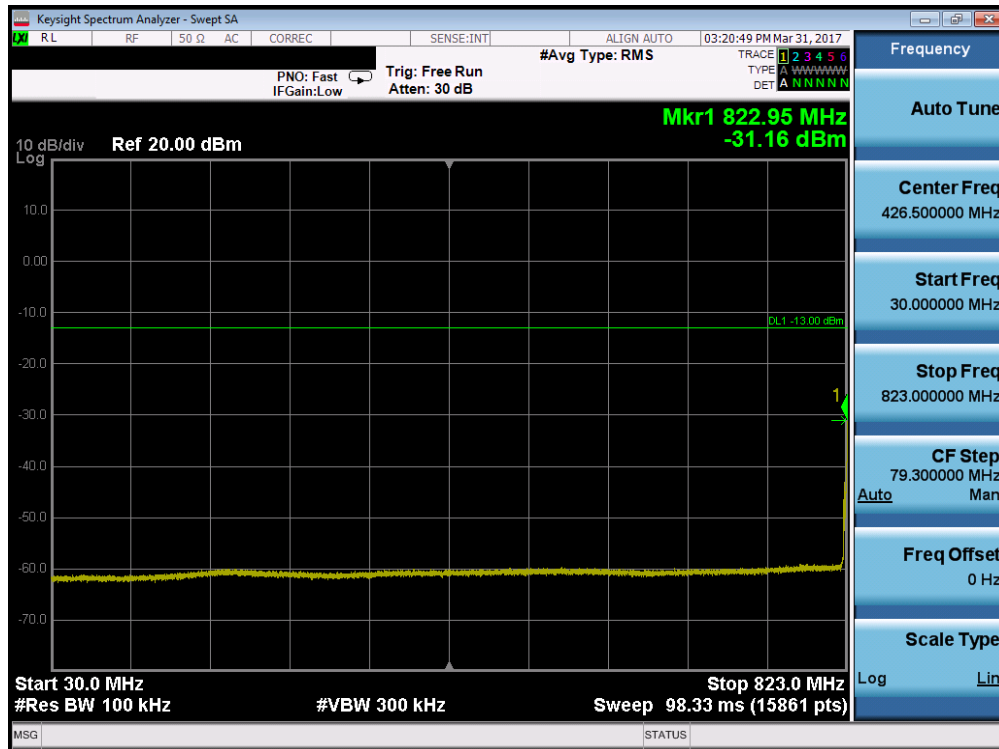
Plot 7-15. Conducted Spurious Plot (Cellular CDMA Mode – Ch. 1013)
