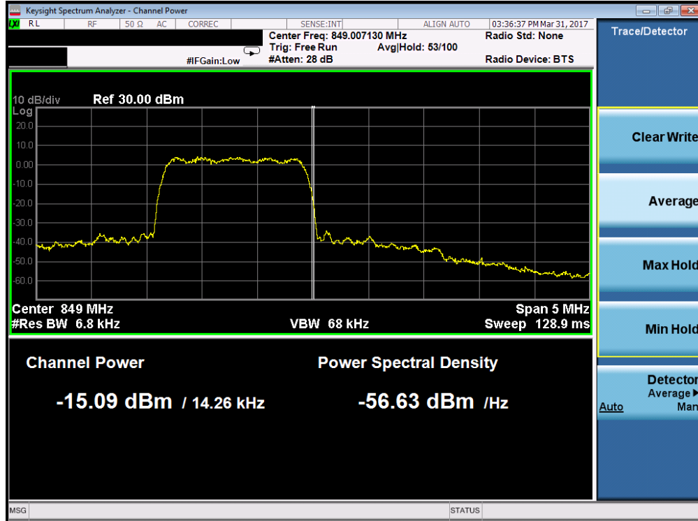
Plot 7-48. Band Edge Plot (Cellular CDMA Mode – Ch. 777)
