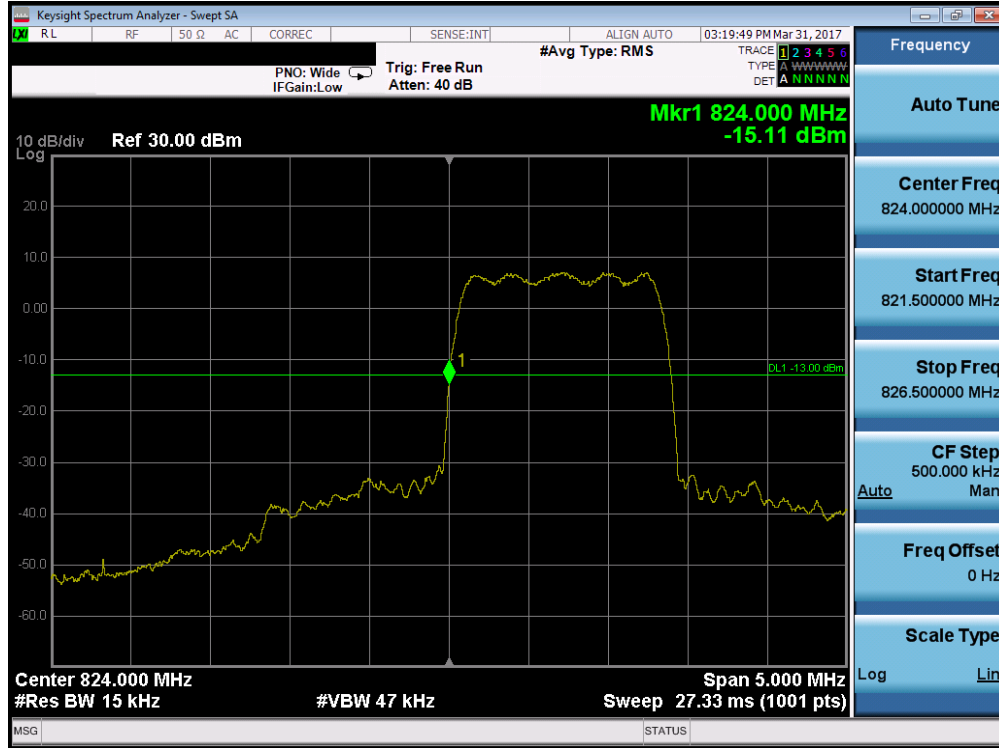
Plot 7-46. Band Edge Plot (Cellular CDMA Mode – Ch. 1013)
