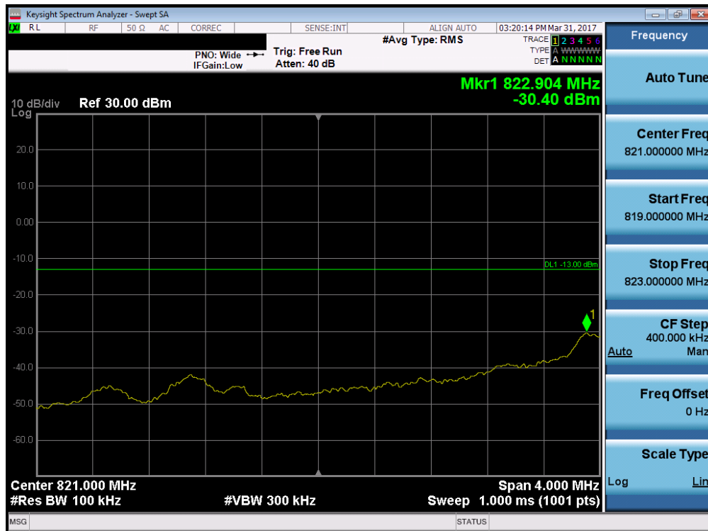
Plot 7-47. 4MHz Span Plot (Cellular CDMA Mode – Ch. 1013)
