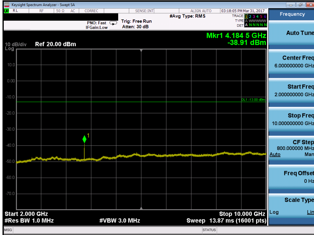
Plot 7-20. Conducted Spurious Plot (Cellular CDMA Mode – Ch. 384)
