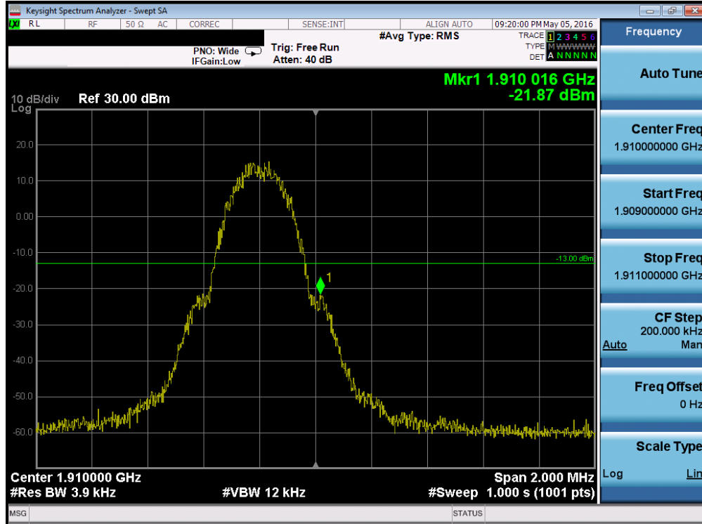
Plot 7-44. Band Edge Plot (PCS GPRS Mode – Ch. 810)
