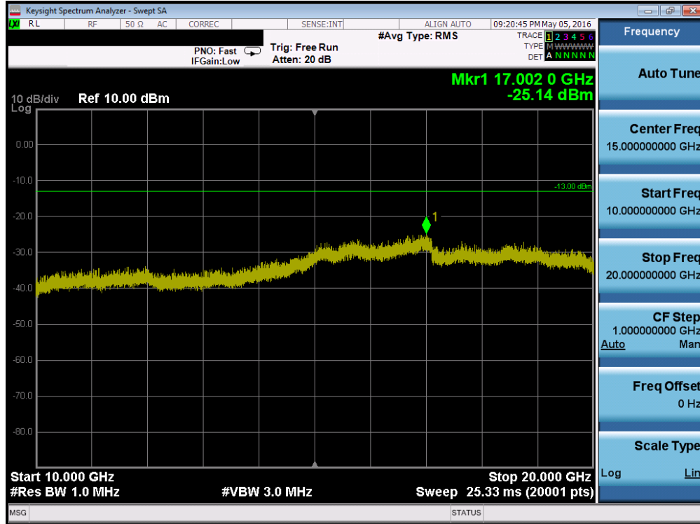
Plot 7-14. Conducted Spurious Plot (PCS GPRS Mode – Ch. 810)
