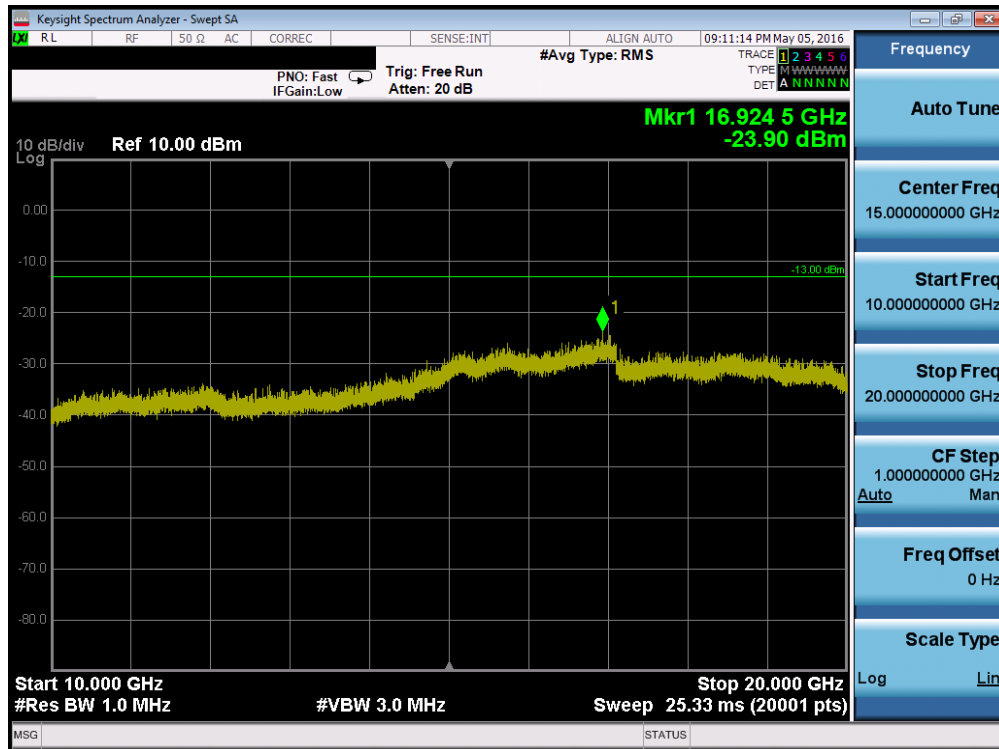
Plot 7-11. Conducted Spurious Plot (PCS GPRS Mode – Ch. 661)
