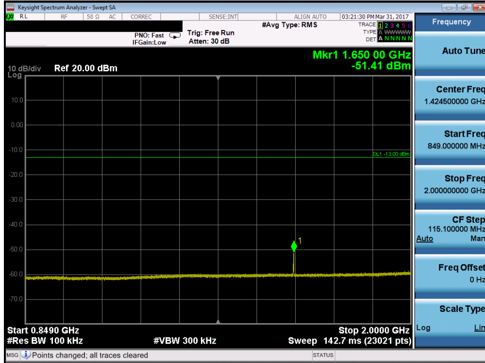
Plot 7-16. Conducted Spurious Plot (Cellular CDMA Mode – Ch. 1013)
