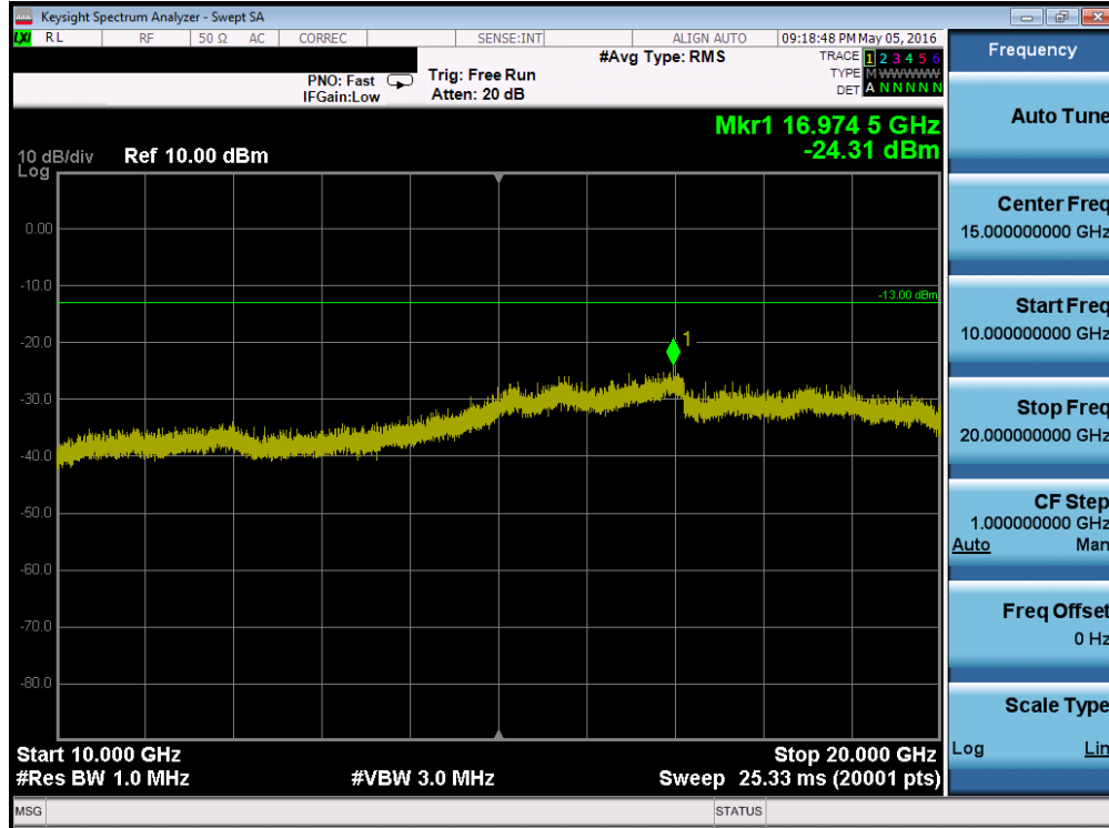
Plot 7-8. Conducted Spurious Plot (PCS GPRS Mode – Ch. 512)
