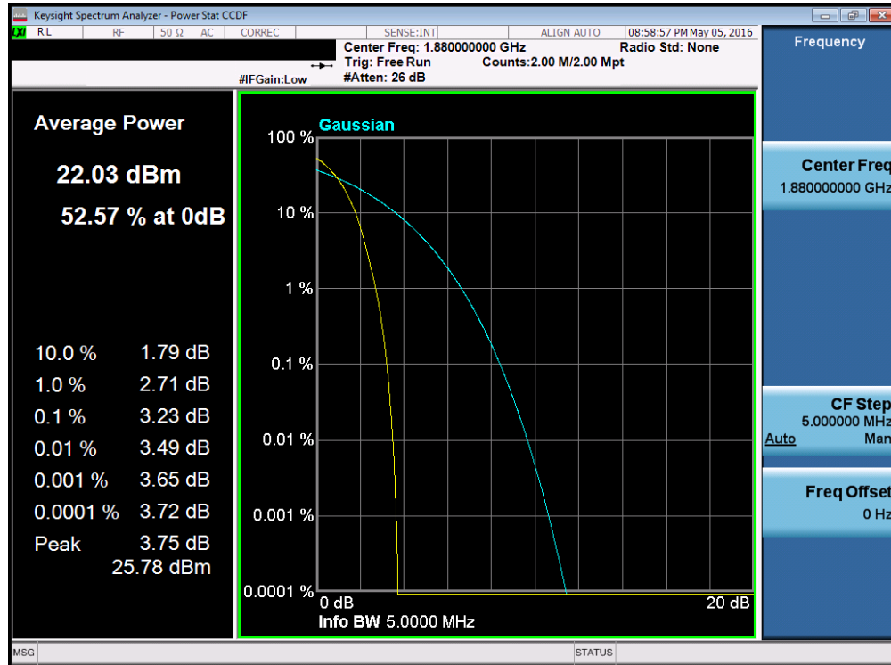
Plot 7-58. Peak-Average Ratio Plot (PCS WCDMA Mode – Ch. 9400)
