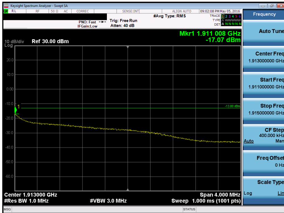
Plot 7-55. 4MHz Span Plot (PCS WCDMA Mode – Ch. 9538)
