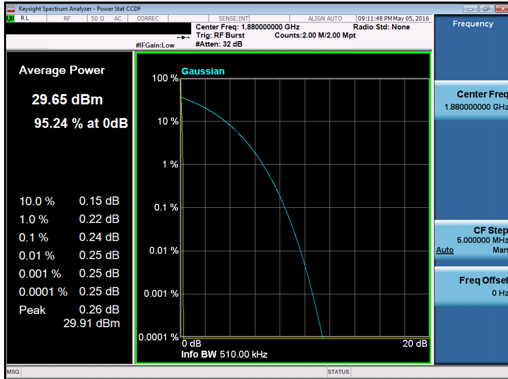
Plot 7-56. Peak-Average Ratio Plot (PCS GPRS Mode – Ch. 661)
