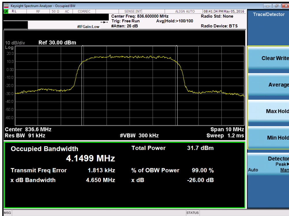
Plot 7-4. Occupied Bandwidth Plot (Cellular WCDMA Mode – Ch. 4183)
