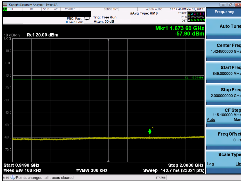
Plot 7-19. Conducted Spurious Plot (Cellular CDMA Mode – Ch. 384)
