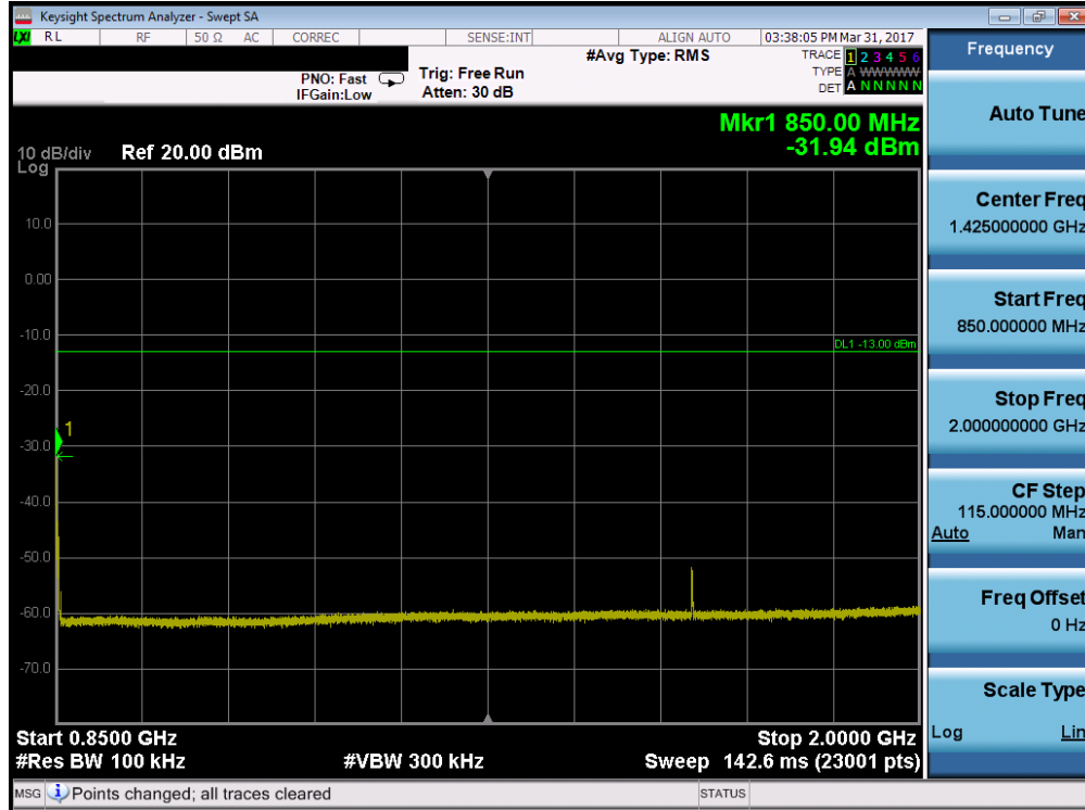
Plot 7-22. Conducted Spurious Plot (Cellular CDMA Mode – Ch. 777)
