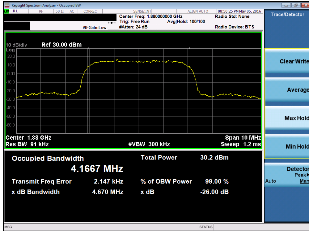
Plot 7-5. Occupied Bandwidth Plot (PCS WCDMA Mode – Ch. 9400)
