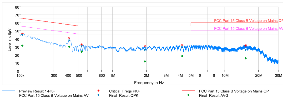
Plot 7-56. Line-Conducted Test Plot (N)
