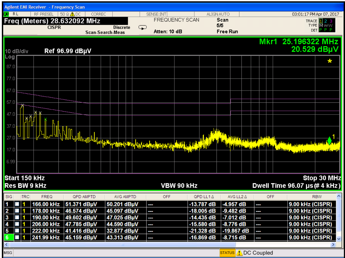
Plot 7-1. Line Conducted Plot with 802.11b (L1)
