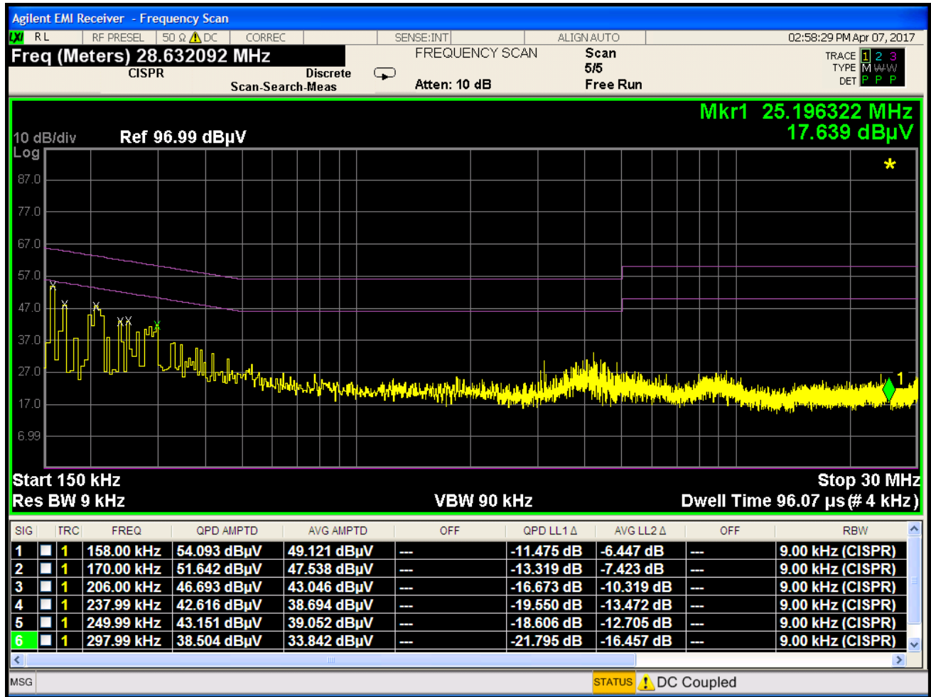
Plot 7-2. Line Conducted Plot with 802.11b (N)
