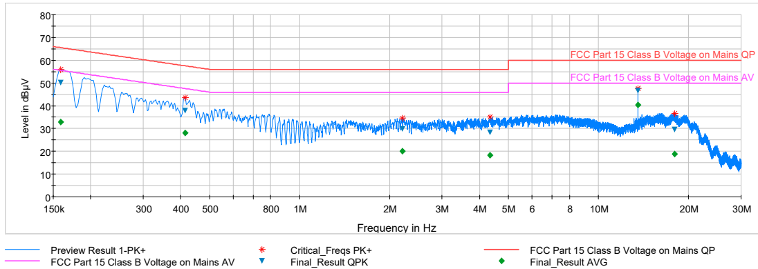
Plot 8-1. Line-Conducted Test Plot (L1)
