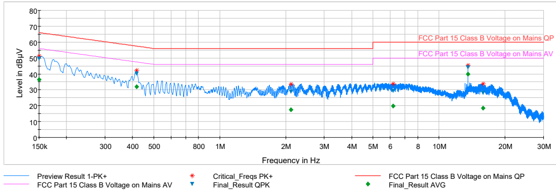
Plot 8-3. Line-Conducted Test Plot (N)
