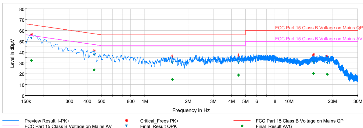
Plot 7-43. Line Conducted Plot with 802.11b (L1)
