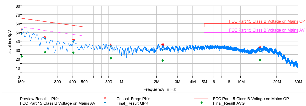
Plot 7-44. Line Conducted Plot with 802.11b (N)
