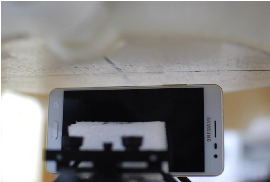
SAR Test Setup Photo 10 – Left Edge 1.0 cm
