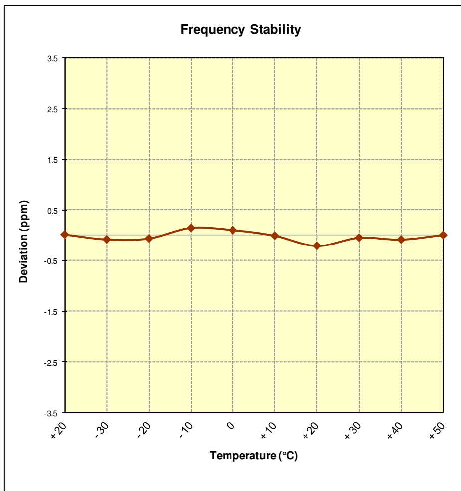
Figure 7-10. Frequency Stability Graph (AWS WCDMA Mode – Ch. 1762)
