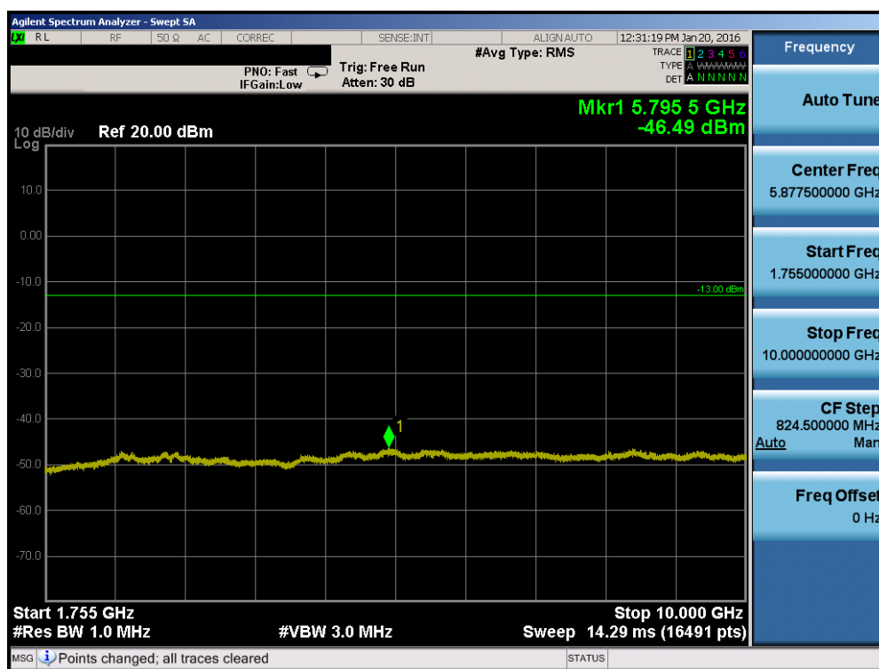
Plot 7-39. Conducted Spurious Plot (AWS WCDMA Mode – Ch. 1412)
