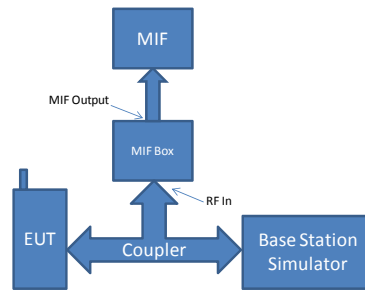
Figure 7-1 MIF Measurement Setup for licensed modes
