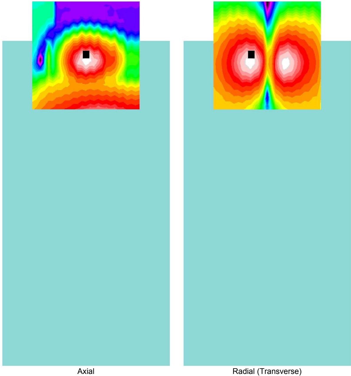
Figure 6-1 T-Coil Scan Overlay Magnetic Field Distributions
