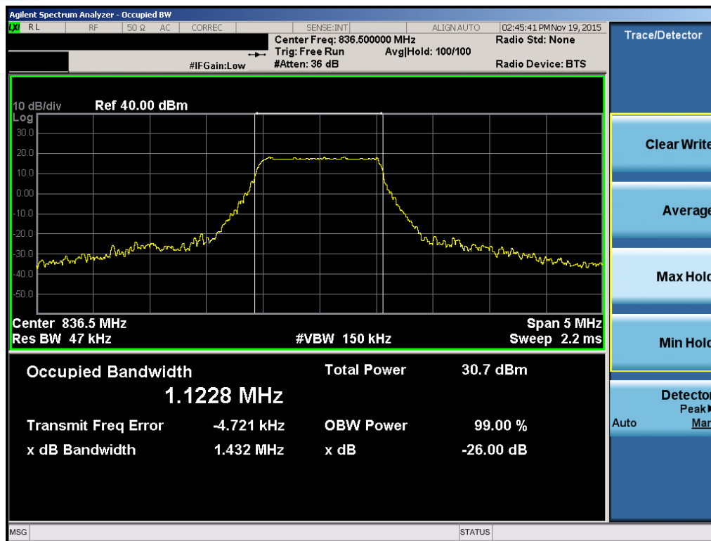
Plot 7-9. Occupied Bandwidth Plot (Band 5 – 1.4MHz QPSK – RB Size 6)
