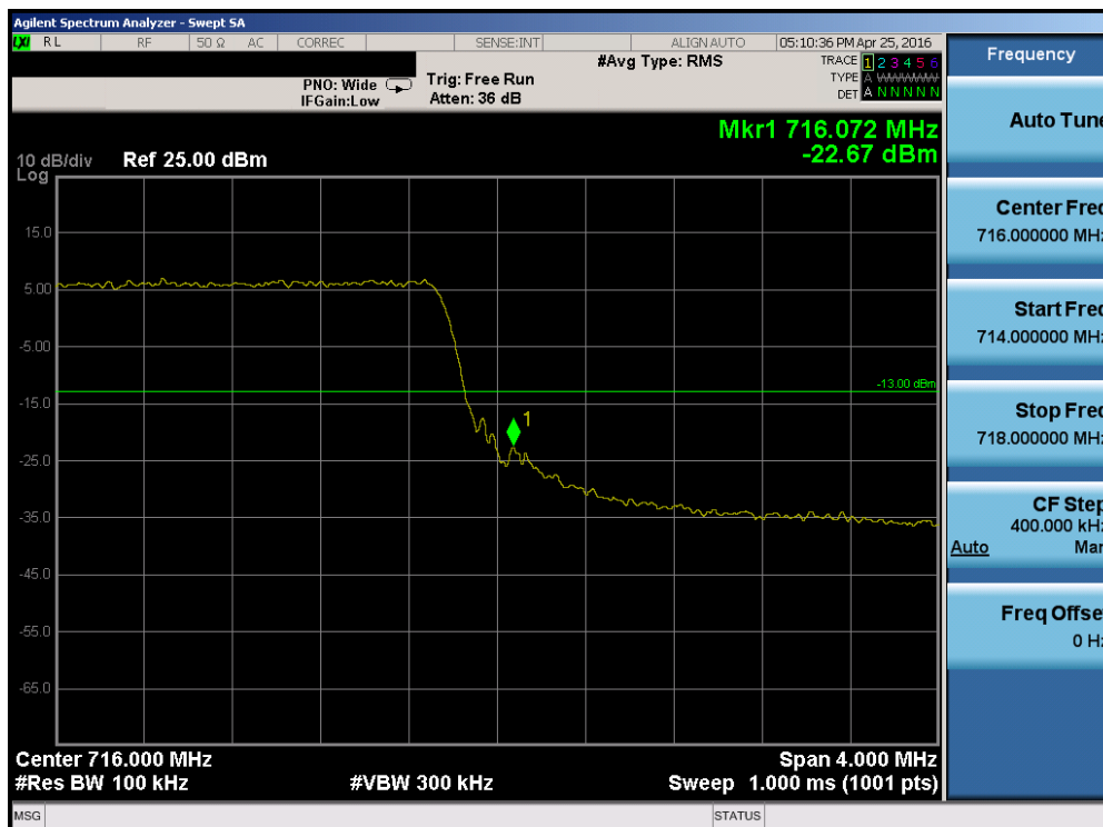
Plot 7-15. Upper Band Edge Plot (Band 17 – 5.0MHz QPSK – RB Size 25)
