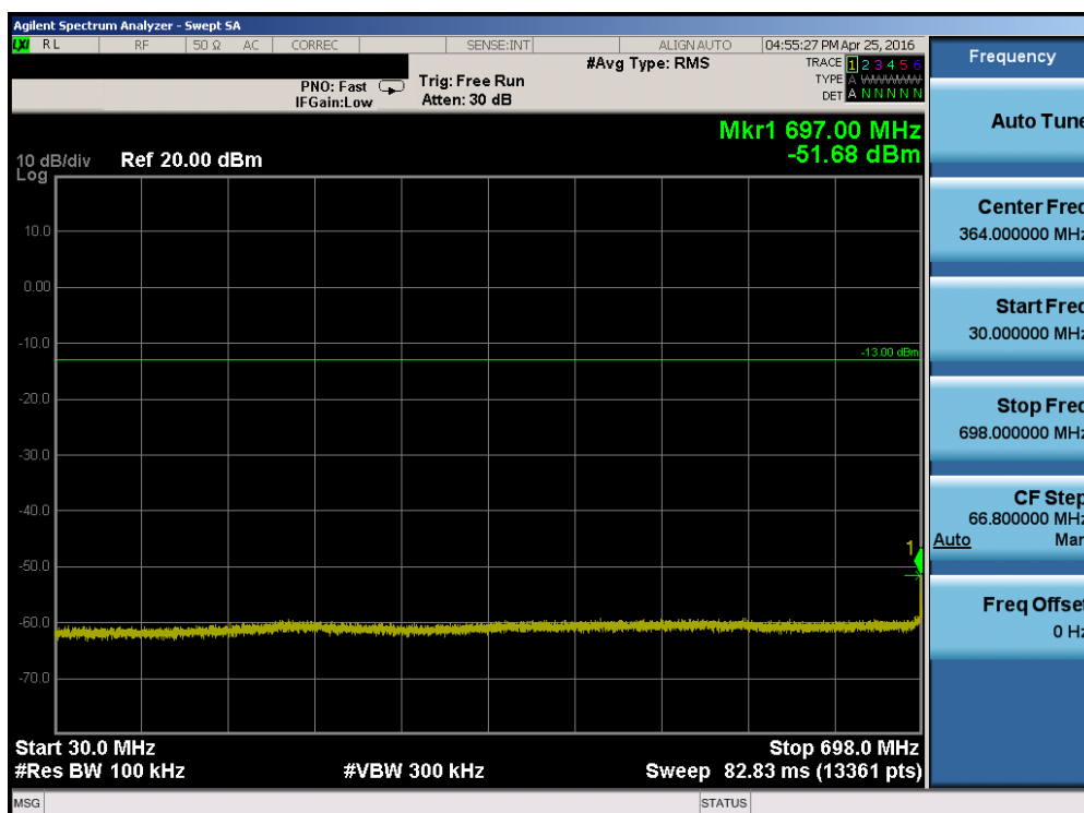
Plot 7-8. Conducted Spurious Plot (Band 17 – 10.0MHz QPSK – RB Size 1, RB Offset 0 – Mid Channel)
