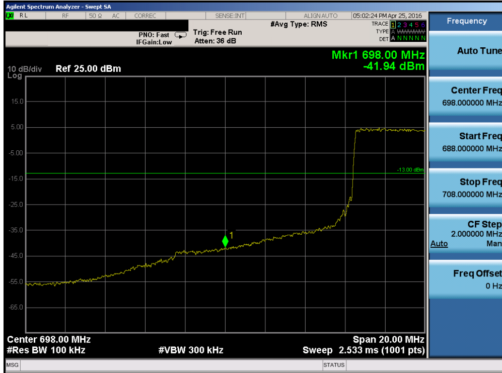
Plot 7-16. Lower Band Edge Plot (Band 17 – 10.0MHz QPSK – RB Size 50)
