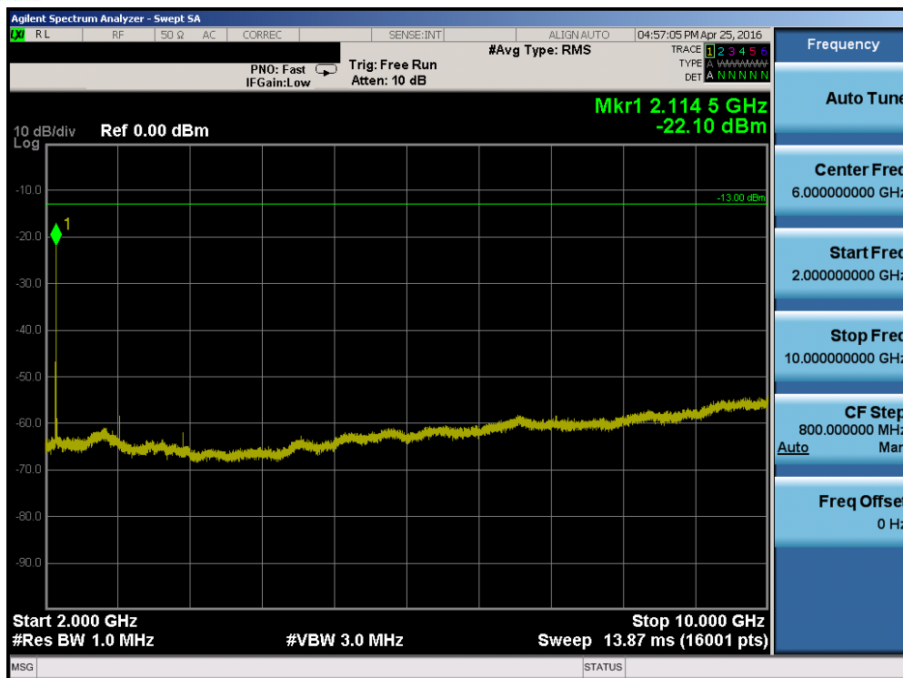
Plot 7-7. Conducted Spurious Plot (Band 17 – 10.0MHz QPSK – RB Size 1, RB Offset 0 – Low Channel)
