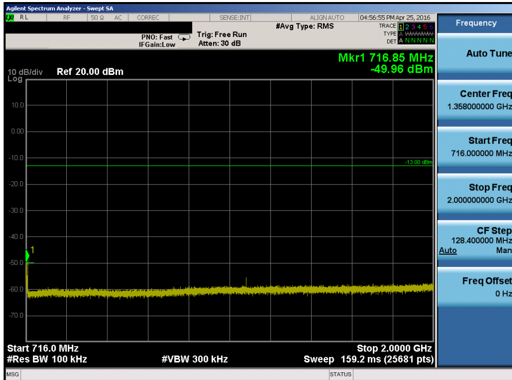
Plot 7-6. Conducted Spurious Plot (Band 17 – 10.0MHz QPSK – RB Size 1, RB Offset 0 – Low Channel)
