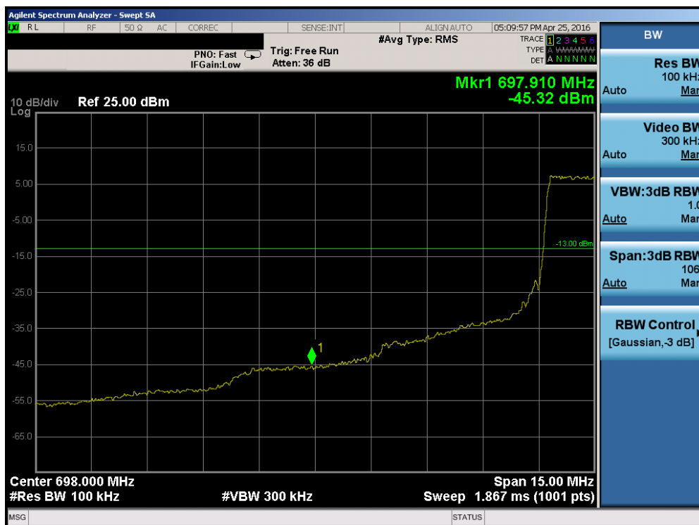
Plot 7-14. Lower Band Edge Plot (Band 17 – 5.0MHz QPSK – RB Size 25)
