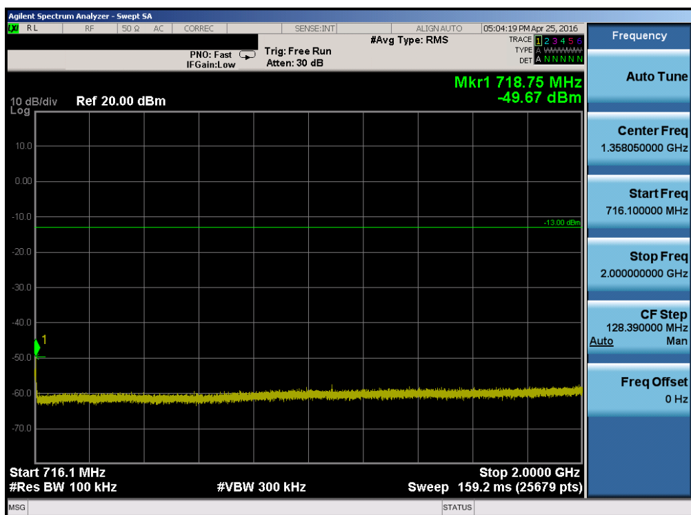
Plot 7-12. Conducted Spurious Plot (Band 17 – 10.0MHz QPSK – RB Size 1, RB Offset 0 – High Channel)
