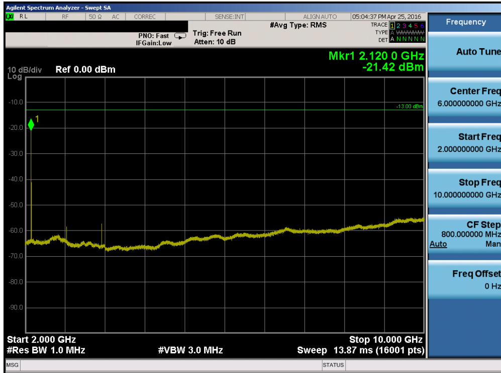
Plot 7-13. Conducted Spurious Plot (Band 17 – 10.0MHz QPSK – RB Size 1, RB Offset 0 – High Channel)
