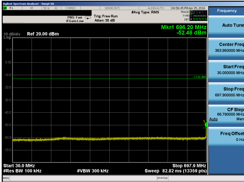
Plot 7-5. Conducted Spurious Plot (Band 17 – 10.0MHz QPSK – RB Size 1, RB Offset 0– Low Channel)
