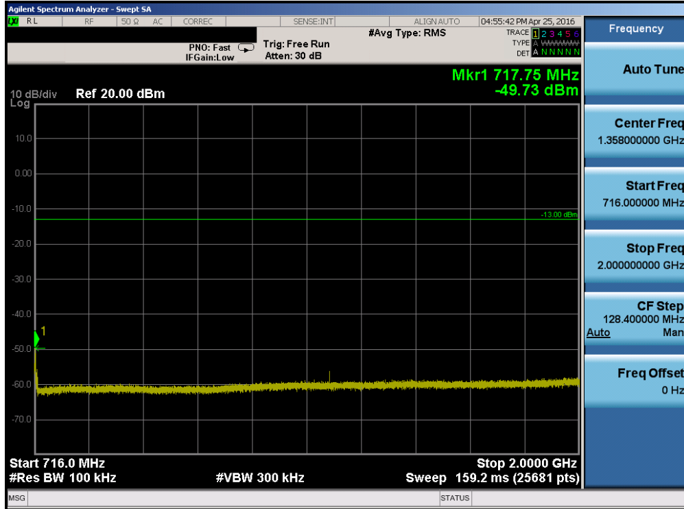
Plot 7-9. Conducted Spurious Plot (Band 17 – 10.0MHz QPSK – RB Size 1, RB Offset 0 – Mid Channel)
