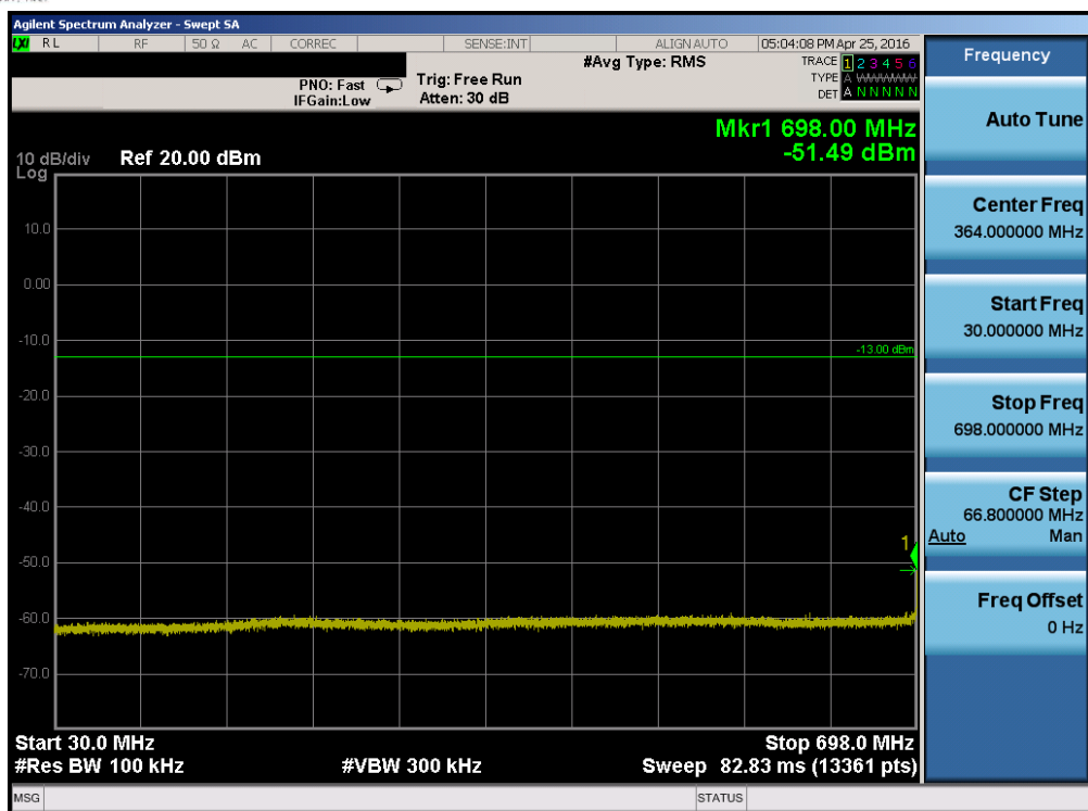
Plot 7-11. Conducted Spurious Plot (Band 17 – 10.0MHz QPSK – RB Size 1, RB Offset 0 – High Channel)
