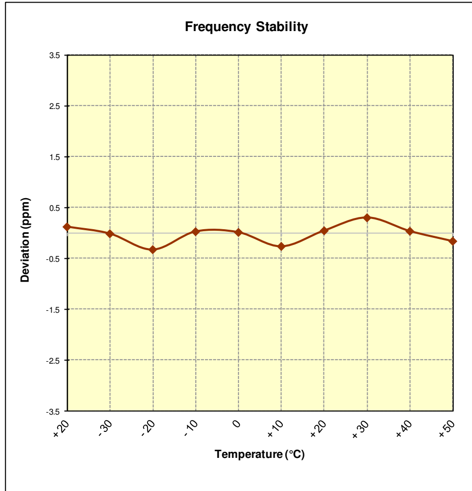
Figure 7-6. Frequency Stability Graph (Band 17)
