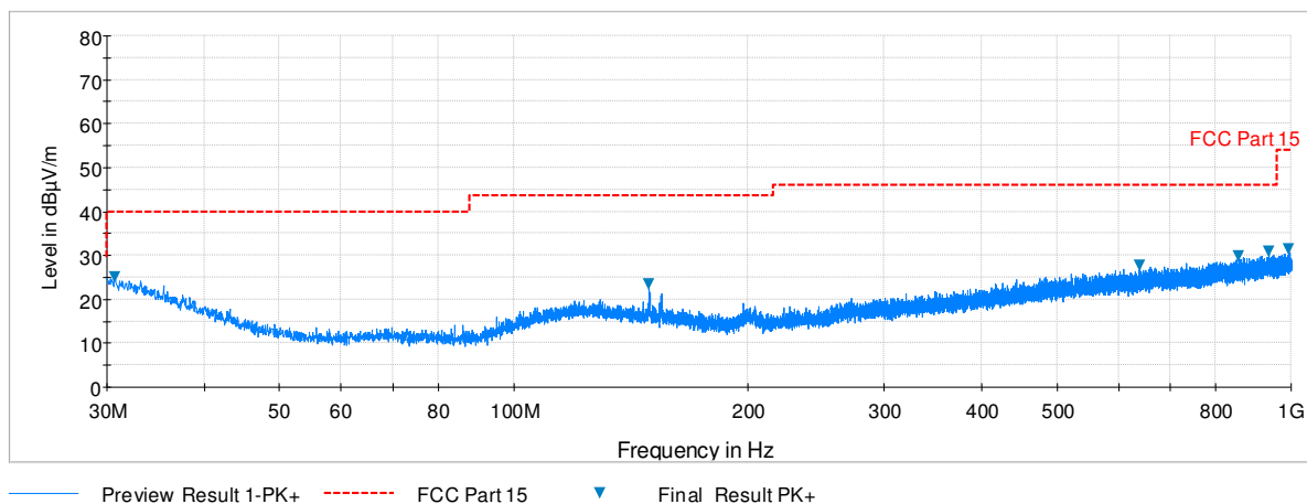
Plot 7-42. Radiated Spurious Plot below 1GHz (Pol. V)
