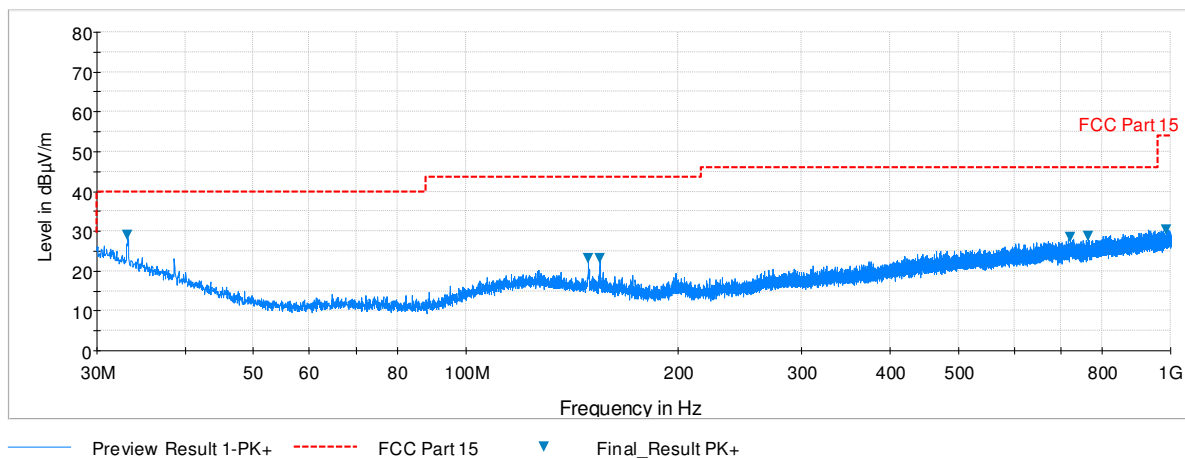
Plot 7-41. Radiated Spurious Plot below 1GHz (Pol. H)
