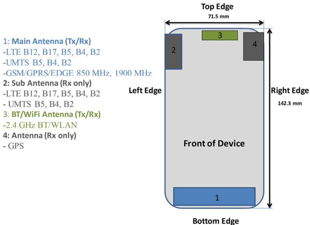
Figure F-1 DUT Antenna Locations
