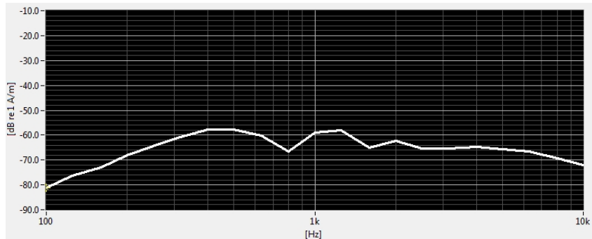
Figure 7-2 Worst-case ABM2 Plot for CDMA
