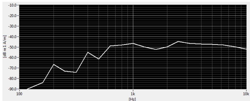
Figure 7-3 Worst-case ABM2 Plot for GSM
