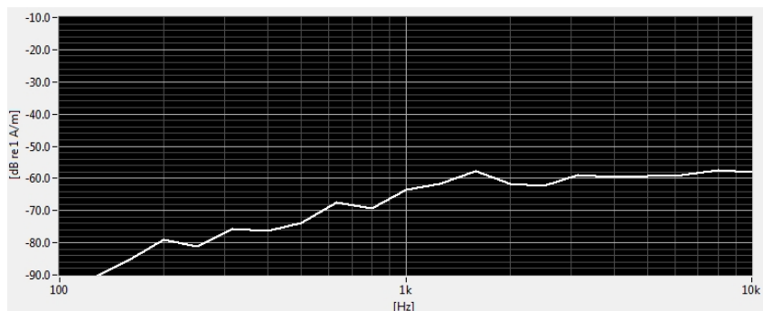
Figure 7-4 Worst-case ABM2 Plot for UMTS
