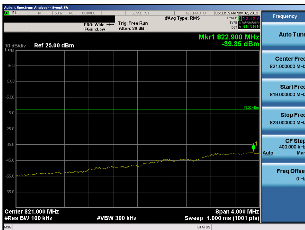
Plot 7-111. Lower Extended Band Edge Plot (Band 5/26 – 1.4MHz QPSK – RB Size 6)
