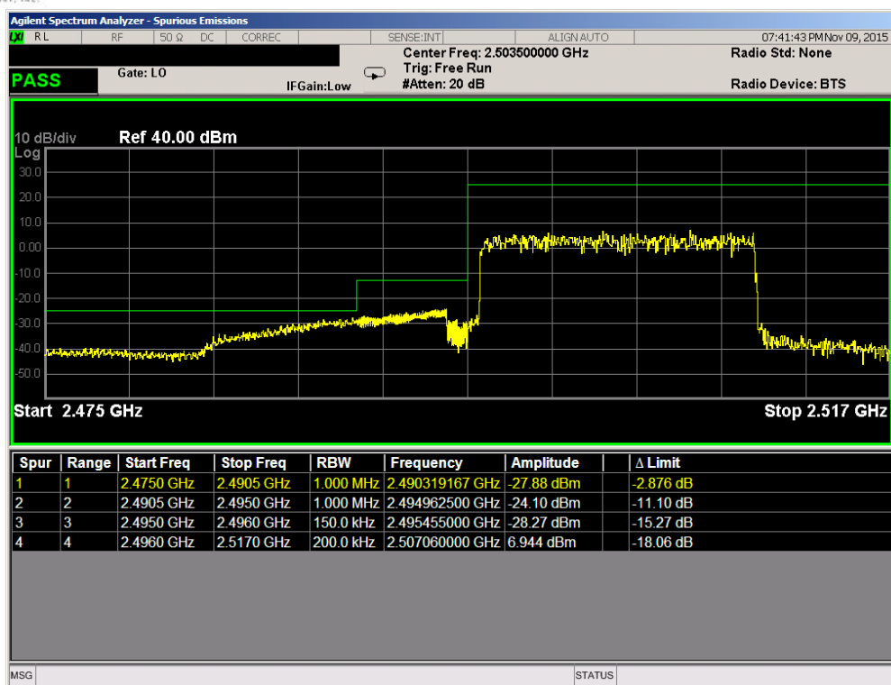
Plot 7-178. Lower ACP Plot (Band 41 – 15.0MHz QPSK – RB Size 75)
