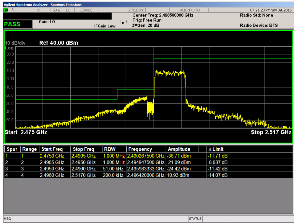
Plot 7-174. Lower ACP Plot (Band 41 – 5.0MHz QPSK – RB Size 25)
