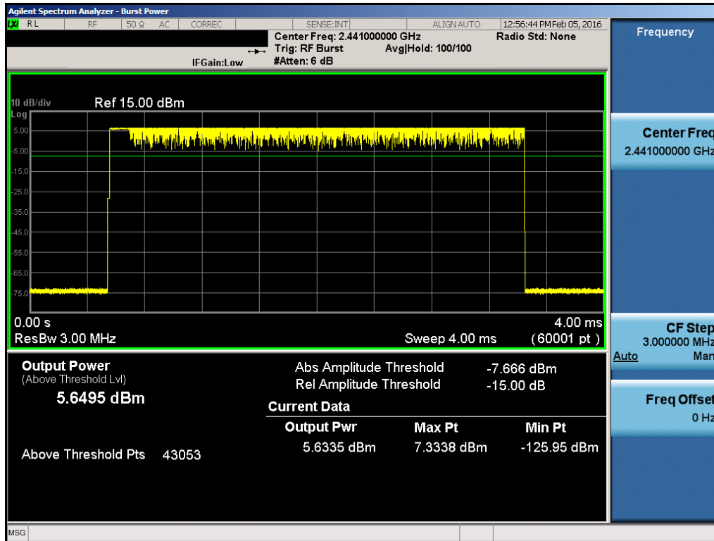
Plot 7-23. Average Conducted Power (2Mbps – Ch. 39)
