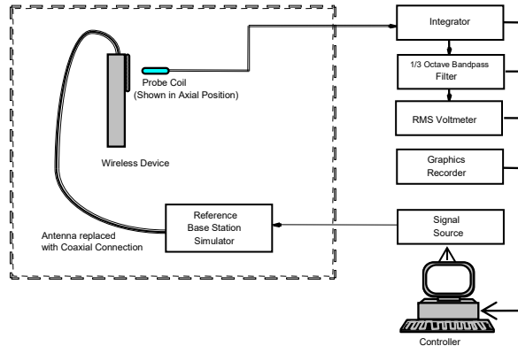
Figure 5-11 Audio Magnetic Field Test Setup
