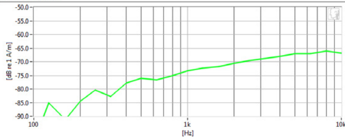
Frequency Response
