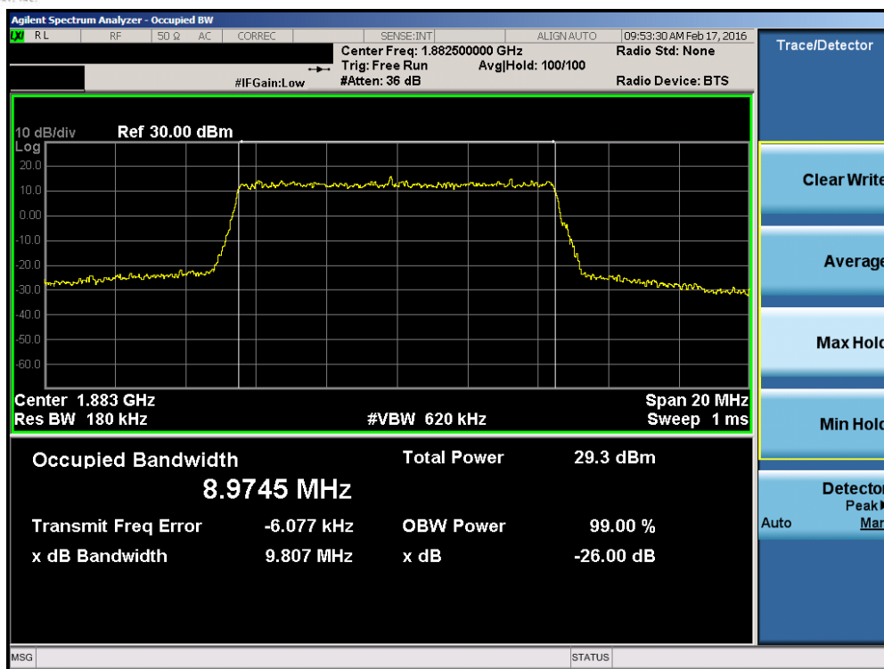
Plot 7-35. Occupied Bandwidth Plot (Band 2/25 – 10.0MHz QPSK – RB Size 50)
