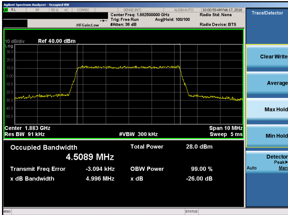
Plot 7-34. Occupied Bandwidth Plot (Band 2/25 – 5.0MHz 16-QAM – RB Size 25)
