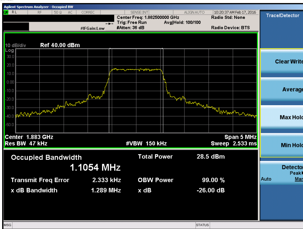
Plot 7-29. Occupied Bandwidth Plot (Band 2/25 – 1.4MHz QPSK – RB Size 6)
