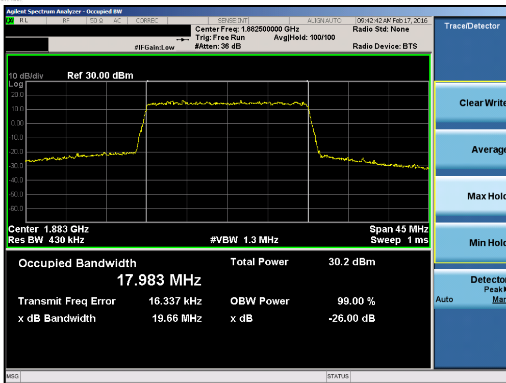
Plot 7-39. Occupied Bandwidth Plot (Band 2/25 – 20.0MHz QPSK – RB Size 100)
