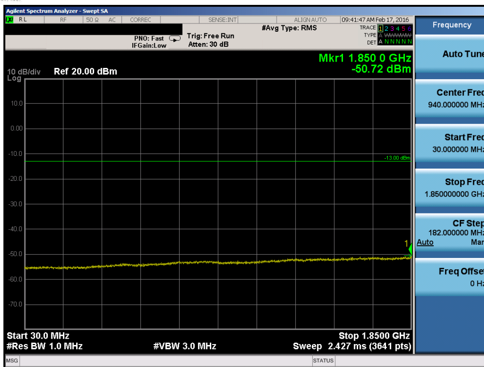
Plot 7-71. Conducted Spurious Plot (Band 2/25 – 20.0MHz QPSK – RB Size 1, RB Offset 0 – Mid Channel)
