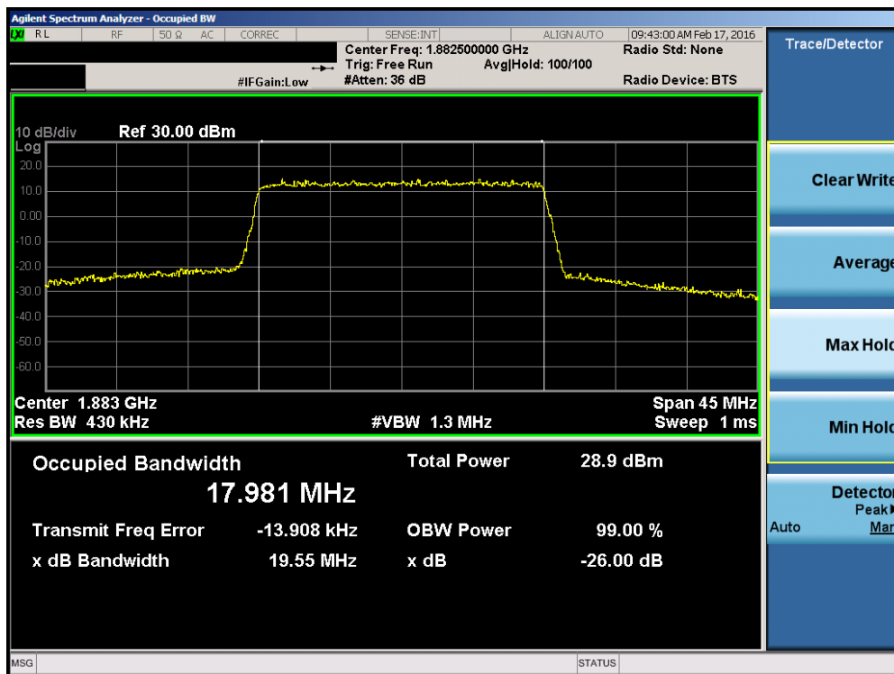
Plot 7-40. Occupied Bandwidth Plot (Band 2/25 – 20.0MHz 16-QAM – RB Size 100)
