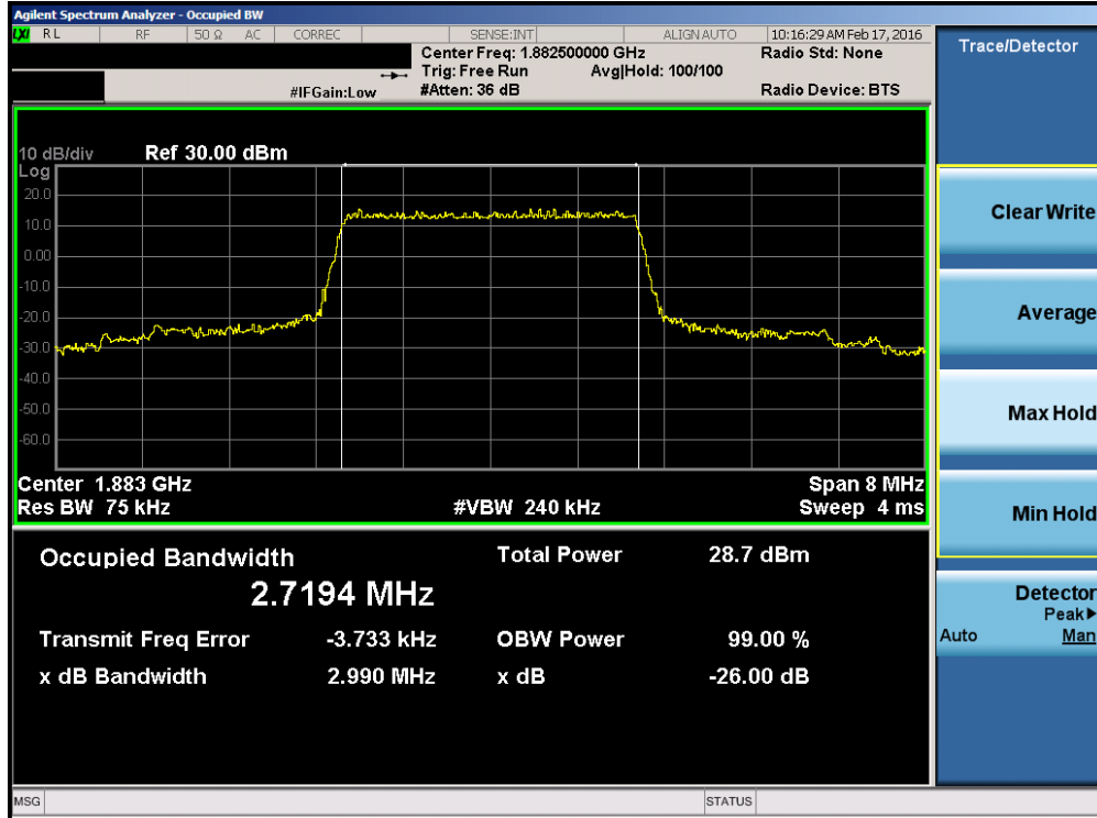
Plot 7-31. Occupied Bandwidth Plot (Band 2/25 – 3.0MHz QPSK – RB Size 15)
