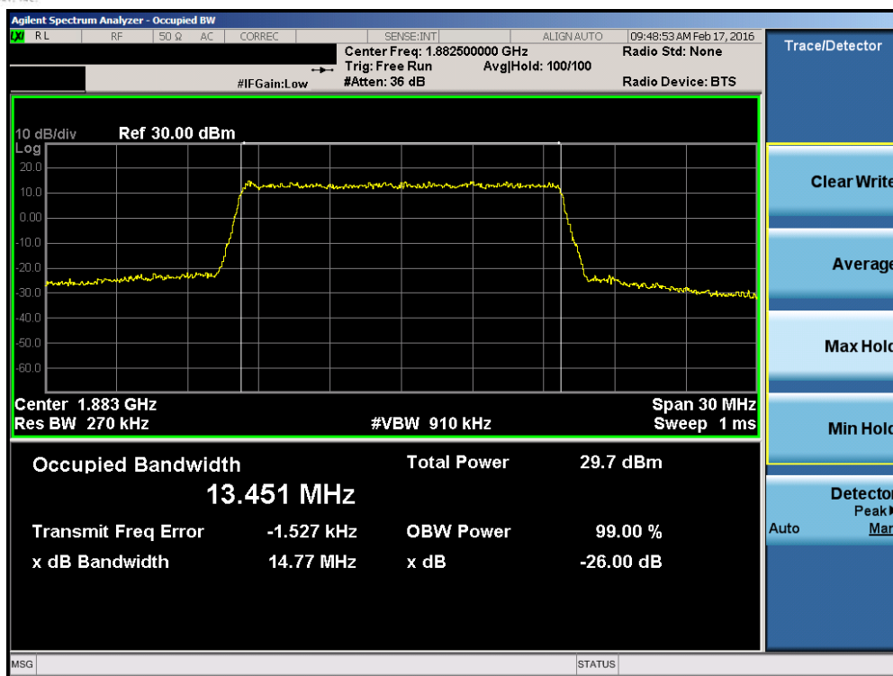
Plot 7-37. Occupied Bandwidth Plot (Band 2/25 – 15.0MHz QPSK – RB Size 75)
