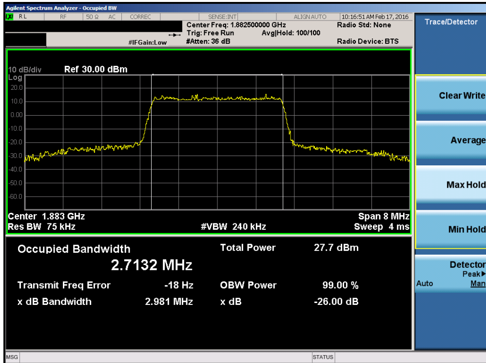
Plot 7-32. Occupied Bandwidth Plot (Band 2/25 – 3.0MHz 16-QAM – RB Size 15)
