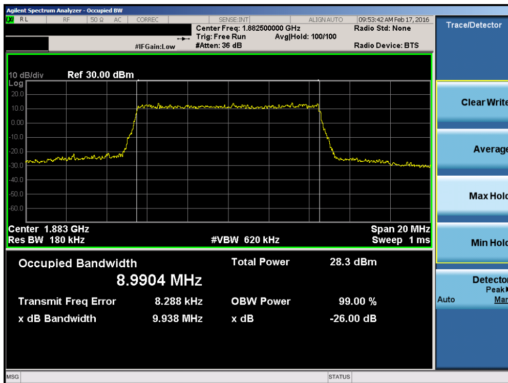
Plot 7-36. Occupied Bandwidth Plot (Band 2/25 – 10.0MHz 16-QAM – RB Size 50)
