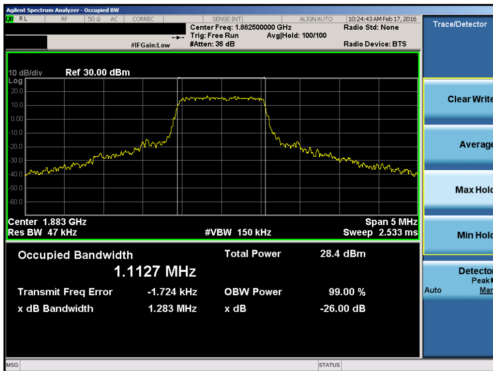
Plot 7-30. Occupied Bandwidth Plot (Band 2/25 – 1.4MHz 16-QAM – RB Size 6)
