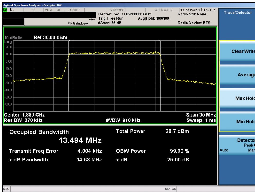
Plot 7-38. Occupied Bandwidth Plot (Band 2/25 – 15.0MHz 16-QAM – RB Size 75)
