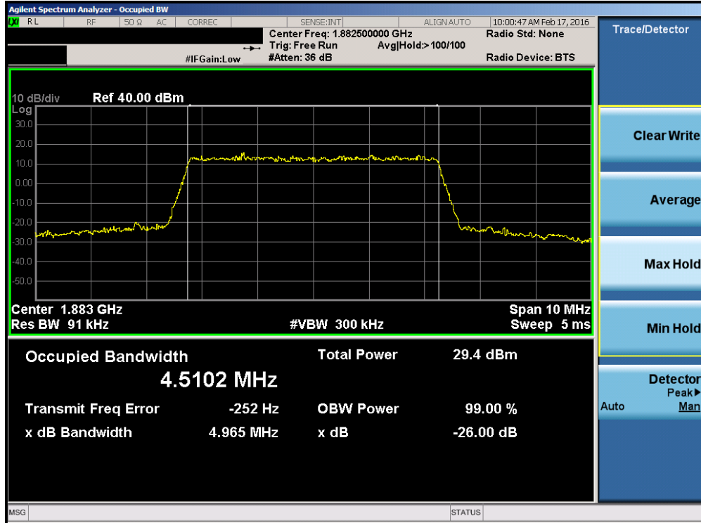
Plot 7-33. Occupied Bandwidth Plot (Band 2/25 – 5.0MHz QPSK – RB Size 25)
