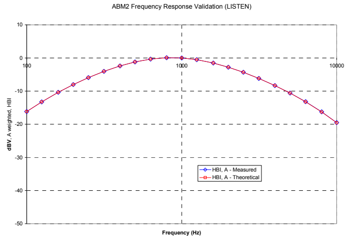
Figure 5-7 ABM2 Frequency Response Validation
