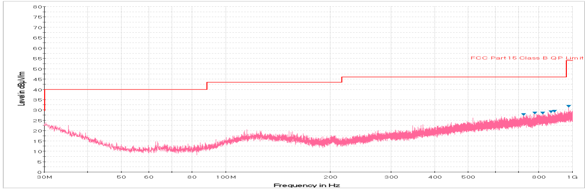
Plot 7-93. Radiated Spurious Plot below 1GHz (802.11a – U3 Ch. 157, Ant. Pol. H)
