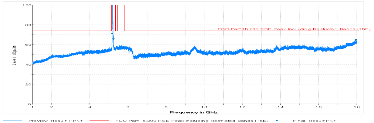
Plot 7-67. Radiated Spurious Plot above 1GHz (802.11a – U1 Ch. 40, Ant. Pol. H)
