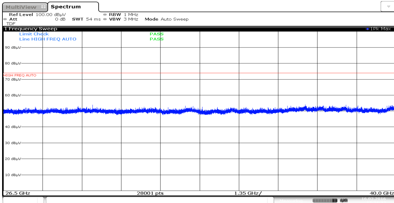
Plot 7-78. Radiated Spurious Plot above 26GHz (802.11a – Ant. Pol. V)
