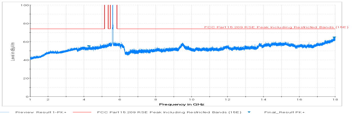
Plot 7-72. Radiated Spurious Plot above 1GHz (802.11a – U2C Ch. 116, Ant. Pol. V)
