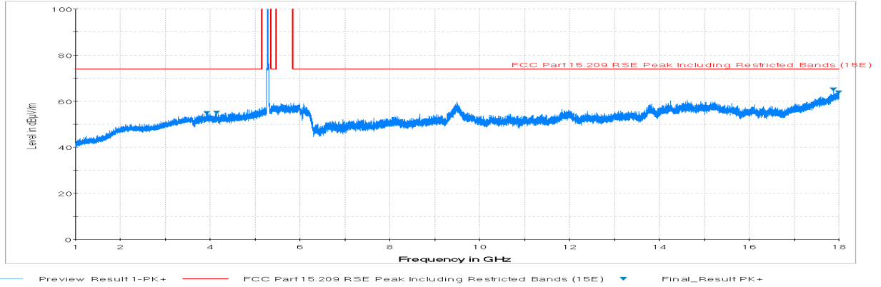
Plot 7-70. Radiated Spurious Plot above 1GHz (802.11a – U2A Ch. 56, Ant. Pol. V)
