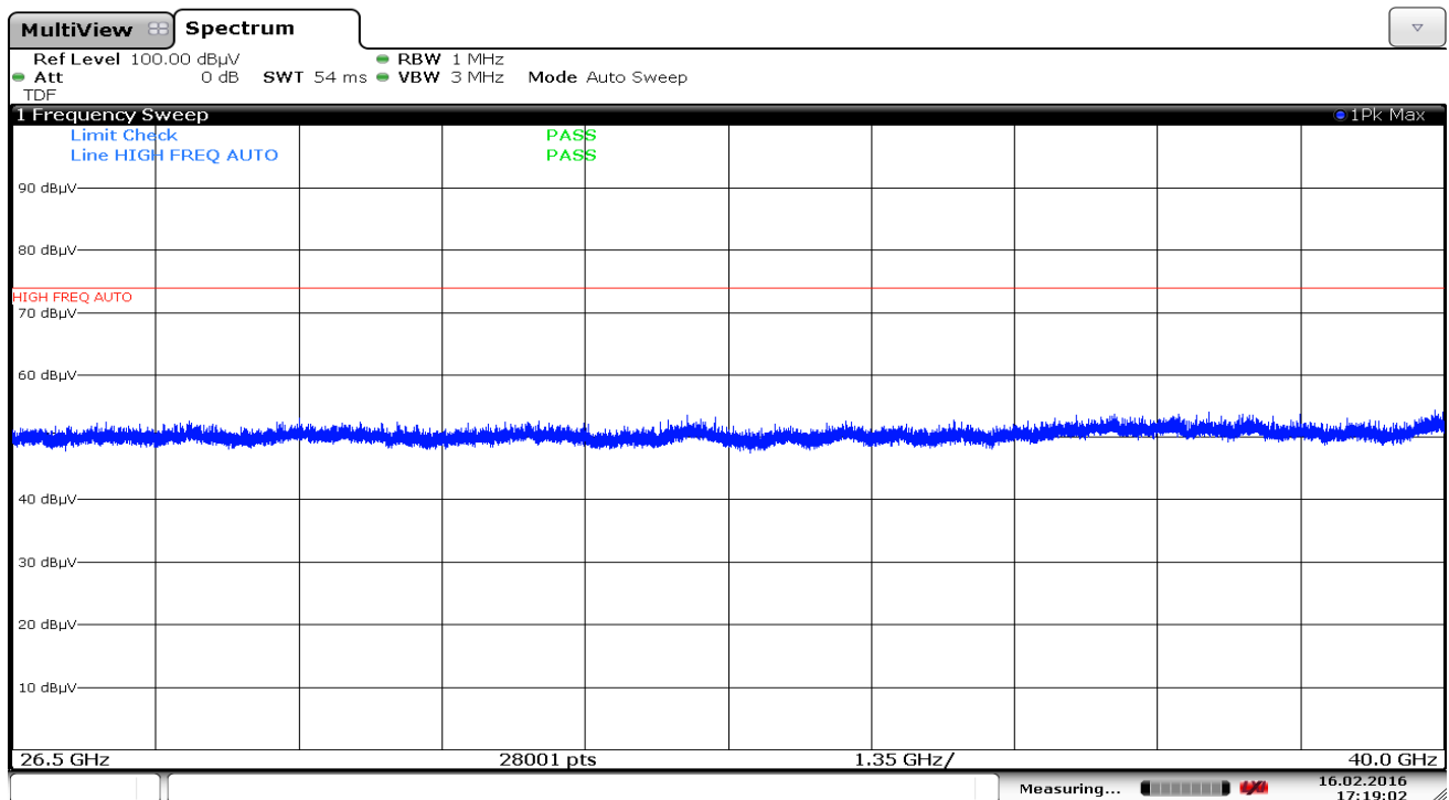
Plot 7-76. Radiated Spurious Plot above 26GHz (802.11a – Ant. Pol. H)
