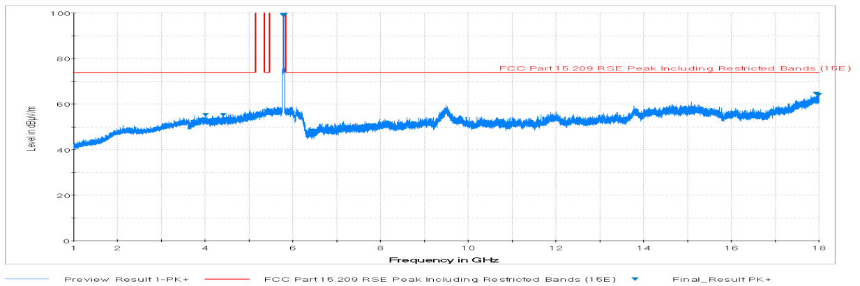
Plot 7-74. Radiated Spurious Plot above 1GHz (802.11a – U3 Ch. 157, Ant. Pol. V)
