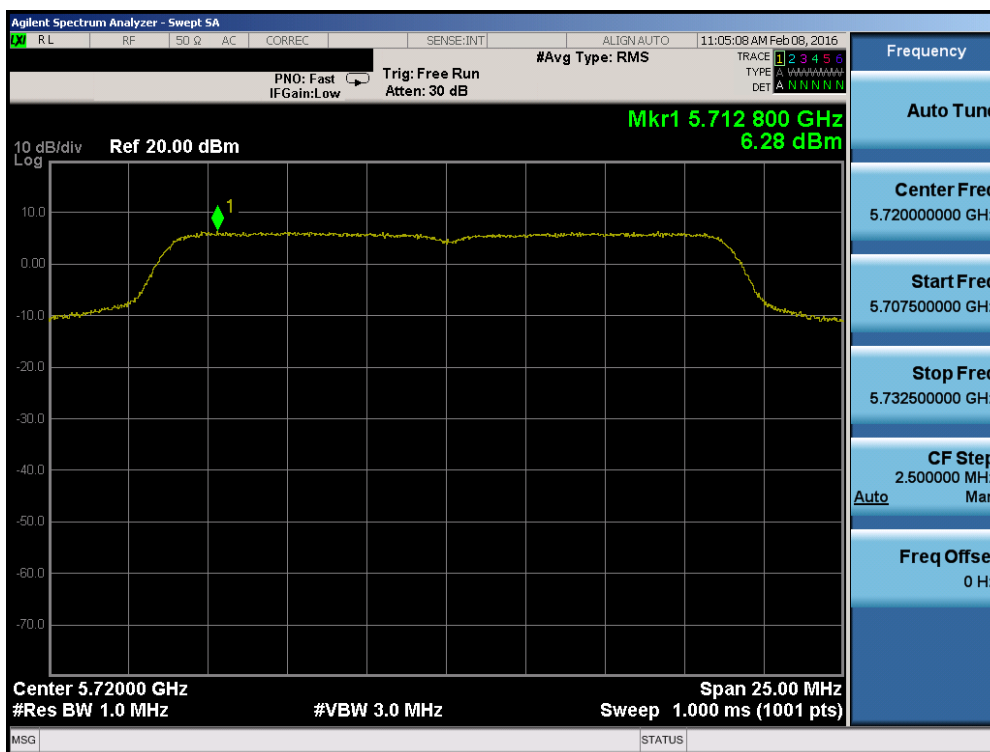
Plot 7-55. Power Spectral Density Plot (20MHz BW 802.11n (UNII Band 2C) – Ch. 144)
