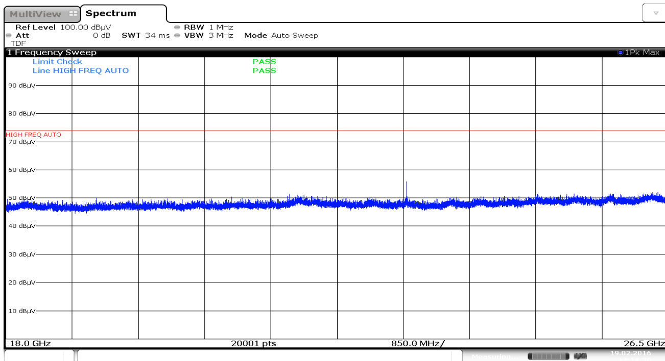
Plot 7-77. Radiated Spurious Plot above 18GHz (802.11a – Ant. Pol. V)
