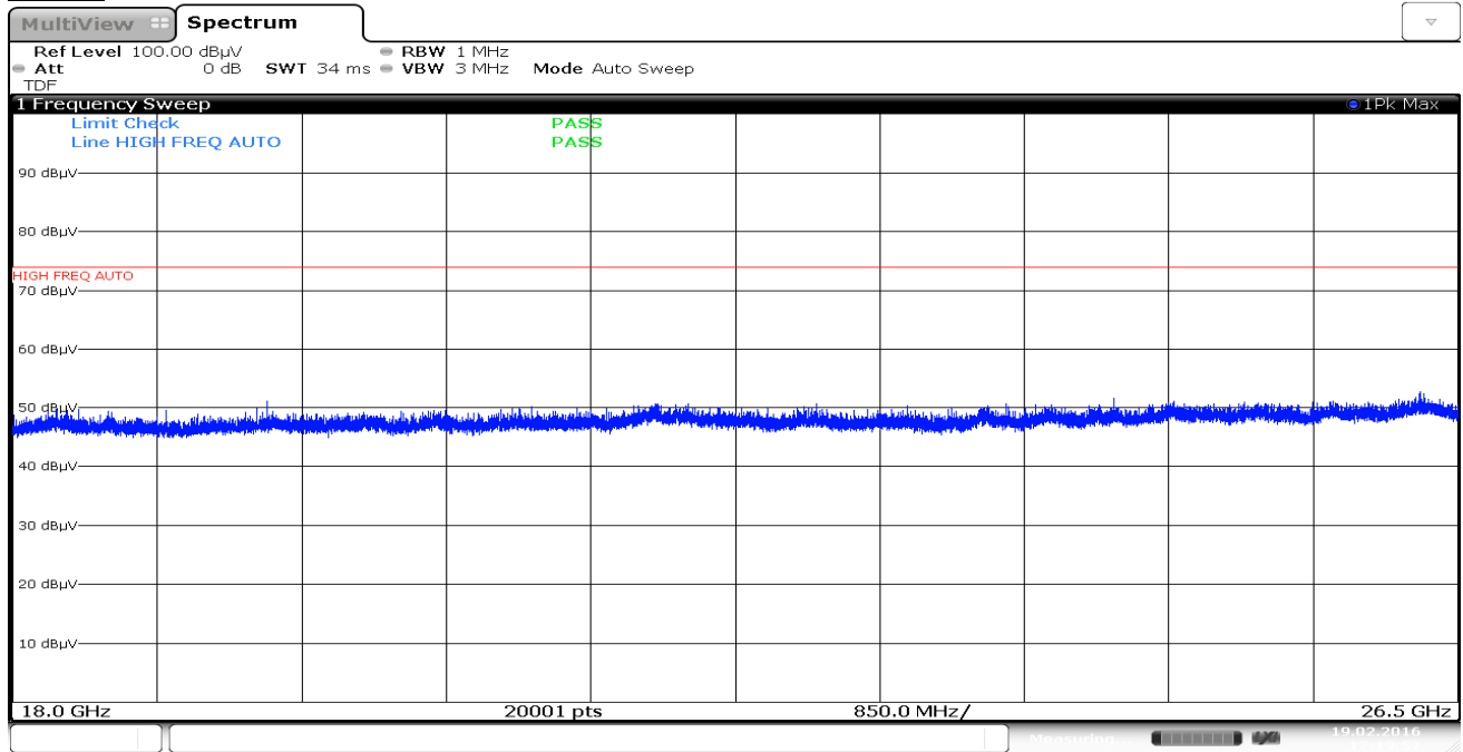
Plot 7-37. Radiated Spurious Plot above 18GHz (Pol. H)
