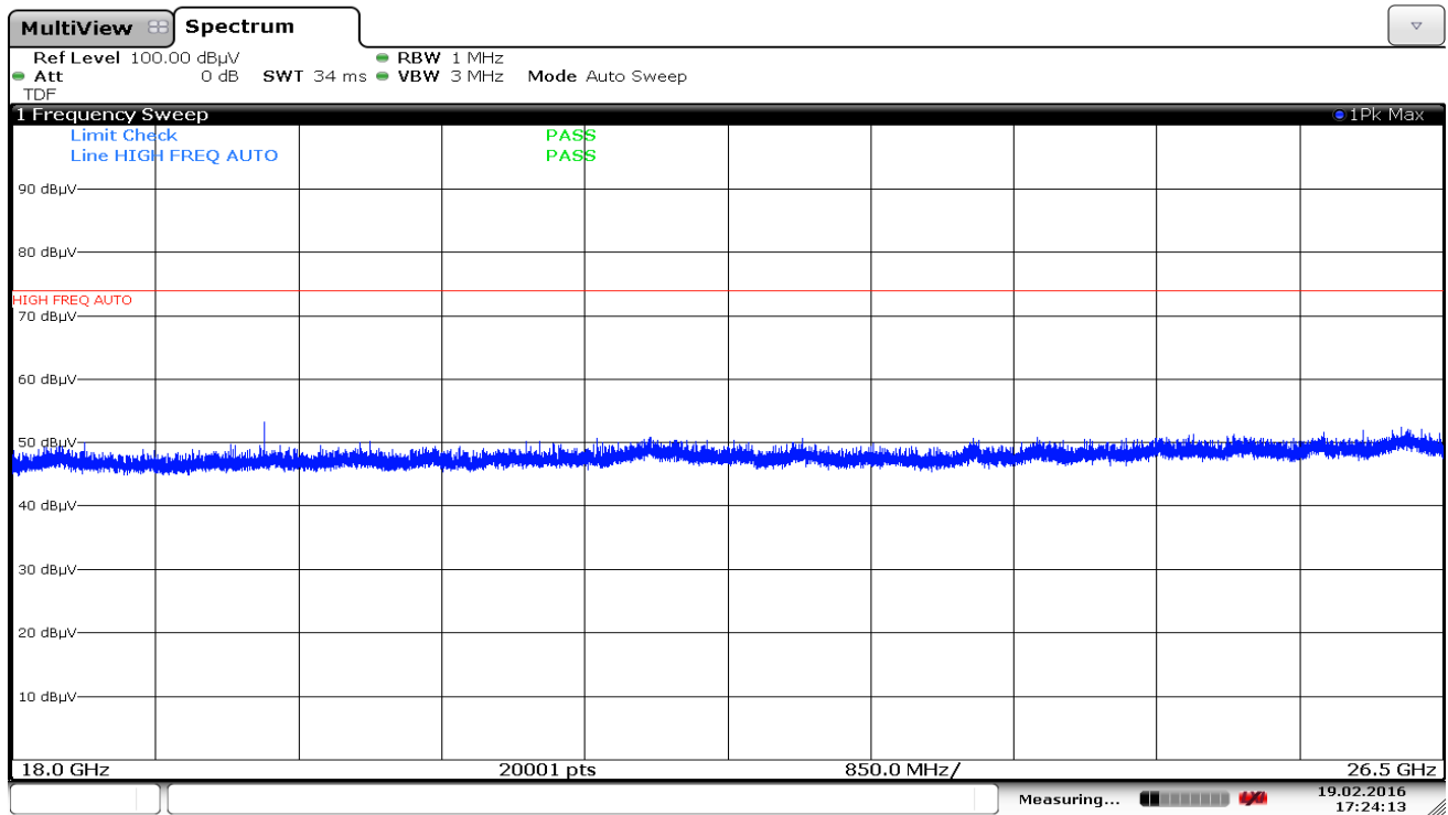
Plot 7-38. Radiated Spurious Plot above 18GHz (Pol. V)
