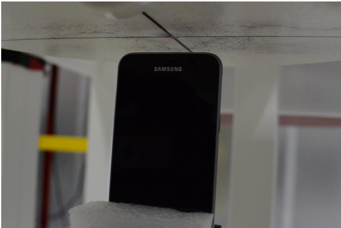
SAR Test Setup Photo 7: Top at 1.0 cm
