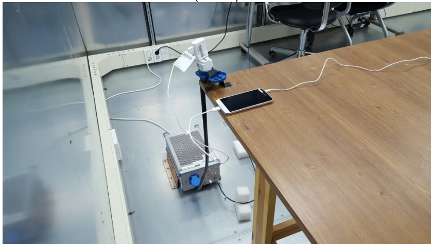
LINE CONDUCTED EMISSION (BACK)
