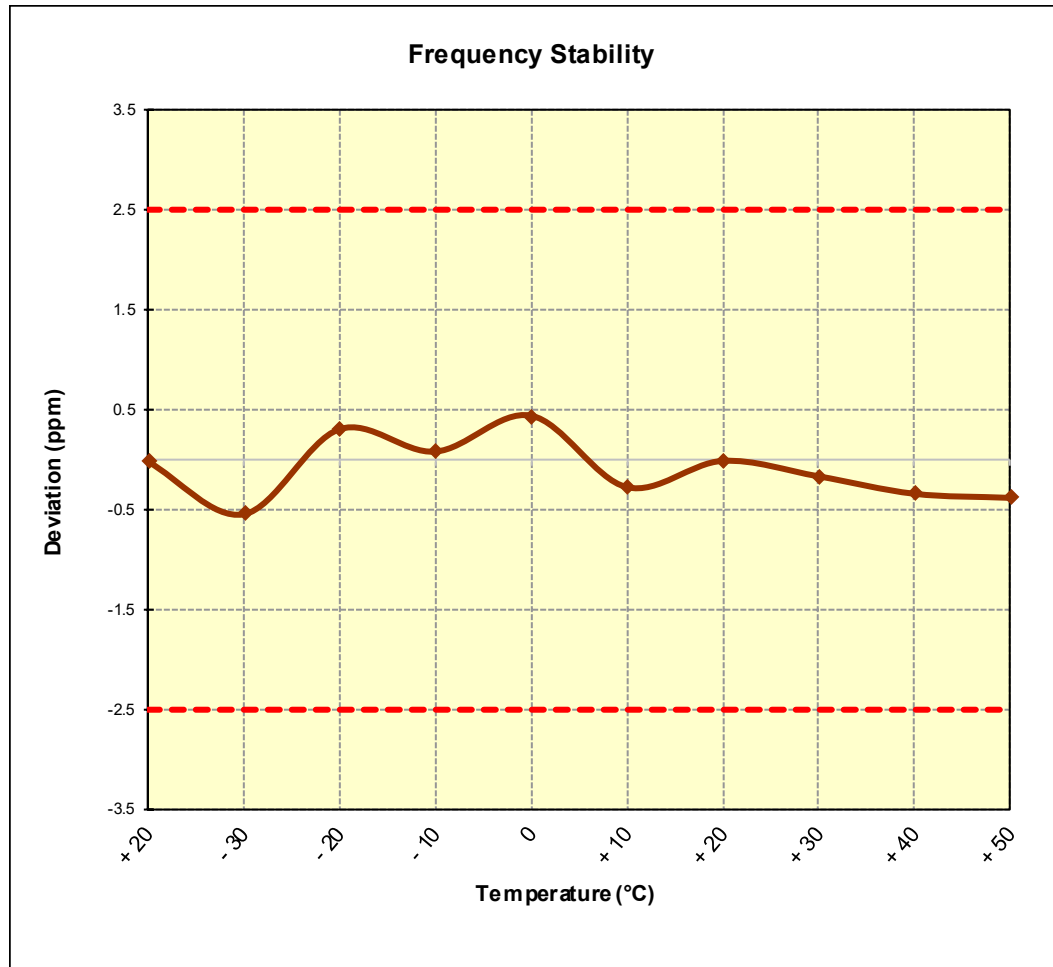
Figure 7-9. Frequency Stability Graph (Cellular CDMA Mode – Ch. 384)
