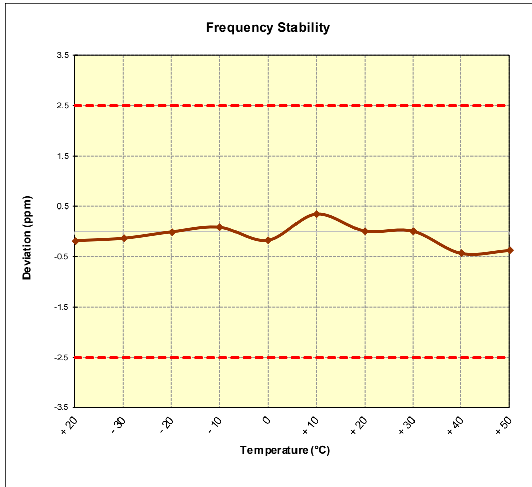
Figure 7-10. Frequency Stability Graph (Cellular WCDMA Mode – Ch. 4183)
