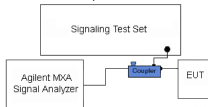
Figure 7-4. Test Instrument & Measurement Setup
