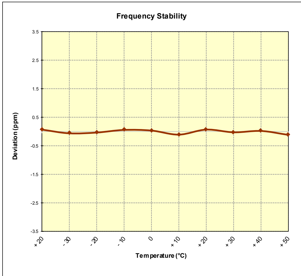
Figure 7-12. Frequency Stability Graph (PCS GPRS Mode – Ch. 661)
