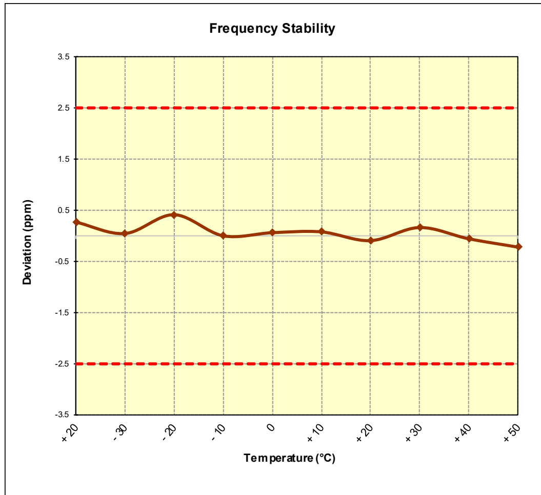
Figure 7-8. Frequency Stability Graph (Cellular GPRS Mode – Ch. 190)
