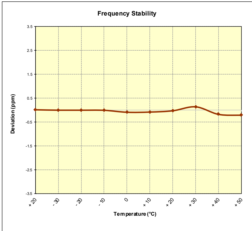
Figure 7-14. Frequency Stability Graph (PCS WCDMA Mode – Ch. 9400)
