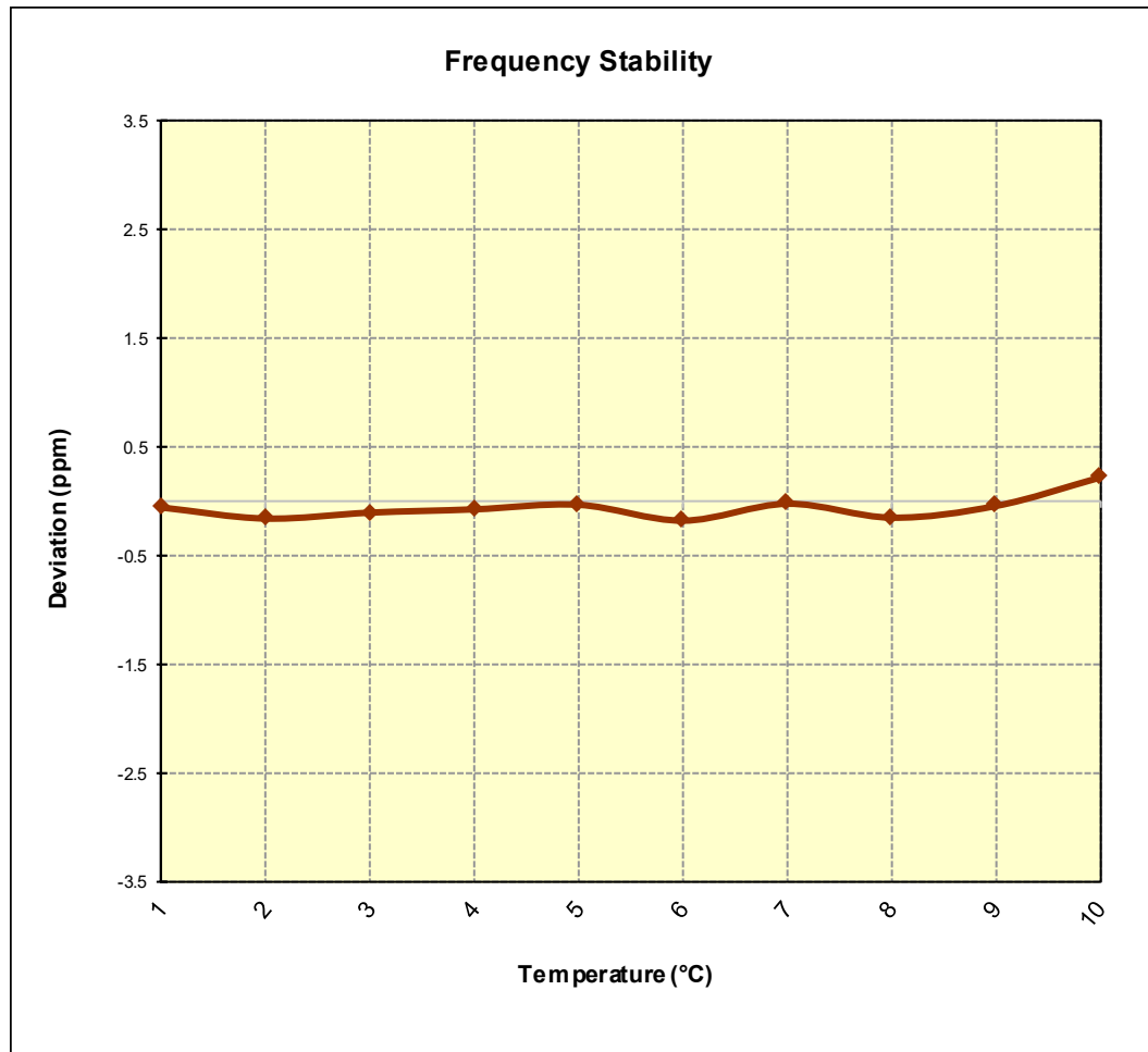
Figure 7-11. Frequency Stability Graph (AWS WCDMA Mode – Ch. 1412)
