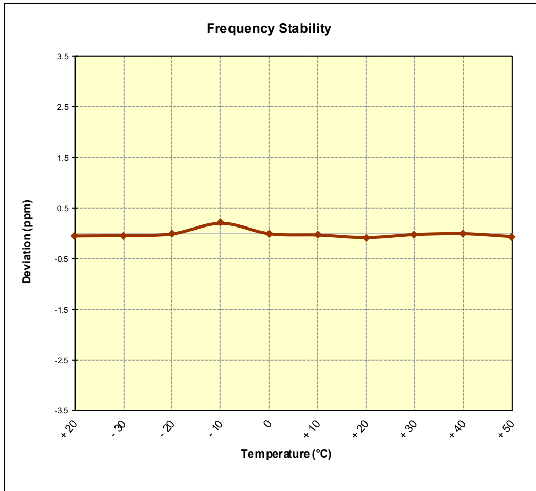
Figure 7-13. Frequency Stability Graph (PCS CDMA Mode – Ch. 600)
