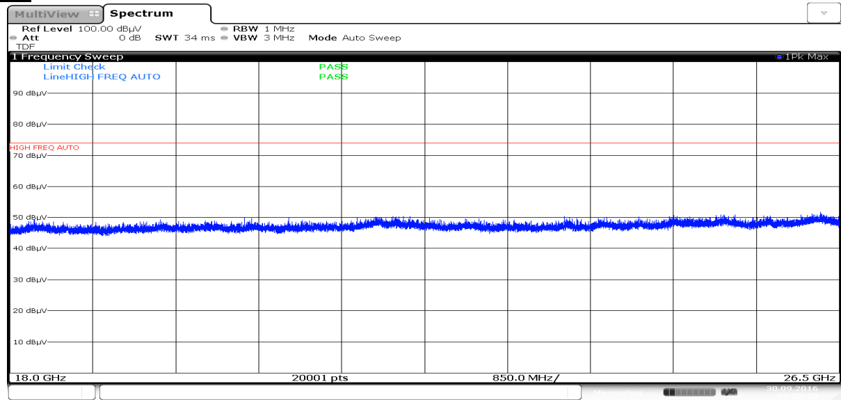
Plot 7-48. Radiated Spurious Plot above 18GHz (Pol. H)
