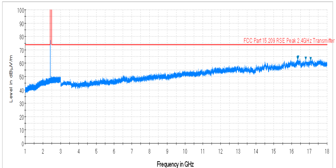
Plot 7-42. Radiated Spurious Plot above 1GHz (BT – Ch. 0, Ant. Pol. H)
