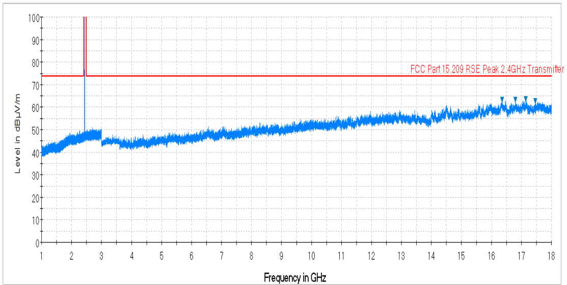
Plot 7-45. Radiated Spurious Plot above 1GHz (BT – Ch. 39, Ant. Pol. V)
