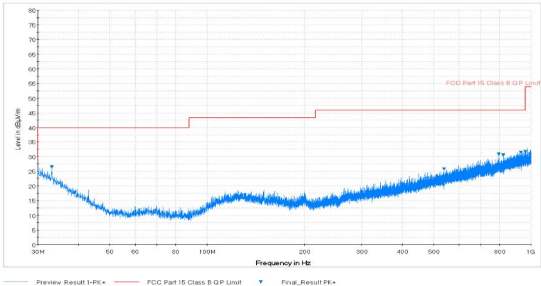
Plot 7-52. Radiated Spurious Plot below 1GHz (Pol. H)
