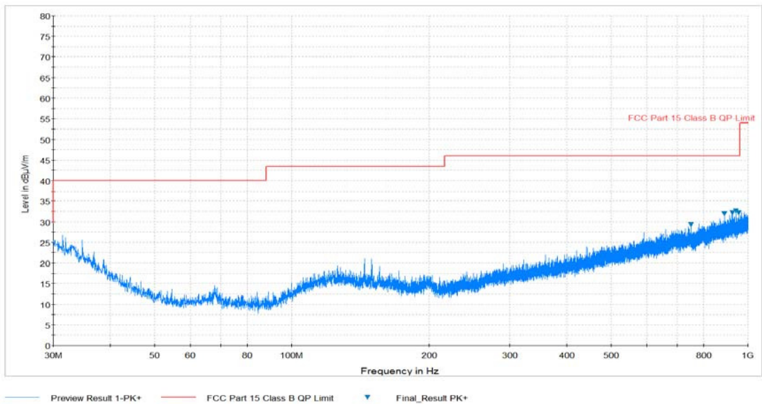
Plot 7-53. Radiated Spurious Plot below 1GHz (Pol. V)
