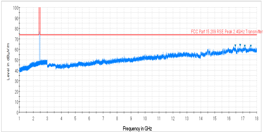
Plot 7-46. Radiated Spurious Plot above 1GHz (BT – Ch. 78, Ant. Pol. H)
