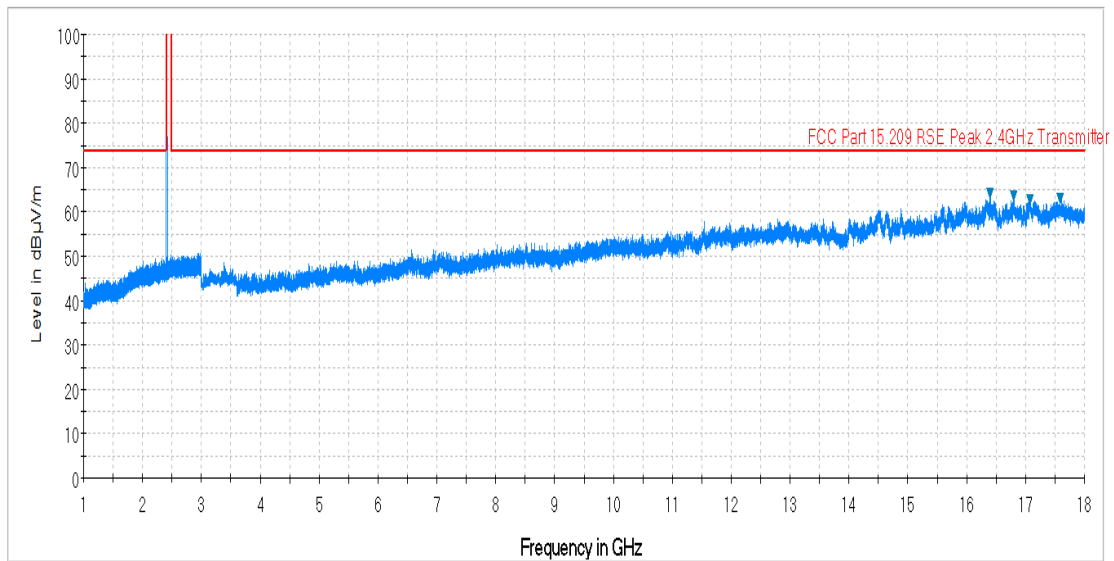
Plot 7-43. Radiated Spurious Plot above 1GHz (BT – Ch. 0, Ant. Pol. V)
