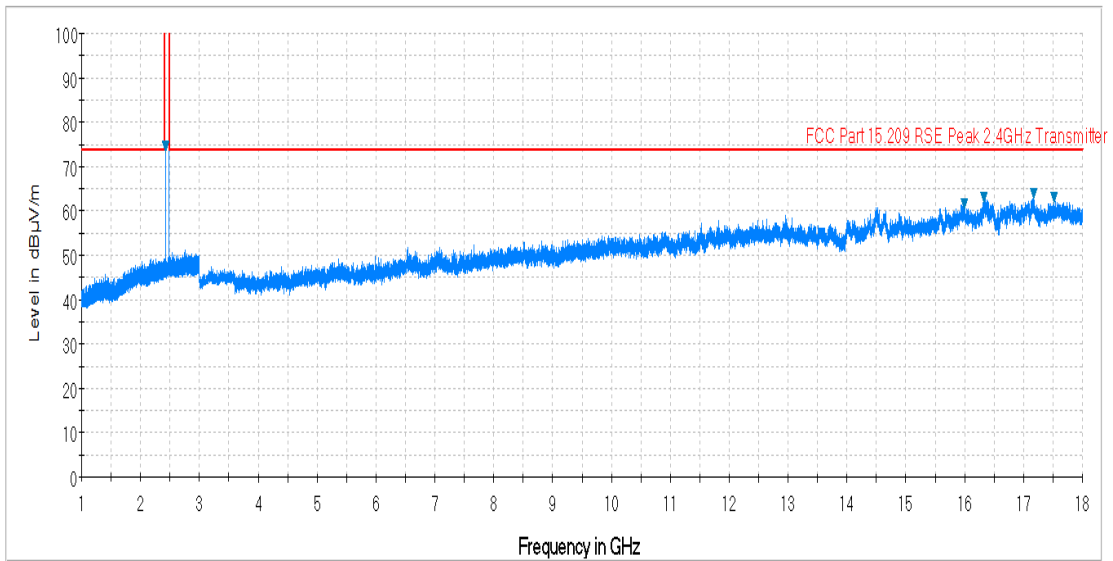
Plot 7-47. Radiated Spurious Plot above 1GHz (BT – Ch. 78, Ant. Pol. V)
