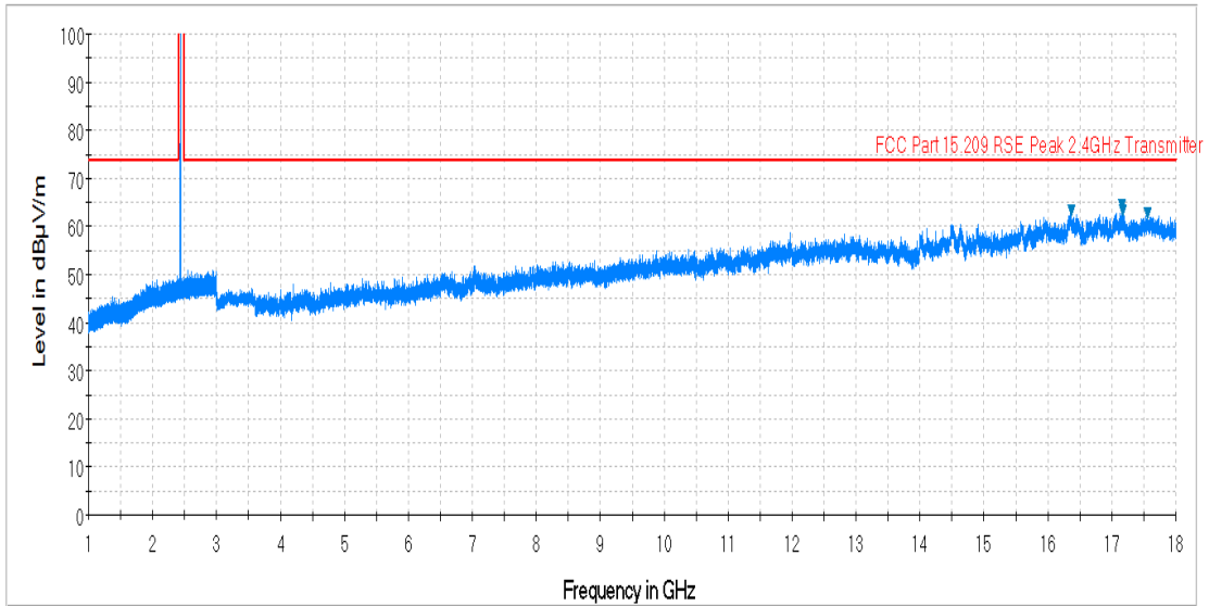
Plot 7-44. Radiated Spurious Plot above 1GHz (BT – Ch. 39, Ant. Pol. H)
