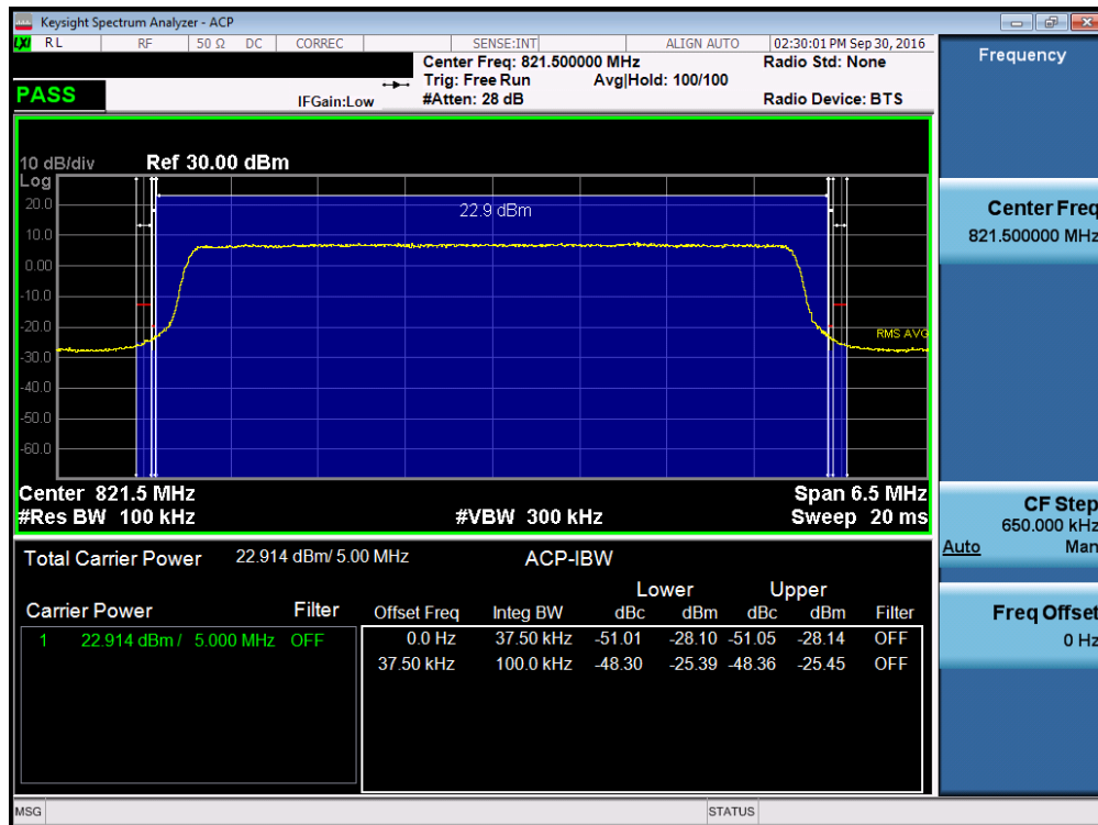
Plot 7-26. Channel Edge Plot (LTE Band 26, 5MHz QPSK – RB Size 25 – High Channel)
