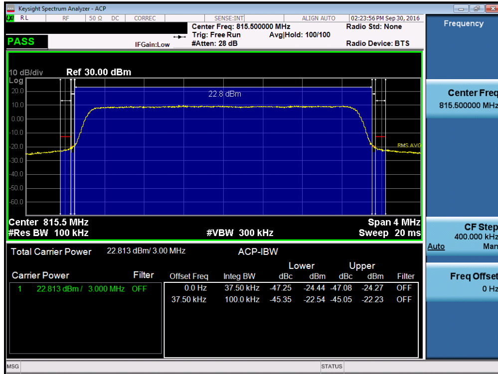
Plot 7-23. Channel Edge Plot (LTE Band 26, 3MHz QPSK – RB Size 15– Low Channel)
