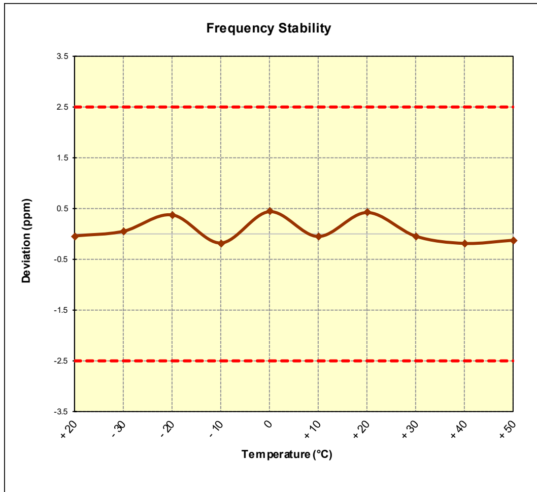
Figure 7-6. CDMA BC10 Frequency Stability Graph (Ch. 476)
