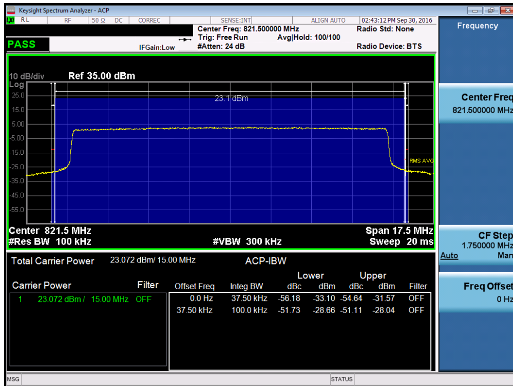
Plot 7-28. Channel Edge Plot (LTE Band 26, 15MHz QPSK – RB Size 75)
