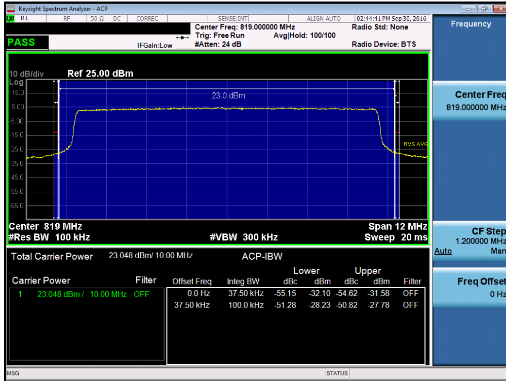
Plot 7-27. Channel Edge Plot (LTE Band 26, 10MHz QPSK – RB Size 50)
