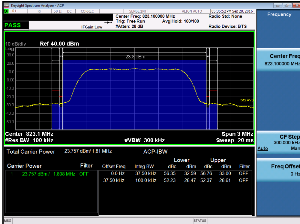
Plot 7-20. Channel Edge Plot (Ch. 684)
