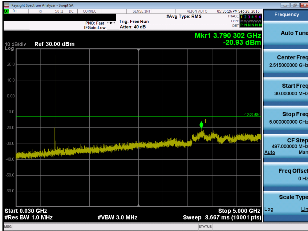
Plot 7-15. Conducted Spurious Plot (CDMA BC10, Ch. 684)
