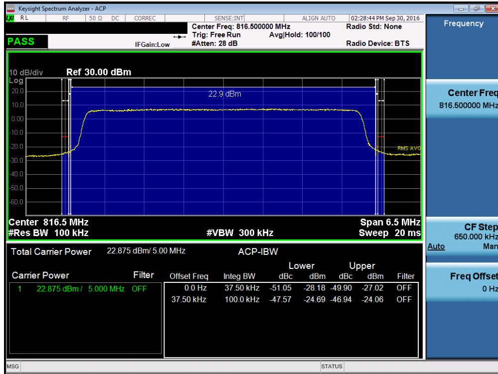
Plot 7-25. Channel Edge Plot (LTE Band 26, 5MHz QPSK – RB Size 25– Low Channel)
