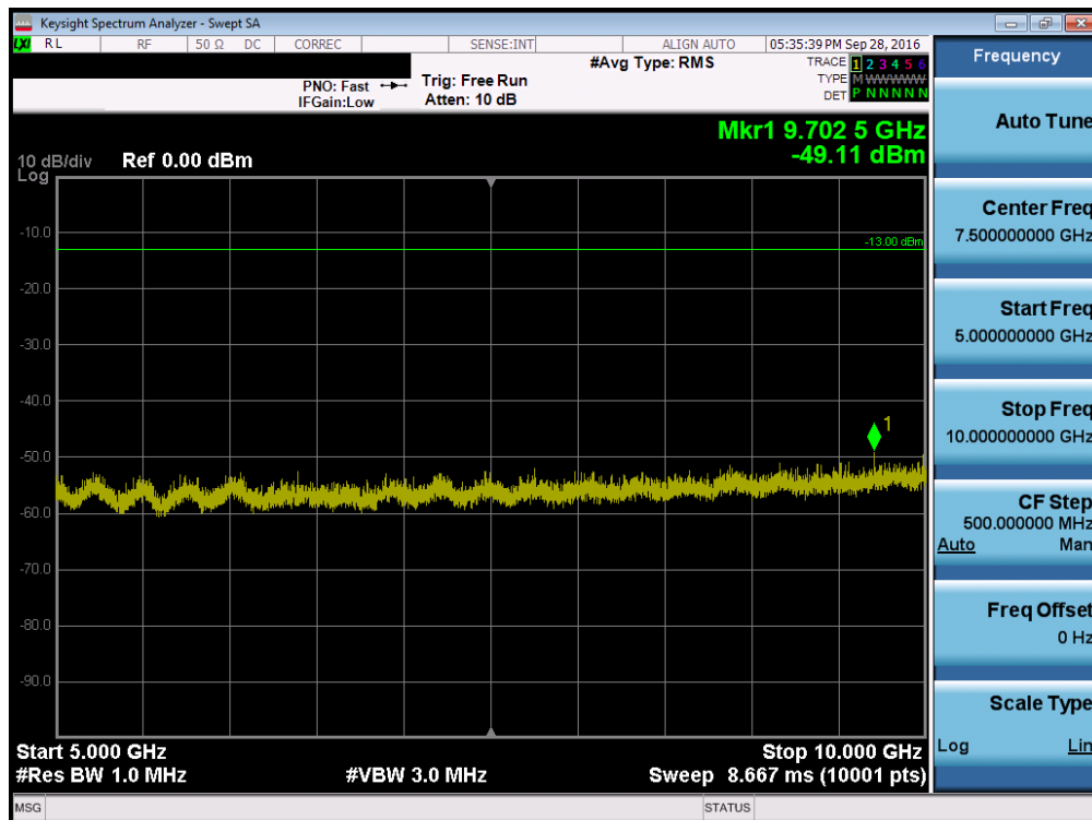
Plot 7-16. Conducted Spurious Plot (CDMA BC10, Ch. 684)
