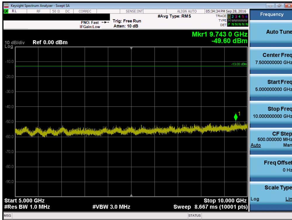
Plot 7-14. Conducted Spurious Plot (CDMA BC10, Ch. 476)
