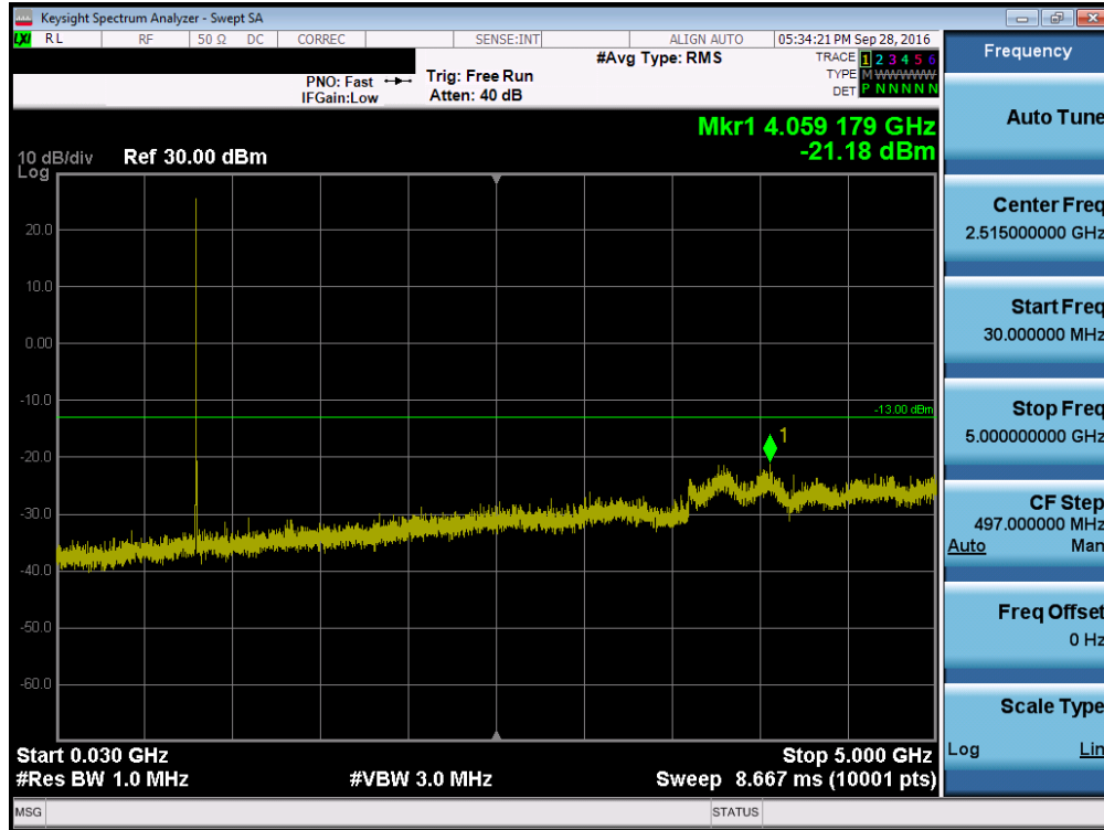
Plot 7-13. Conducted Spurious Plot (CDMA BC10, Ch. 476)
