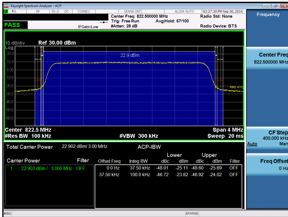
Plot 7-24. Channel Edge Plot (LTE Band 26, 3MHz QPSK – RB Size 15 – High Channel)
