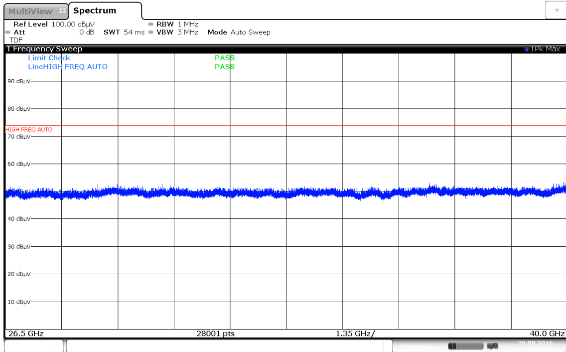
Plot 7-77. Radiated Spurious Plot above 18GHz (802.11a – Ant. Pol. H)
