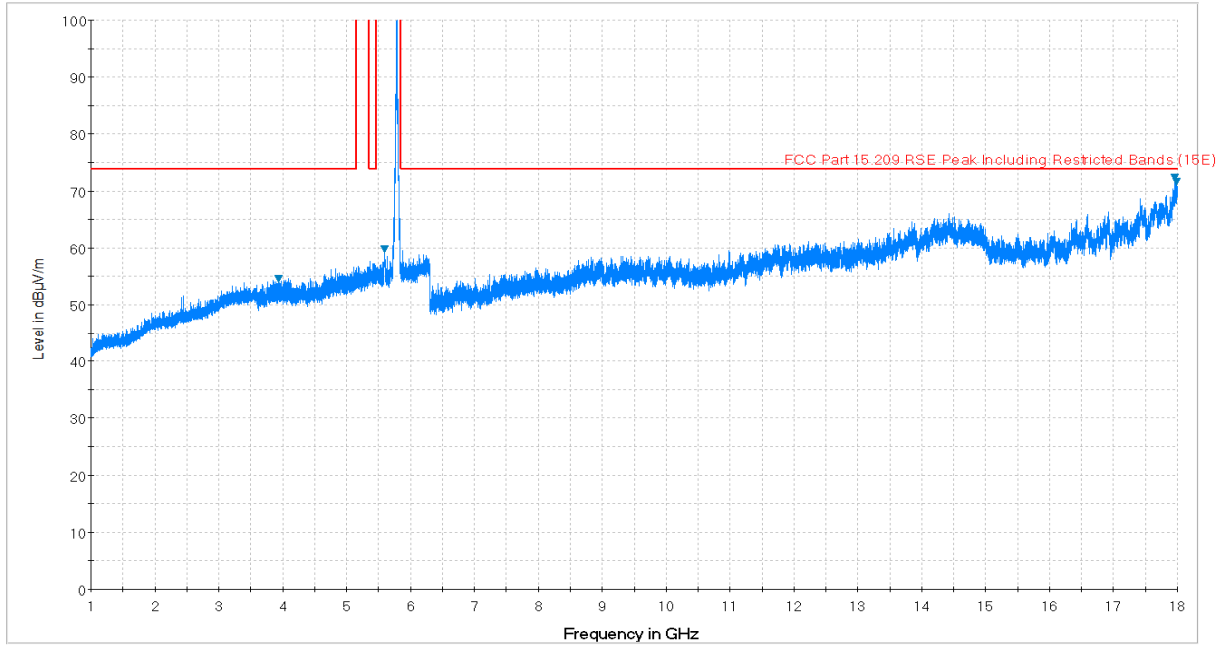
Plot 7-73. Radiated Spurious Plot above 1GHz (802.11a – U3 Ch. 157, Ant. Pol. H)
