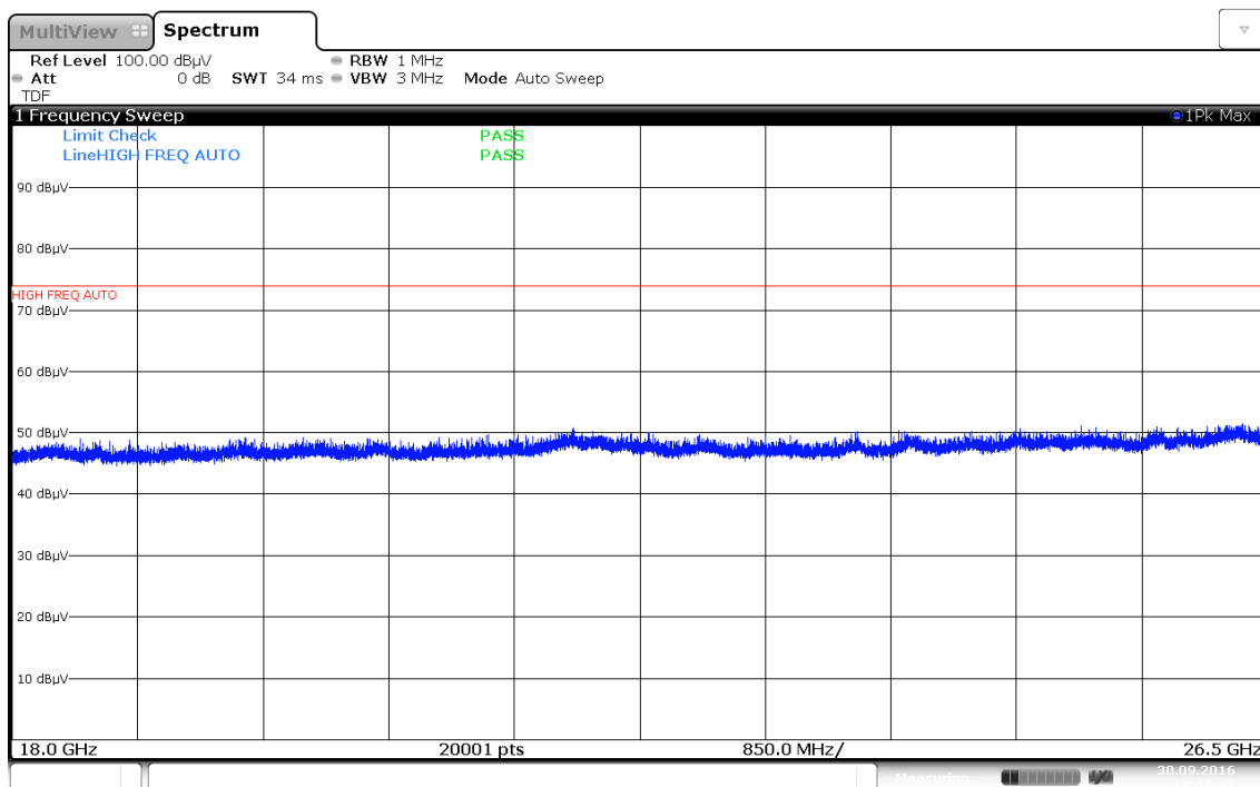
Plot 7-76. Radiated Spurious Plot above 18GHz (802.11a – Ant. Pol. V)
