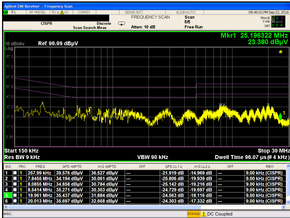
Plot 7-102. Line Conducted Plot with 802.11a UNII Band 3 (N)
