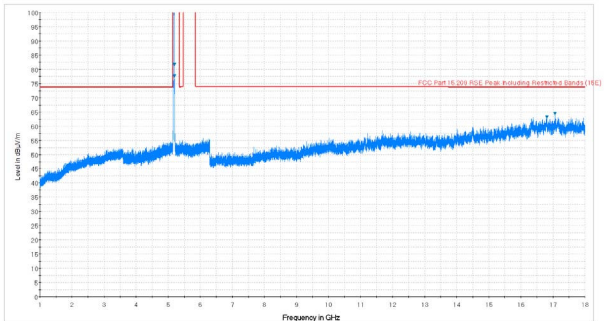
Plot 7-68. Radiated Spurious Plot above 1GHz (802.11a – U1 Ch. 40, Ant. Pol. V)
