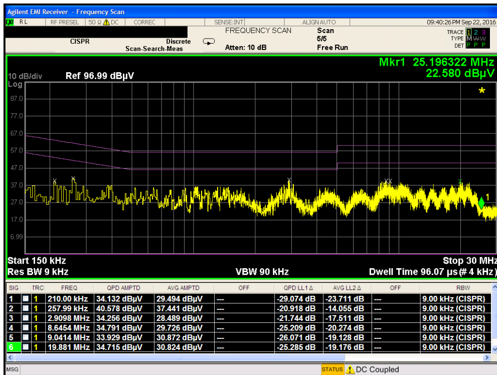
Plot 7-99. Line Conducted Plot with 802.11a UNII Band 2C (L1)
