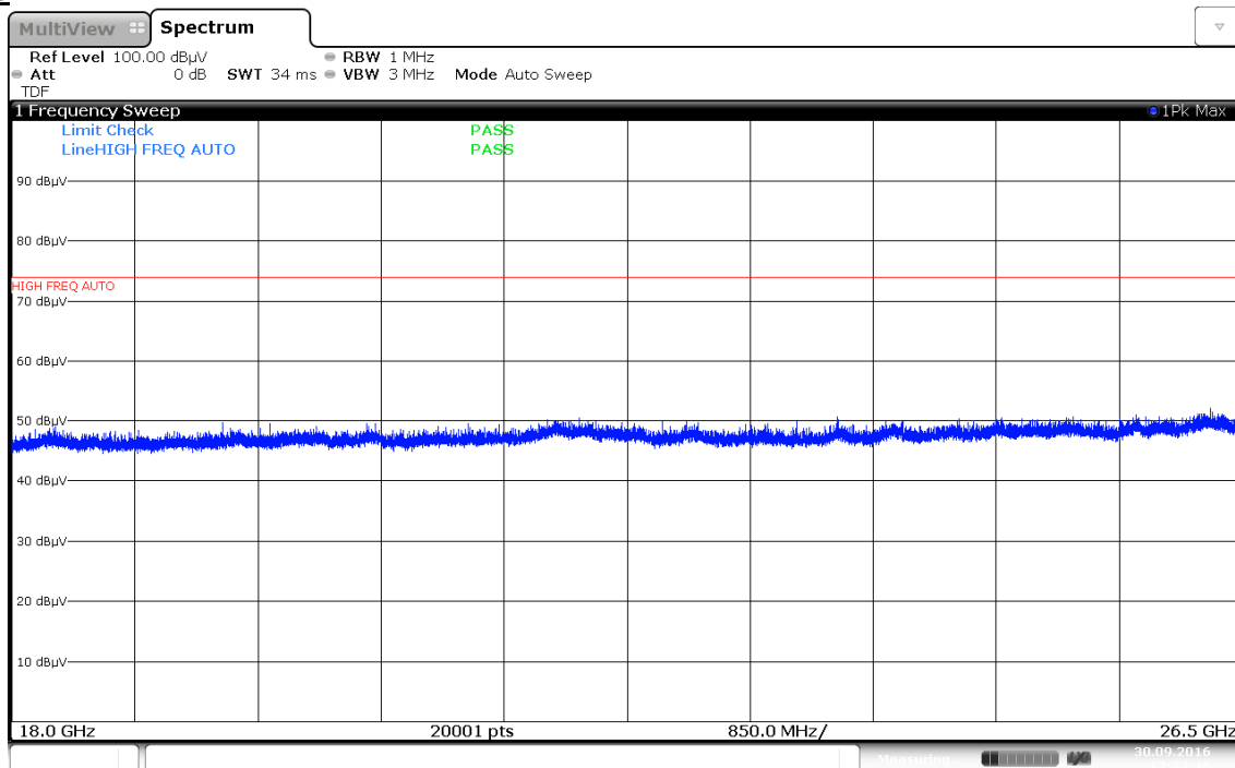
Plot 7-75. Radiated Spurious Plot above 18GHz (802.11a – Ant. Pol. H)
