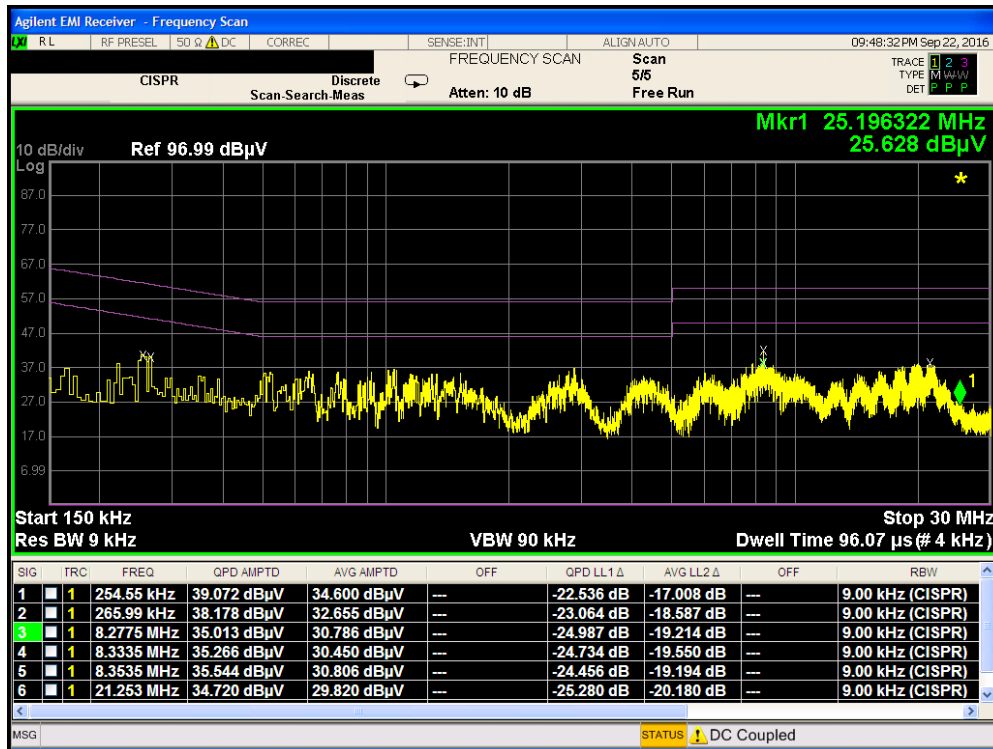
Plot 7-100. Line Conducted Plot with 802.11a UNII Band 2C (N)
