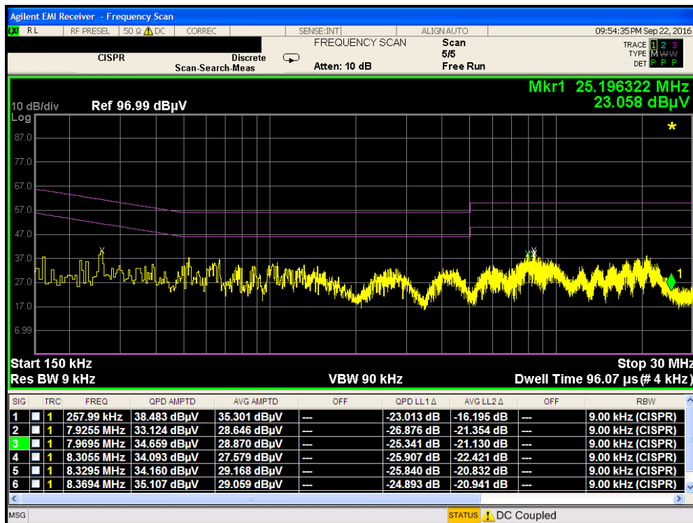
Plot 7-96. Line Conducted Plot with 802.11a UNII Band 1 (N)
