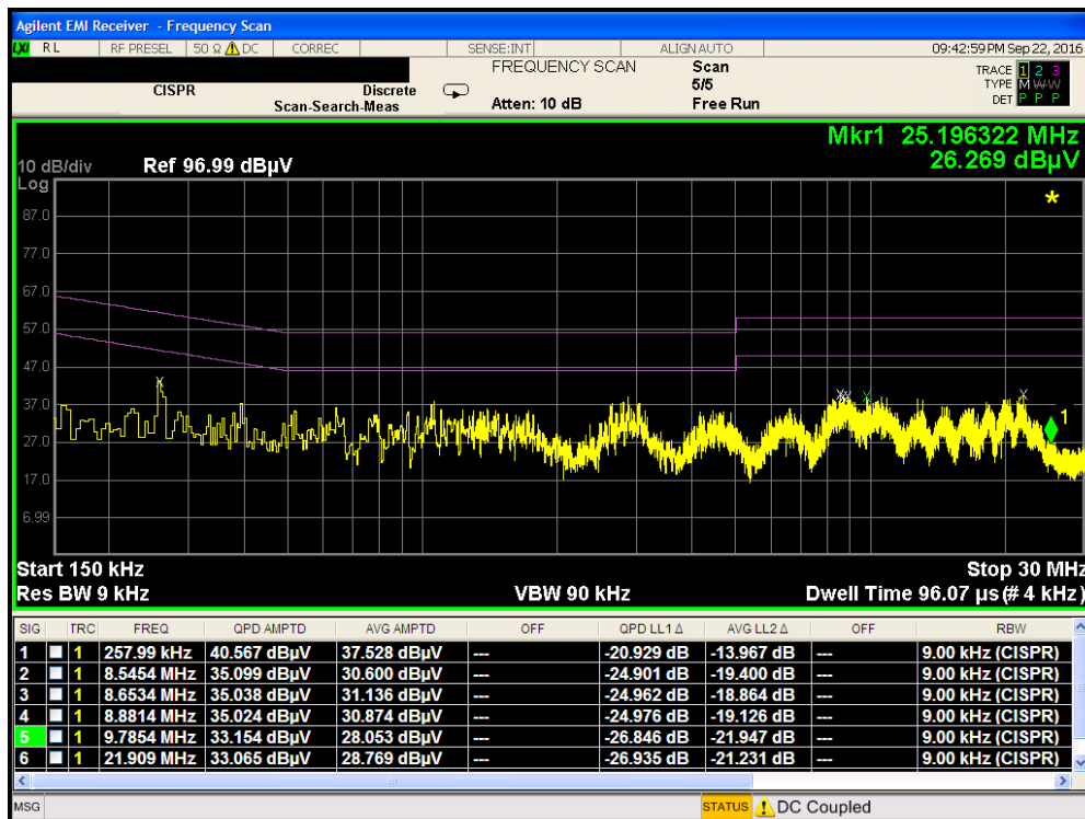
Plot 7-101. Line Conducted Plot with 802.11a UNII Band 3 (L1)
