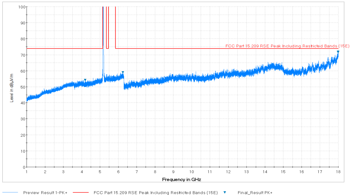
Plot 7-67. Radiated Spurious Plot above 1GHz (802.11a – U1 Ch. 40, Ant. Pol. H)
