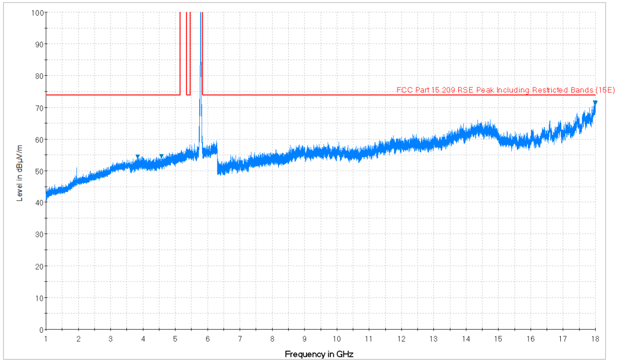
Plot 7-74. Radiated Spurious Plot above 1GHz (802.11a – U3 Ch. 157, Ant. Pol. V)
