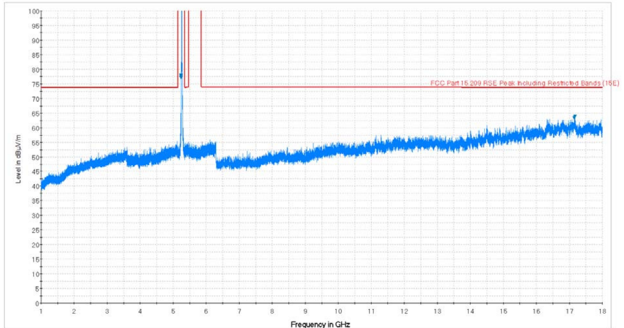
Plot 7-69. Radiated Spurious Plot above 1GHz (802.11a – U2A Ch. 56, Ant. Pol. H)
