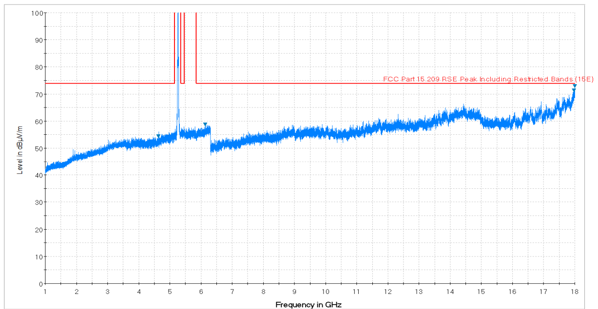
Plot 7-70. Radiated Spurious Plot above 1GHz (802.11a – U2A Ch. 56, Ant. Pol. V)
