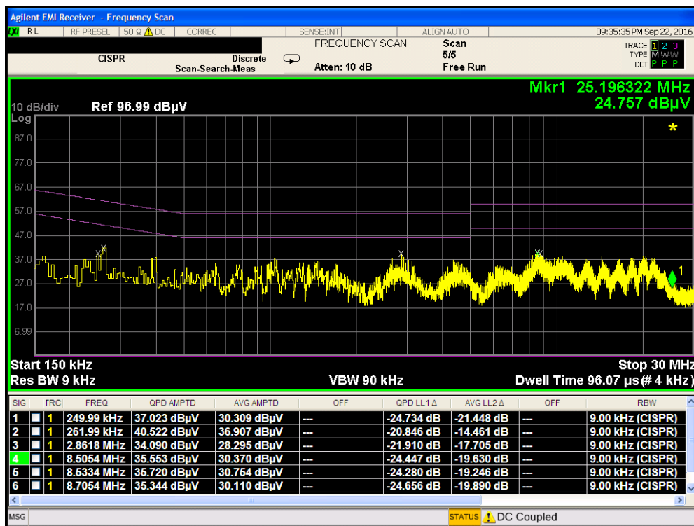
Plot 7-95. Line Conducted Plot with 802.11a UNII Band 1 (L1)
