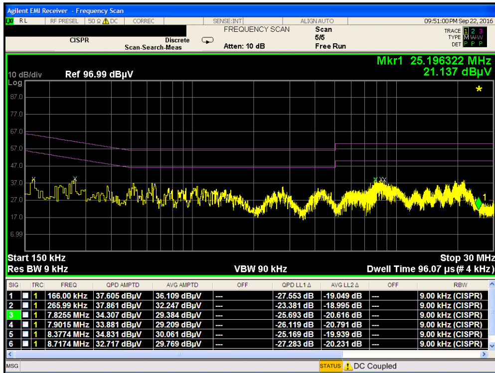
Plot 7-98. Line Conducted Plot with 802.11a UNII Band 2A (N)
