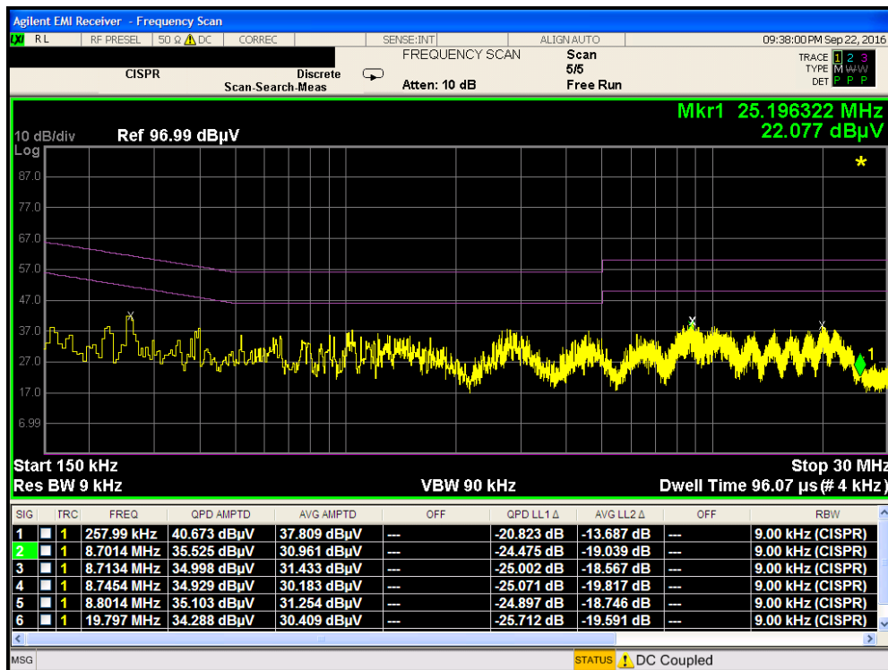
Plot 7-97. Line Conducted Plot with 802.11a UNII Band 2A (L1)
