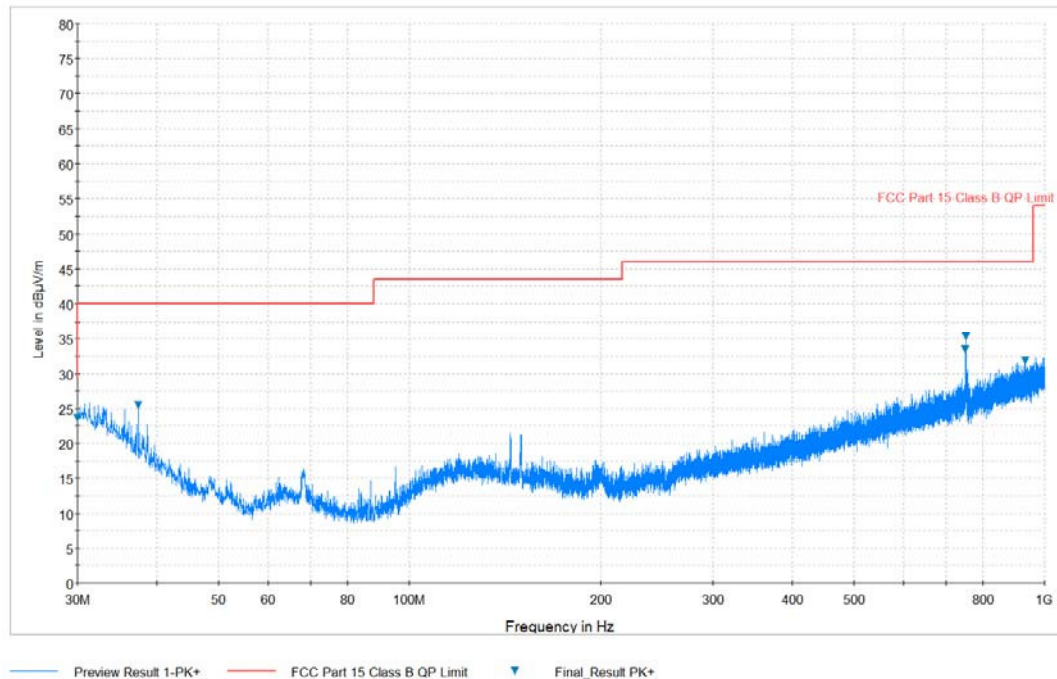
Plot 7-94. Radiated Spurious Plot below 1GHz (802.11a – U3 Ch. 157, Ant. Pol. V)
