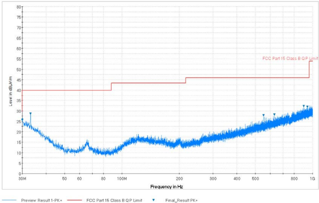
Plot 7-93. Radiated Spurious Plot below 1GHz (802.11a – U3 Ch. 157, Ant. Pol. H)
