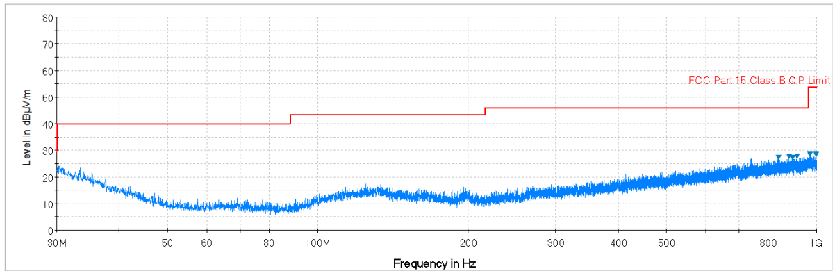
Plot 7-46. Radiated Spurious Plot below 1GHz (Pol. H)
