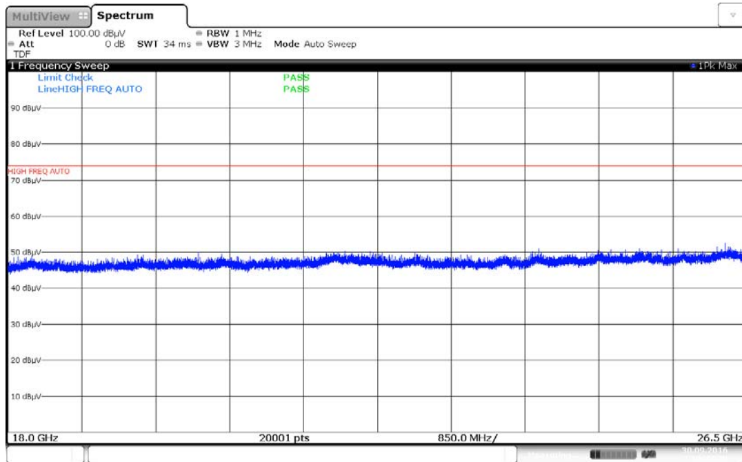
Plot 7-38. Radiated Spurious Plot above 18GHz (Pol. H)
