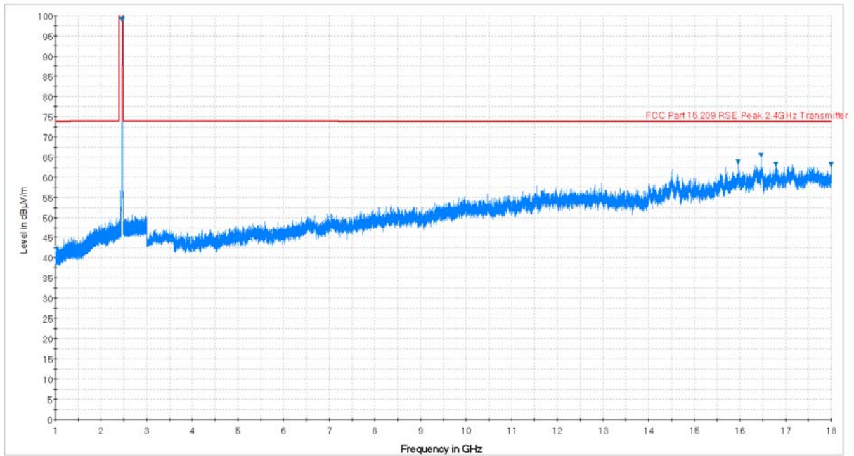
Plot 7-36. Radiated Spurious Plot above 1GHz (802.11b – Ch. 11, Ant. Pol. H)
