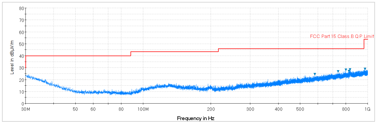
Plot 7-47. Radiated Spurious Plot below 1GHz (Pol. V)
