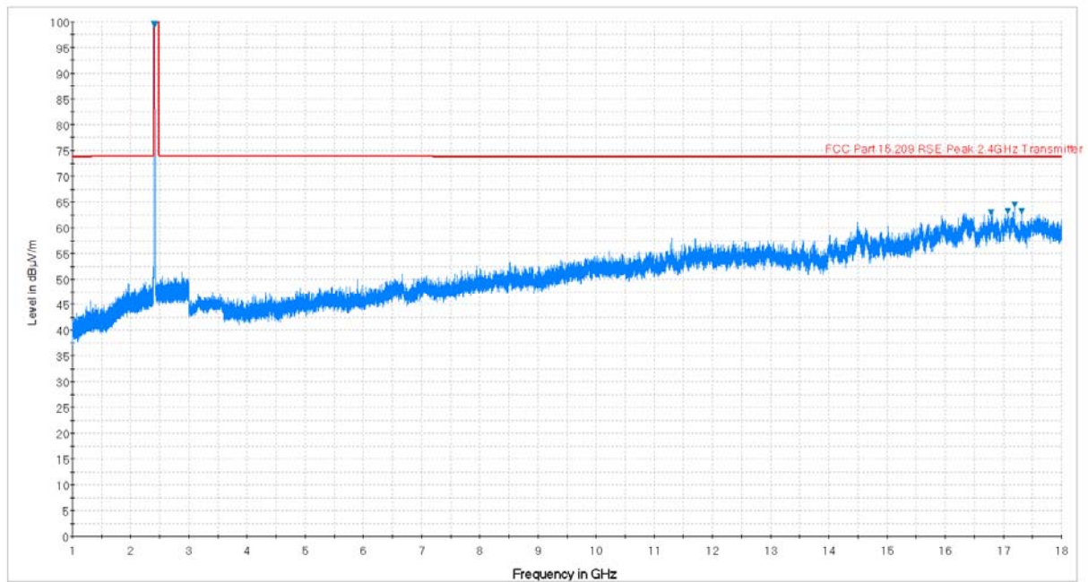
Plot 7-32. Radiated Spurious Plot above 1GHz (802.11b – Ch. 1, Ant. Pol. H)
