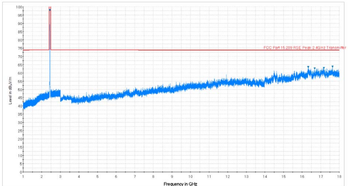
Plot 7-34. Radiated Spurious Plot above 1GHz (802.11b – Ch. 6, Ant. Pol. H)
