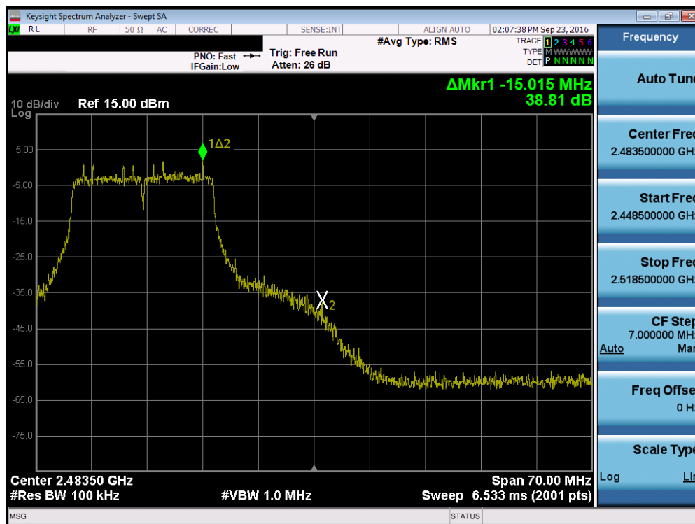
Plot 7-25. Band Edge Plot (802.11n (2.4GHz) – Ch. 11)
