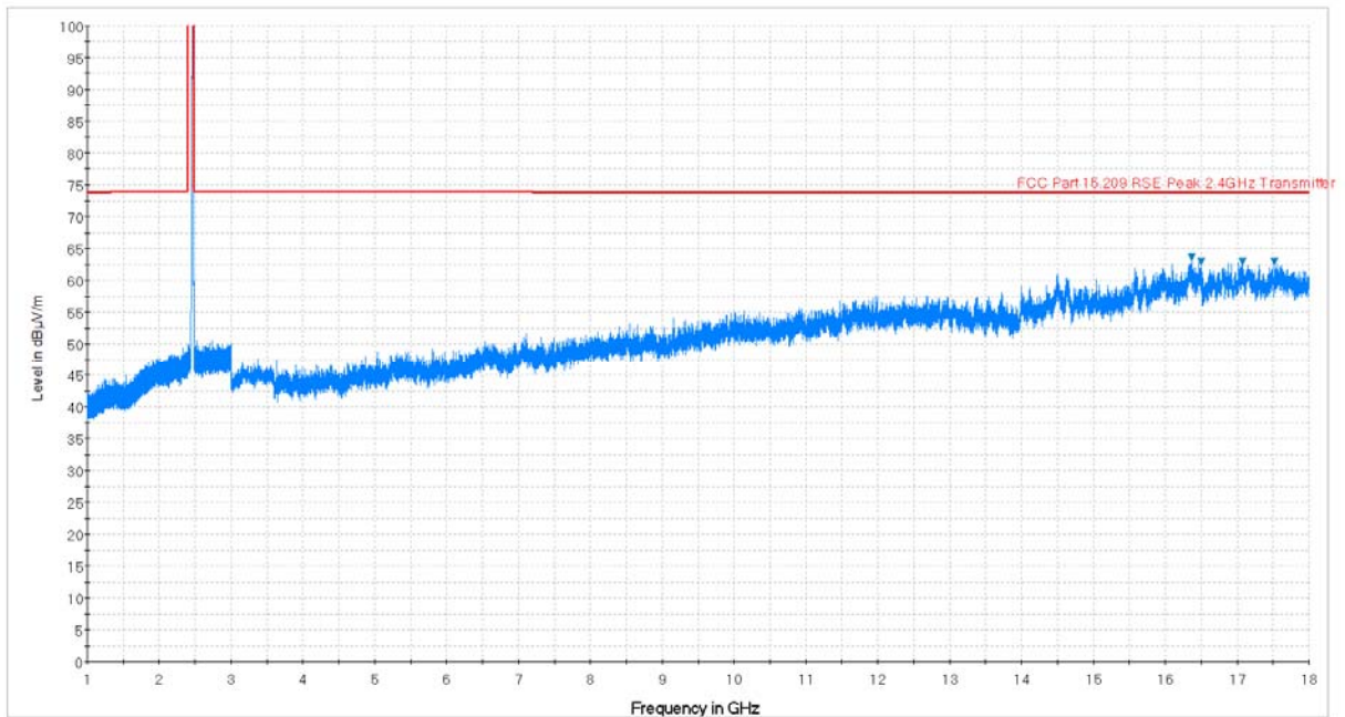
Plot 7-37. Radiated Spurious Plot above 1GHz (802.11b – Ch. 11, Ant. Pol. V)
