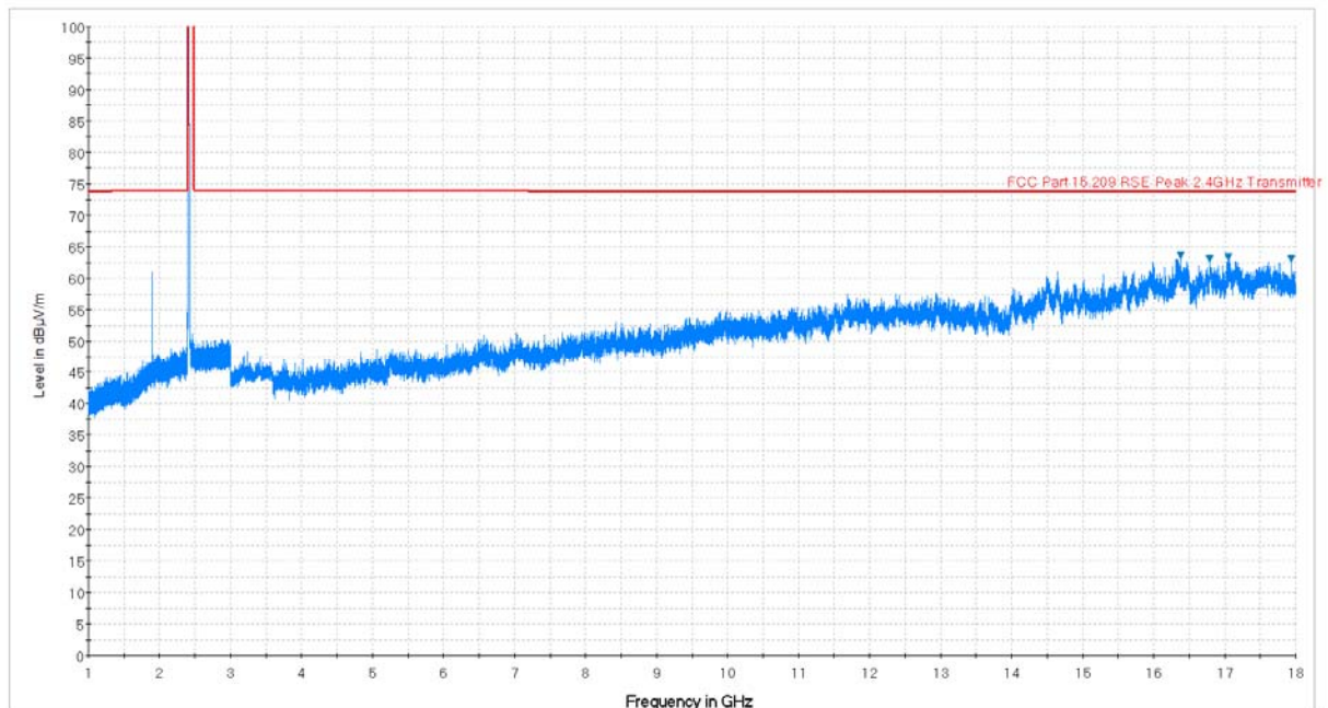
Plot 7-33. Radiated Spurious Plot above 1GHz (802.11b – Ch. 1, Ant. Pol. V)
