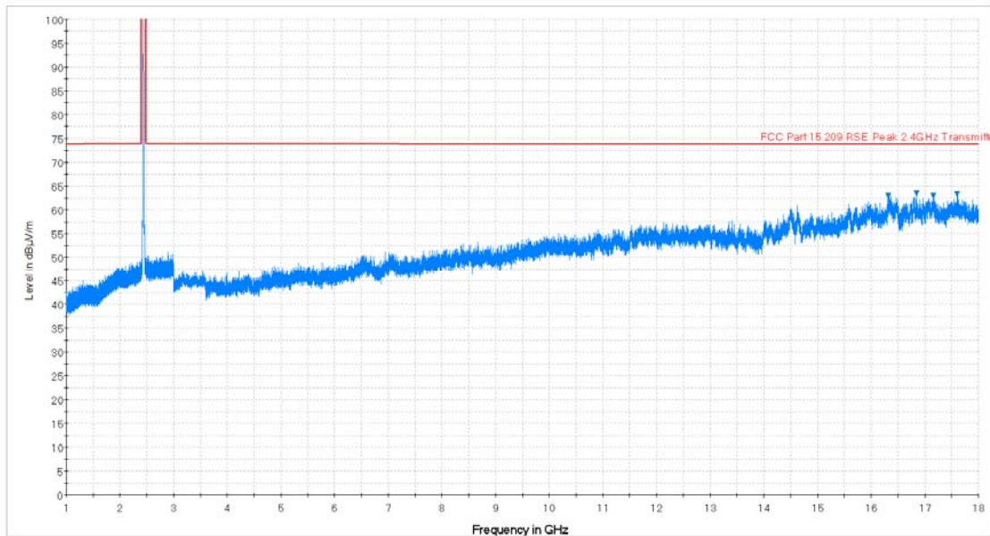
Plot 7-35. Radiated Spurious Plot above 1GHz (802.11b – Ch. 6, Ant. Pol. V)
