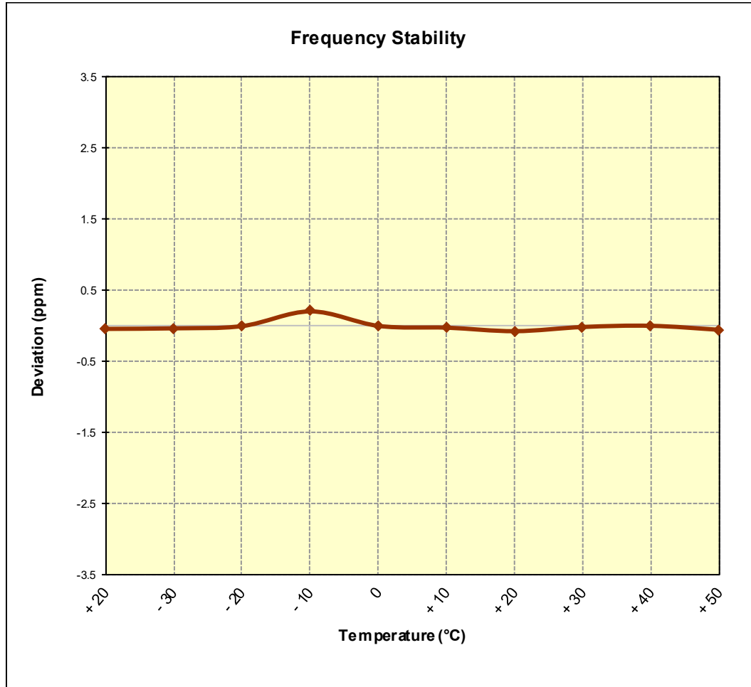
Figure 7-12. Frequency Stability Graph (PCS CDMA Mode – Ch. 600)
