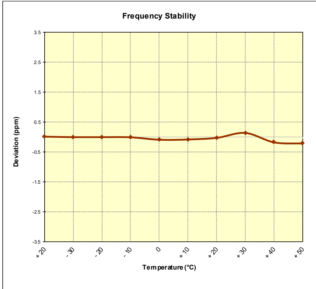
Figure 7-13. Frequency Stability Graph (PCS WCDMA Mode – Ch. 9400)
