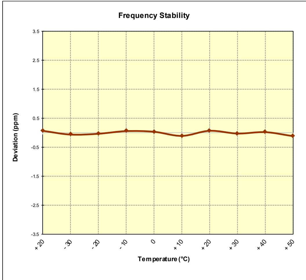
Figure 7-11. Frequency Stability Graph (PCS GPRS Mode – Ch. 661)
