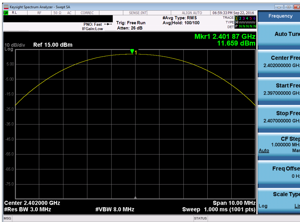
Plot 7-10. Peak Conducted Power (1Mbps – Ch. 0)
