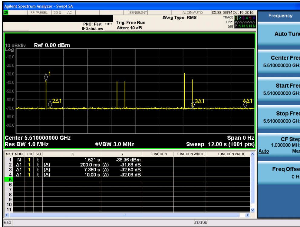
Figure 5-6. Band 2C Move Time and Aggregate Time
