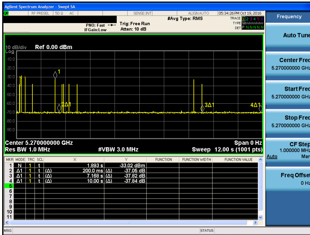
Figure 5-5. Band 2A Move Time and Aggregate Time
