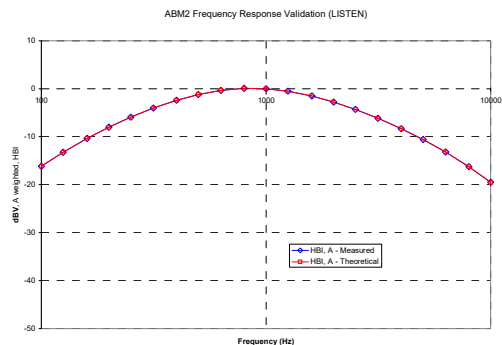
Figure 4-7 ABM2 Frequency Response Validation
