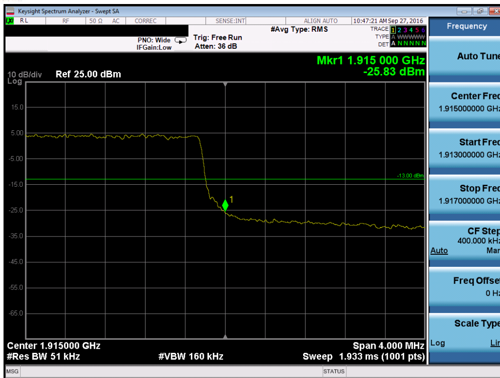
Plot 7-139. Upper Band Edge Plot (Band 2/25 – 5.0MHz QPSK – RB Size 25)
