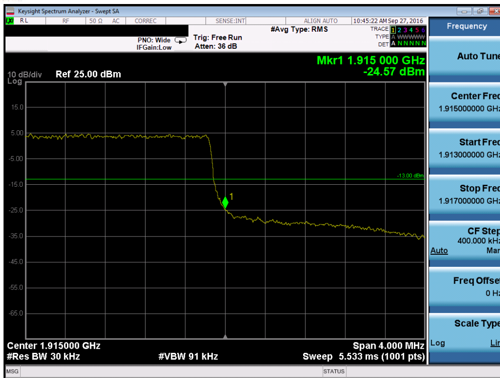
Plot 7-135. Upper Band Edge Plot (Band 2/25 – 3.0MHz QPSK – RB Size 15)
