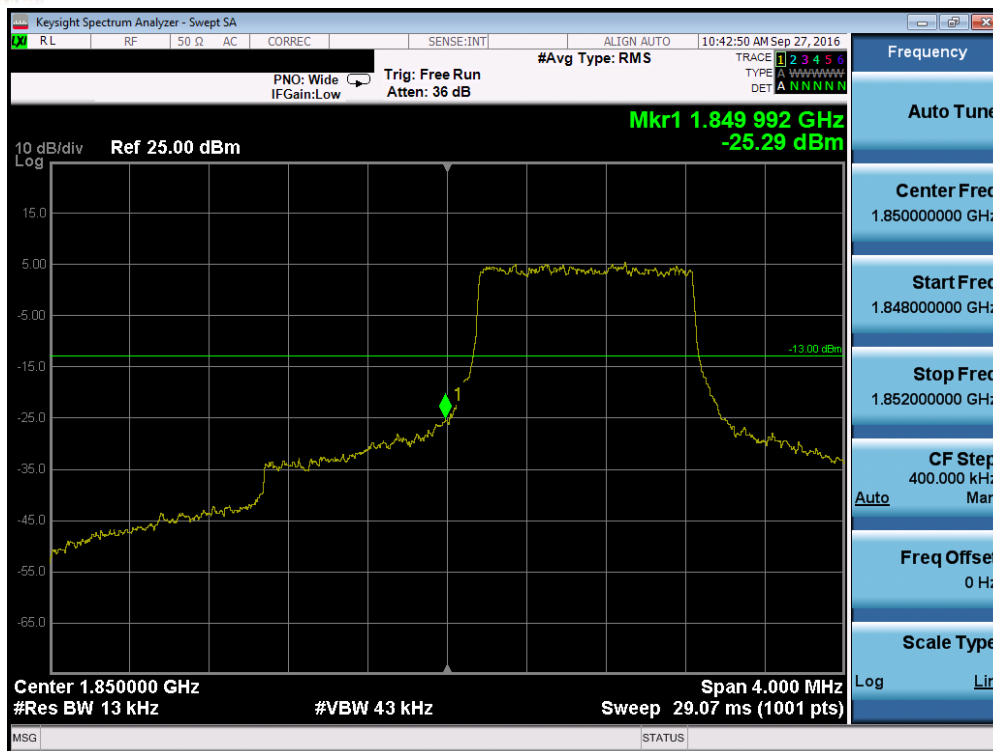
Plot 7-129. Lower Band Edge Plot (Band 2/25 – 1.4MHz QPSK – RB Size 6)
