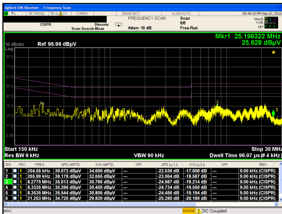
Plot 7-100. Line Conducted Plot with 802.11a UNII Band 2C (N)
