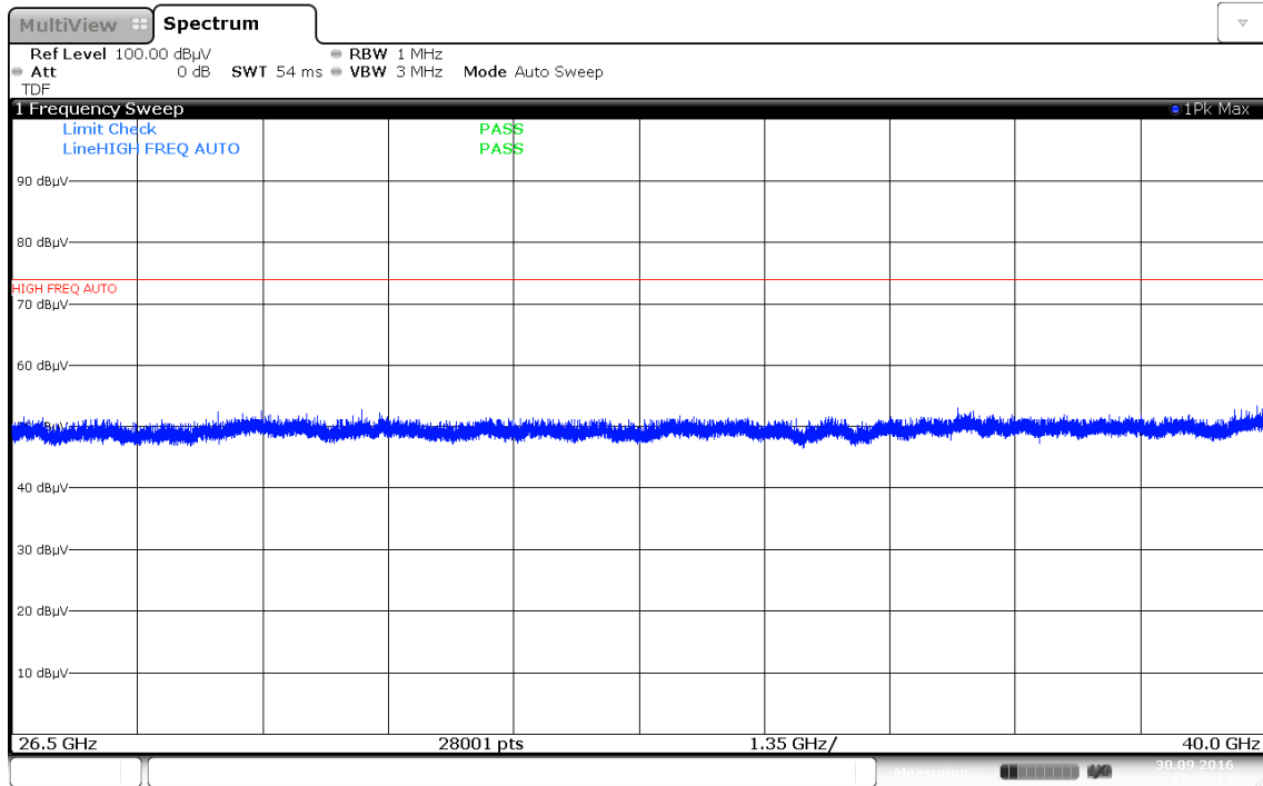
Plot 7-77. Radiated Spurious Plot above 18GHz (802.11a – Ant. Pol. H)
