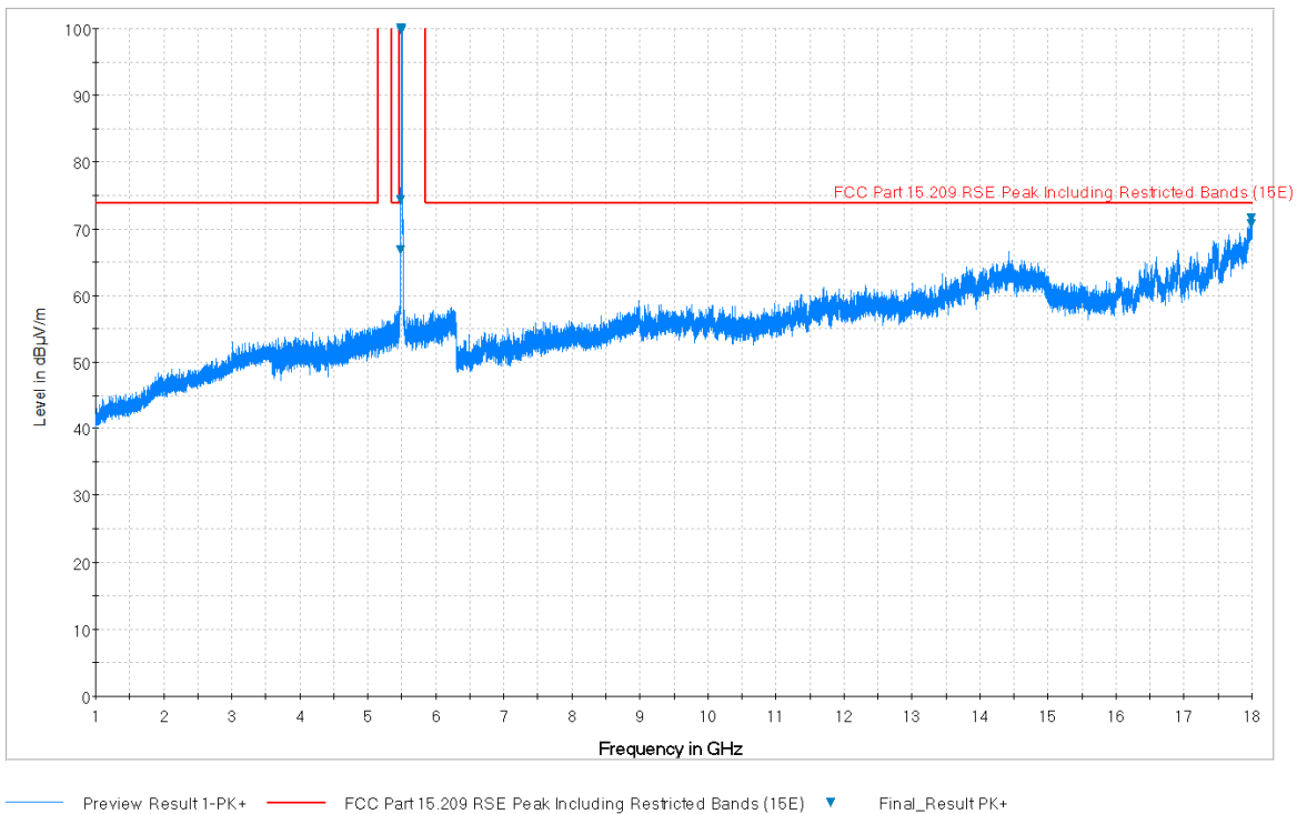
Plot 7-72. Radiated Spurious Plot above 1GHz (802.11a – U2C Ch. 120, Ant. Pol. V)
