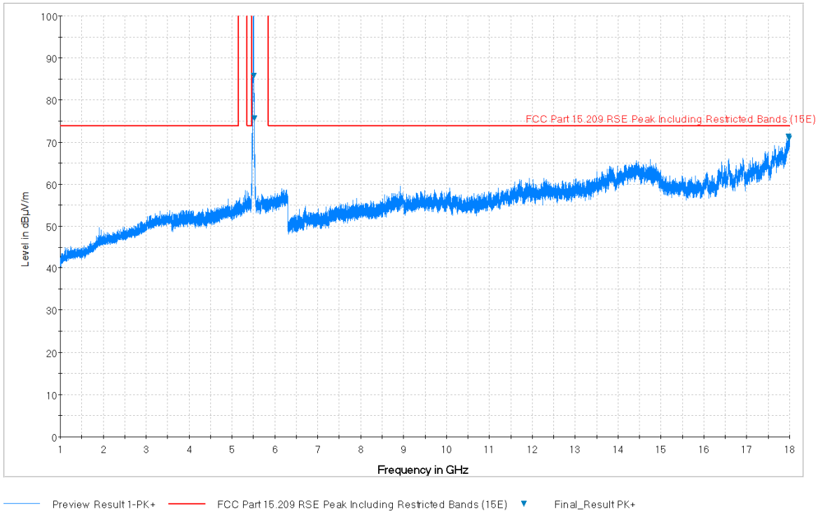
Plot 7-71. Radiated Spurious Plot above 1GHz (802.11a – U2C Ch. 120, Ant. Pol. H)
