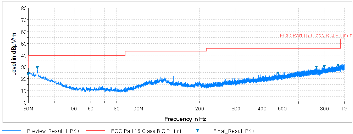
Plot 7-93. Radiated Spurious Plot below 1GHz (802.11a – U3 Ch. 157, Ant. Pol. H)
