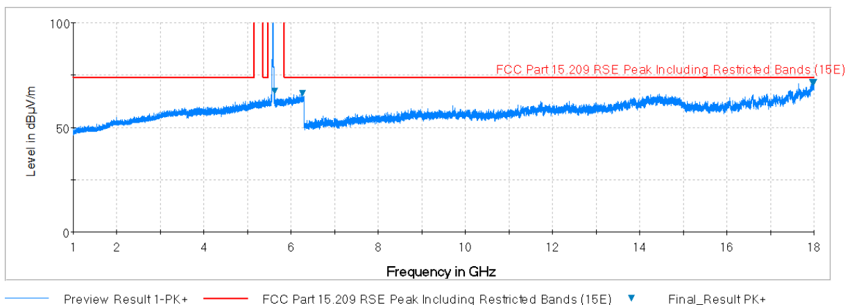
Plot 7-72. Radiated Spurious Plot above 1GHz (802.11a – U2C Ch. 116, Ant. Pol. V)
