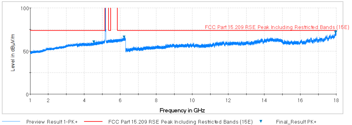
Plot 7-67. Radiated Spurious Plot above 1GHz (802.11a – U1 Ch. 40, Ant. Pol. H)
