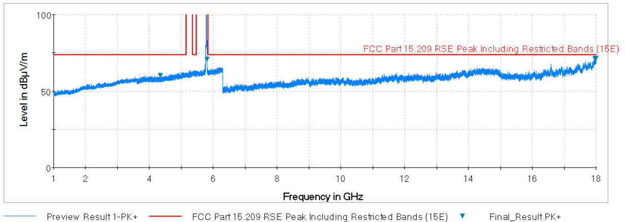
Plot 7-74. Radiated Spurious Plot above 1GHz (802.11a – U3 Ch. 157, Ant. Pol. V)
