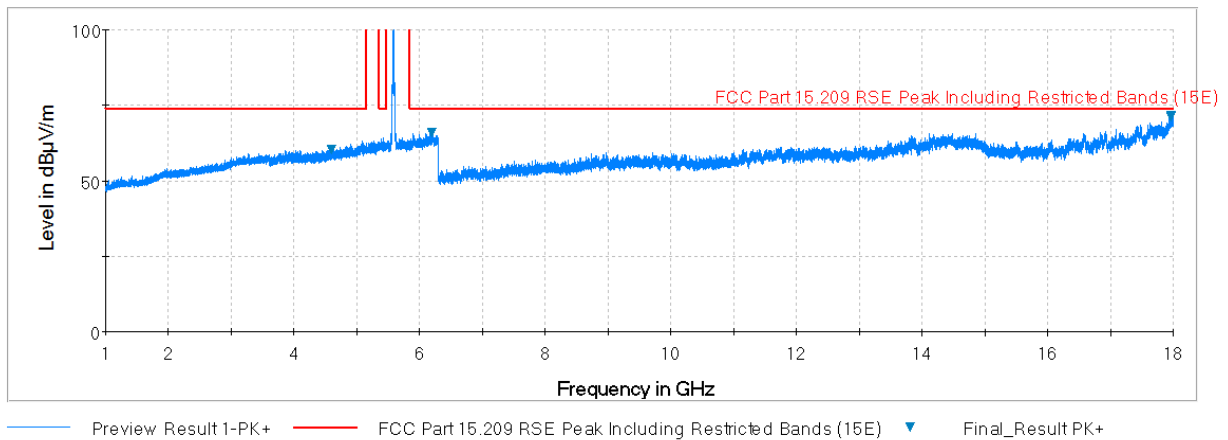
Plot 7-71. Radiated Spurious Plot above 1GHz (802.11a – U2C Ch. 116, Ant. Pol. H)
