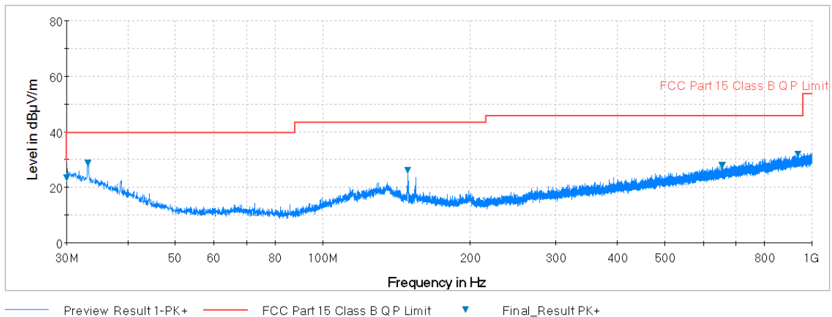
Plot 7-94. Radiated Spurious Plot below 1GHz (802.11a – U3 Ch. 157, Ant. Pol. V)
