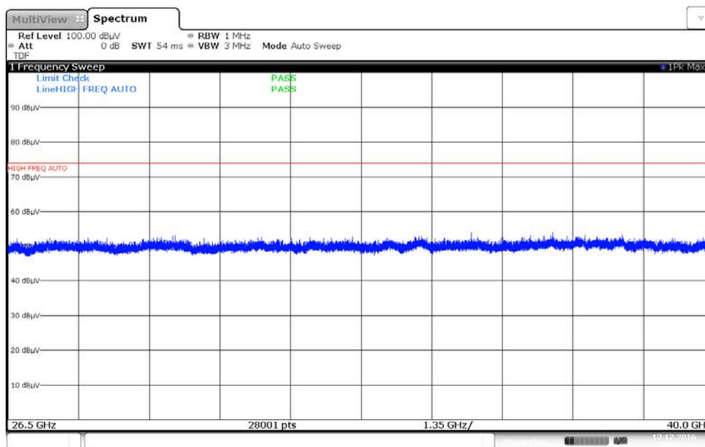
Plot 7-78. Radiated Spurious Plot above 26.5GHz (802.11a – Ant. Pol. V)
