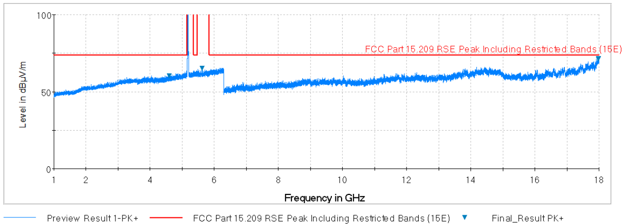
Plot 7-68. Radiated Spurious Plot above 1GHz (802.11a – U1 Ch. 40, Ant. Pol. V)
