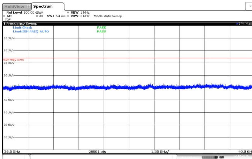
Plot 7-77. Radiated Spurious Plot above 26.5GHz (802.11a – Ant. Pol. H)
