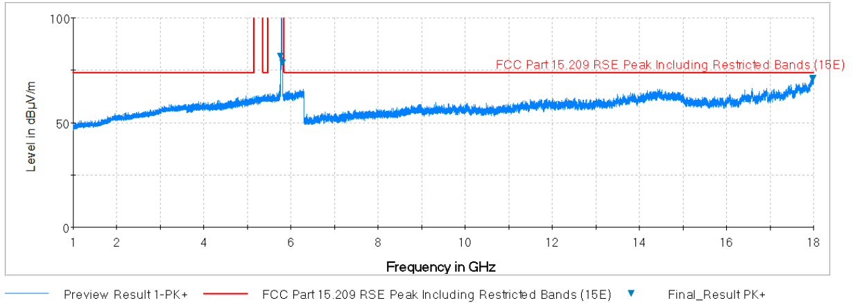
Plot 7-73. Radiated Spurious Plot above 1GHz (802.11a – U3 Ch. 157, Ant. Pol. H)
