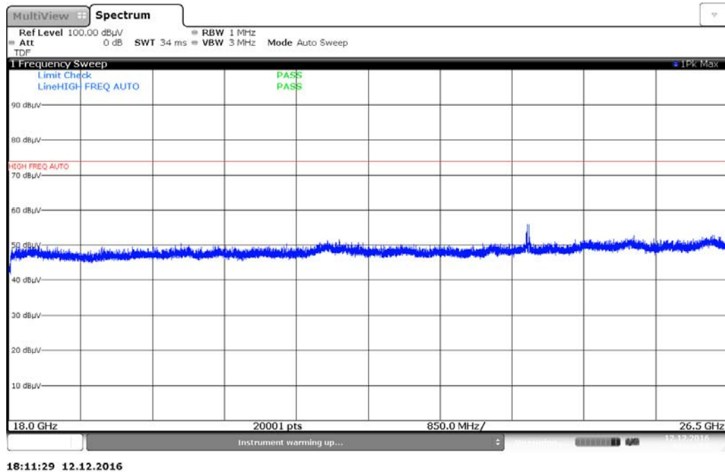
Plot 7-40. Radiated Spurious Plot above 18GHz (Pol. V)
