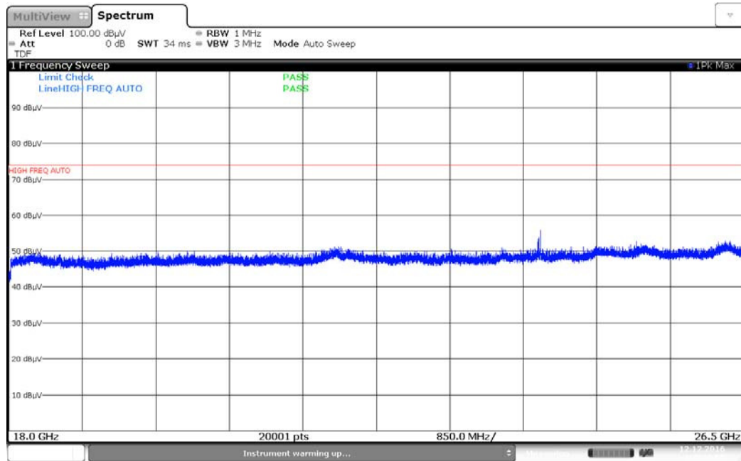
Plot 7-39. Radiated Spurious Plot above 18GHz (Pol. H)
